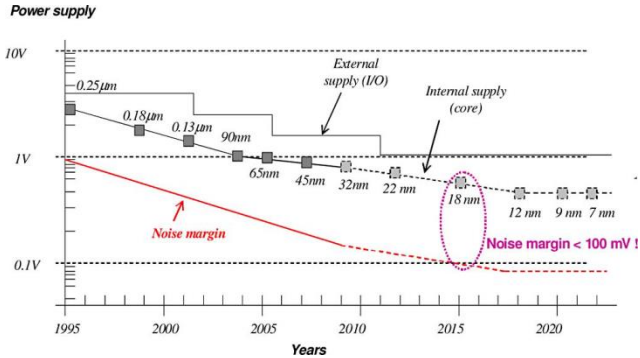
Figure II-20 Reduction of internal supply voltage leads to a reduced noise margin [RAMD09]
