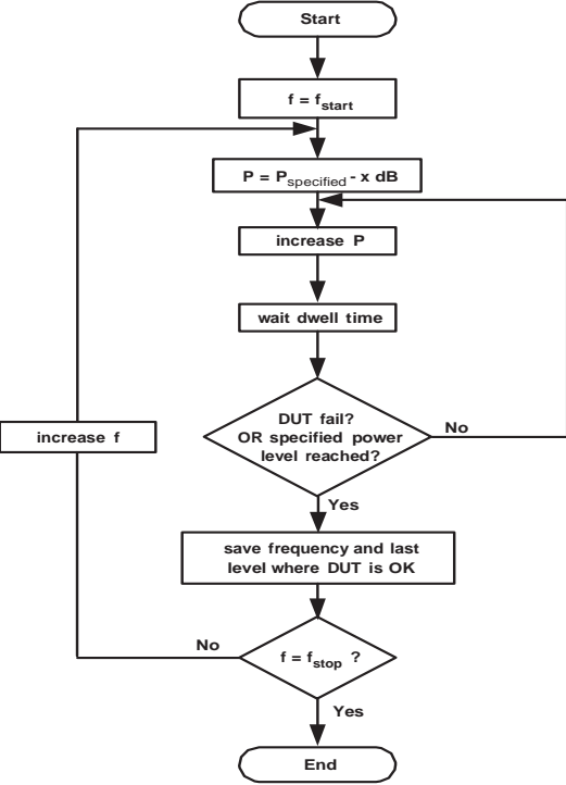
Figure IV-7 Flowchart of the test procedure for Direct Power Injection [IEC 62132-4]
