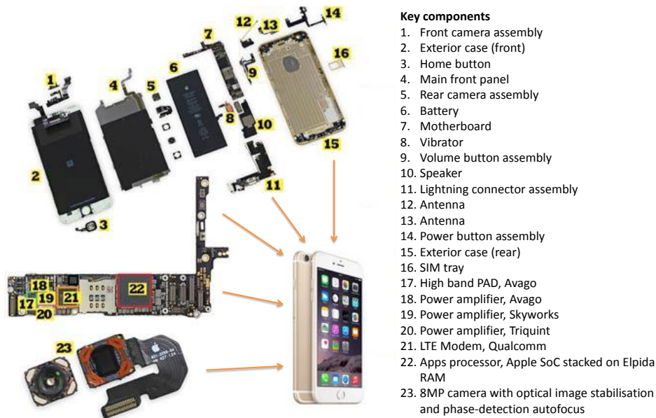
Figure II-7 Teardown analysis of an iPhone 6 Plus [DEMP14]
