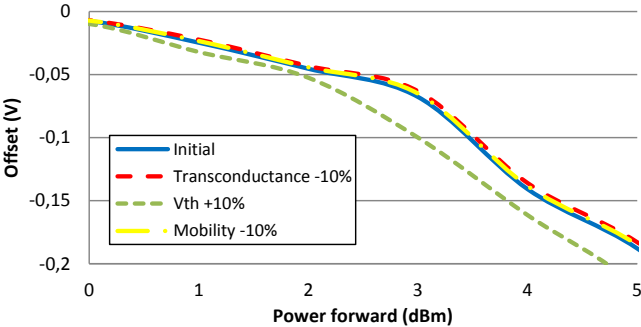
Figure IV-56 Simulation test of offset drift with the variation of different MOSFET parameters
