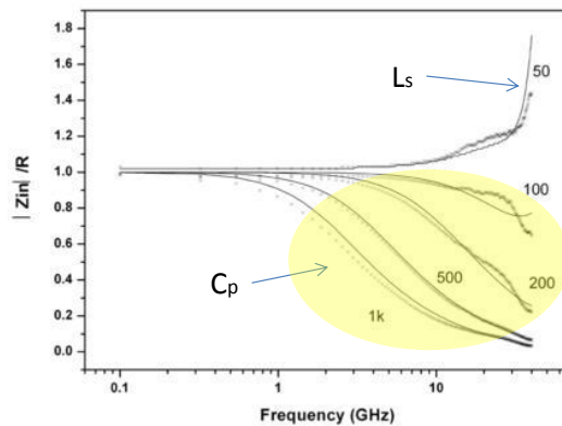
Figure III-38 Impedance measurement (dotted line) and modeling (solid line) of thin film chip resistors of different value [VISH06]
