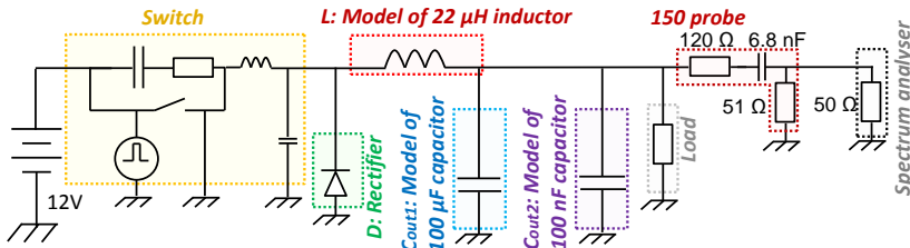
Figure IV-76 Output conducted emission modeling of the DC-DC buck converter
