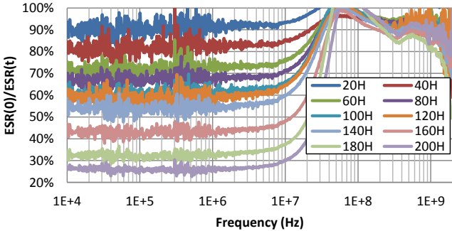
Figure III-55 ESR(0)/ESR(t) with aging time t of C1_1 aluminum electrolytic capacitor 100 μF
