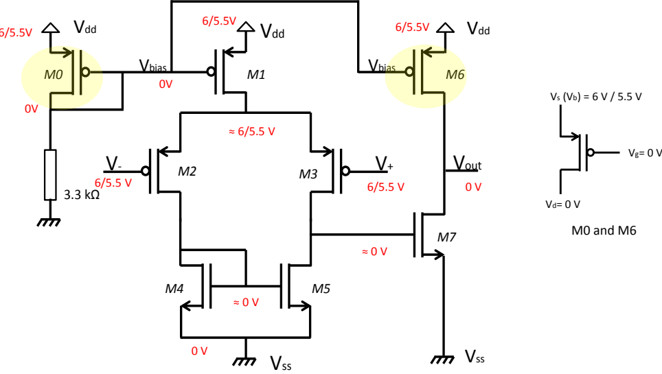
Figure IV-38 Voltage stress on each transistor of the amplifier
