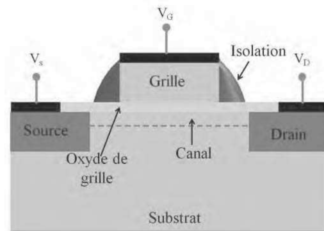
Figure 0.2 – Structure MOSFET.
