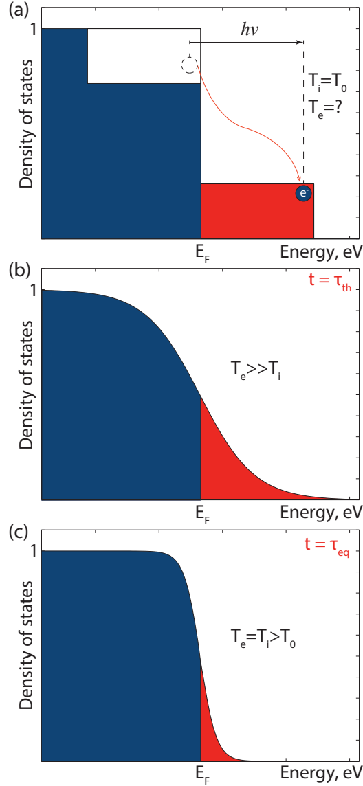
Figure 1.2: Consequent dynamics of the distribution of electrons induced by a femtosecond laser pulse; a) quasi-instantaneous repopulation of the states above the Fermi level E_F induced by absorption of the laser pulse with energy h\nu . Formed distribution is non-Fermi like because of the high level of non-equilibrium, as a result system can not be characterized by an electron temperature T_e . b) After electron thermalization (by the time t = \tau_{th} ) the electron distribution can be described by the Fermi-Dirac statistics, thus electrons can be characterized by some value of T_e that is typically greater than the lattice temperature T_i . c) Through electron-phonon interaction the energy of electrons is redistributed to the lattice and the system reaches equilibrium ( T_e = T_i ) by the time \tau_{eq} .
