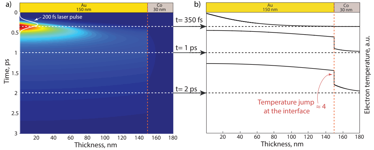
Figure 3.22: a) Distribution of the electron temperature after absorption of 200 fs laser pulse inside of gold/-cobalt layers with the Kapitza resistance. b) Spatial profiles of T_e at t = 0.35 ps, 1 ps and 2 ps demonstrate a temperature drop at the gold/cobalt interface by a factor of 4, which is caused by presence of the Kapitza resistance.
