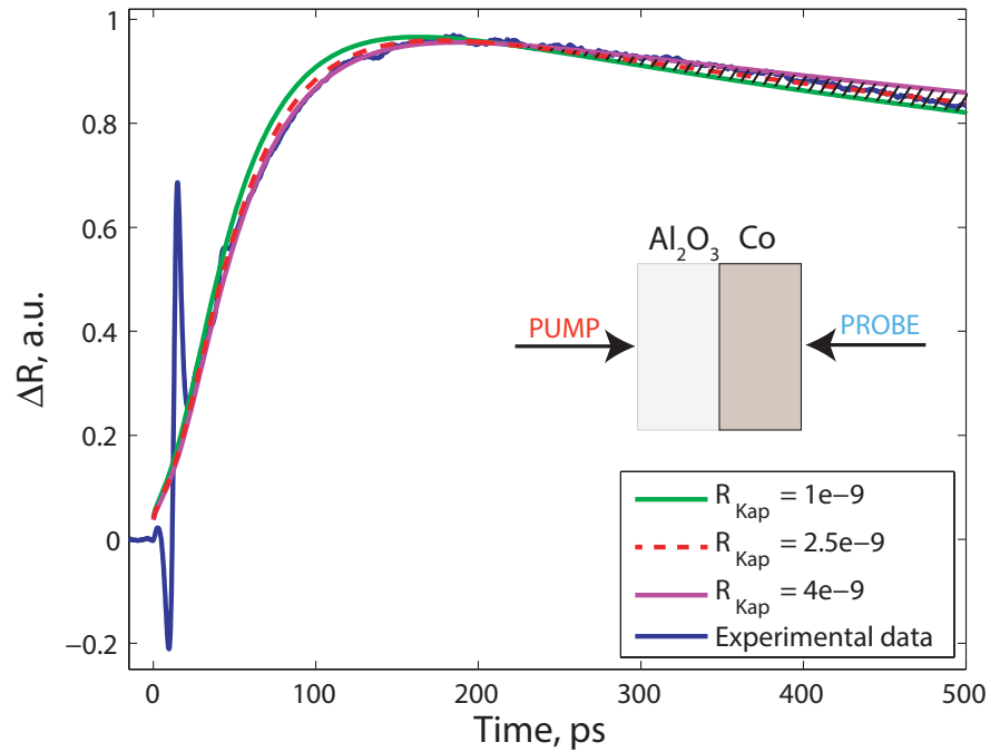
Figure 3.9: Reflectivity curve (blue solid line) of the cobalt/sapphire sample is fitted with the solution of the heat diffusion equation (red dashed line) that corresponds to the Kapitza resistance R_{Kap} = 2.5 \cdot 10^{-9} \text{ m}^2 \text{KW}^{-1} with an error \pm 1.5 \cdot 10^{-9} \text{ m}^2 \text{KW}^{-1} .
