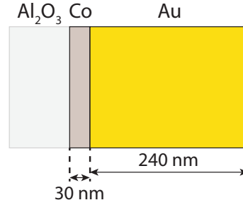
Figure 3.14: Thin 30 nm cobalt layer is sandwiched between 240 nm gold layer and sapphire substrate.
