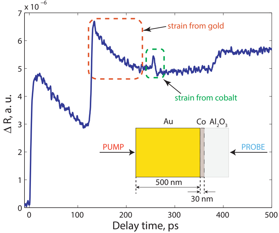
Figure 3.1: Demonstration of the strain generation in cobalt layer through 500 nm of gold
