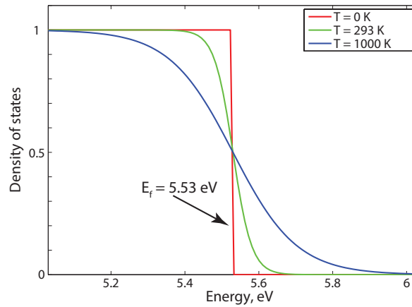
Figure B.13: Example of the Fermi-Dirac distribution for gold for three temperatures T = 0 \text{ K} , 293 \text{ K} and 1000 \text{ K} showing the migration of the electrons towards higher energy states when the temperature of metal is increased.
