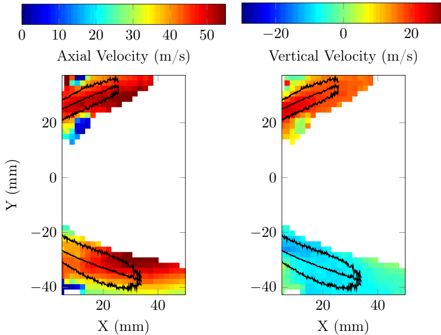
Figure 7.4 – Mean axial (left) and vertical (right) spray velocities from the PIV treatment of the tulip Mie scattering fields. A threshold has been set at 2% of vector validation. The black lines represent the spray limits from the Mie scattering RMS image (Fig.7.3).
