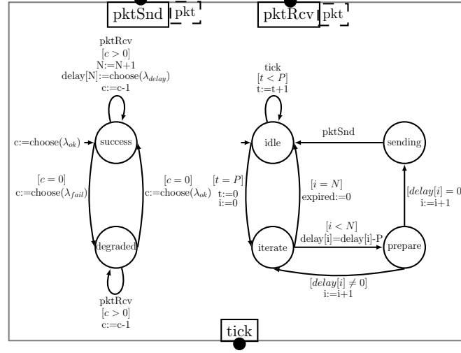
Figure 7.7: AbsWLANModel component
