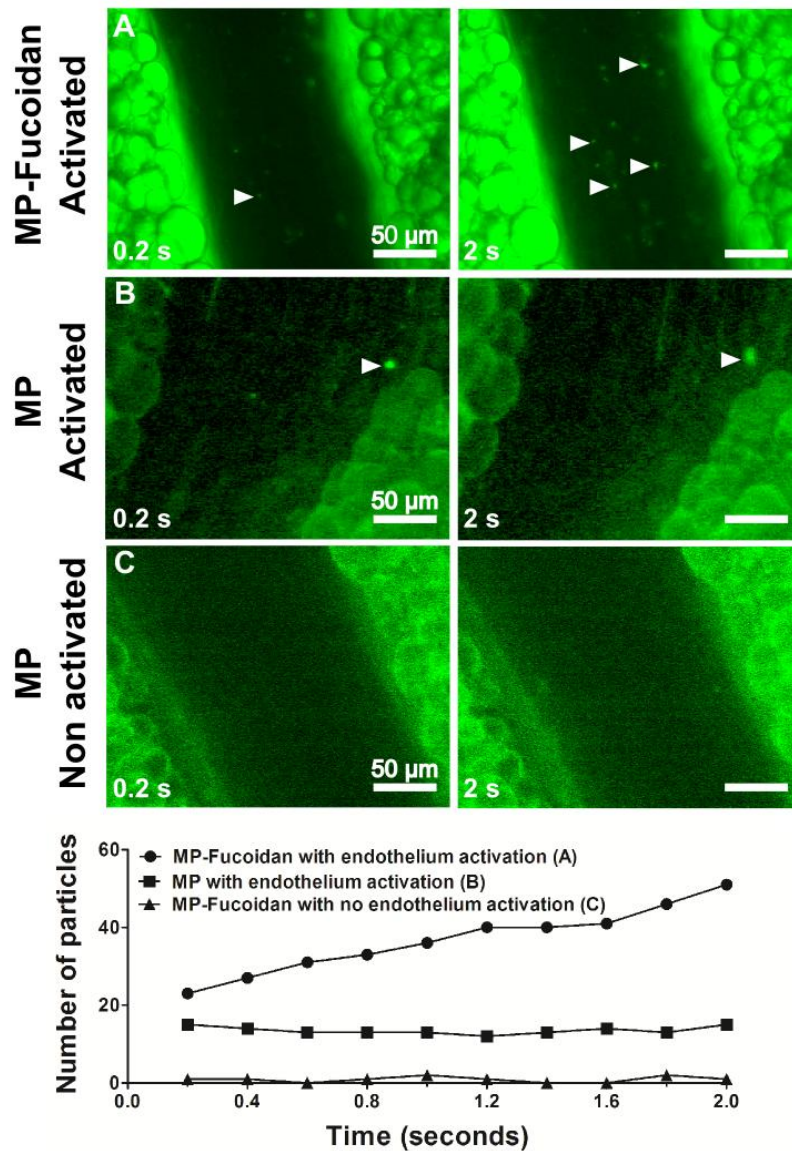
Figure 2. Intravital microscopy dynamic observation in calcium ionophore activated mesenteric venules after intravenous injection (200 \mu L) of MP-Fucoidan (A) and MP (B). Control after injection of MP-Fucoidan with no activation was assessed (C). Snapshot series start before 5 seconds after injections and are separated by 0.2 s. Number of microparticles in function of time after injection were plotted. Scale bar: 50 \mu m. Arrow heads indicate adherent microparticles.
