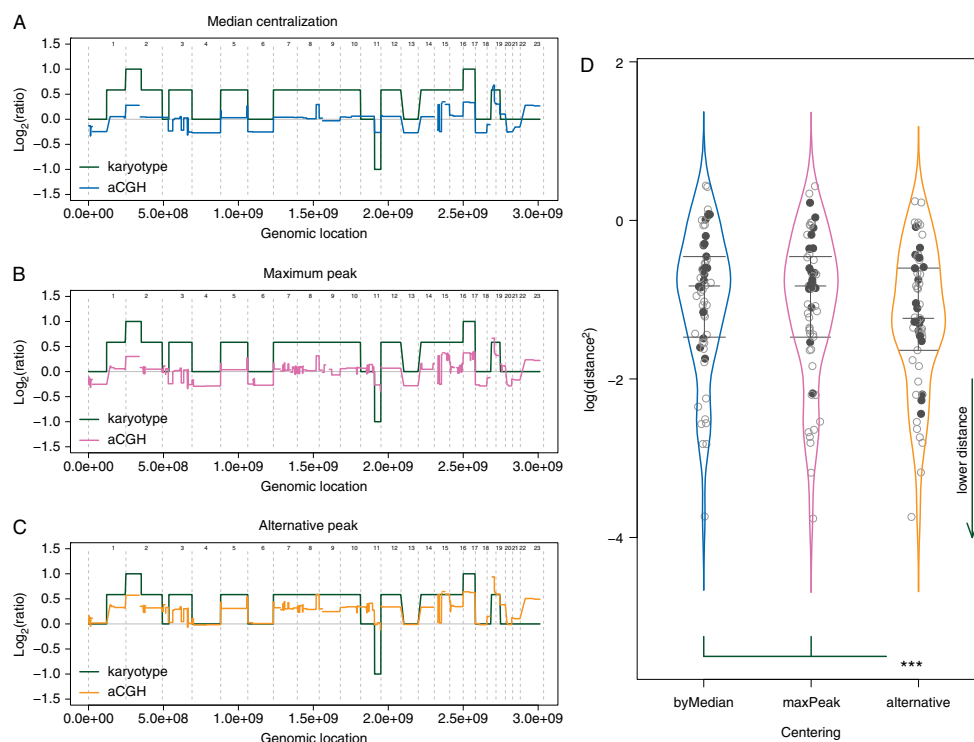
Figure 1. Distance from karyotypes. (A–C) In order to estimate the effect of the centralization methods, squared distances between genomic profiles (colored line) and karyotypes (green line) have been calculated. Distances are symbolized by the colored areas. (D) An alternative peak was available for 18 of the 57 analyzed cell lines (bold black points). Choosing the alternative peak for adjusting the genomic profiles significantly reduce the discrepancies with the corresponding karyotypes, compared with the other methods. P = 1.13e-4 and 6.35e-5 , compared with the maximum peak and the LogR median, respectively. Vertical colored curves represent the densities, and horizontal gray segments are the Q25, Q50, and Q75 quantiles of each distribution.
