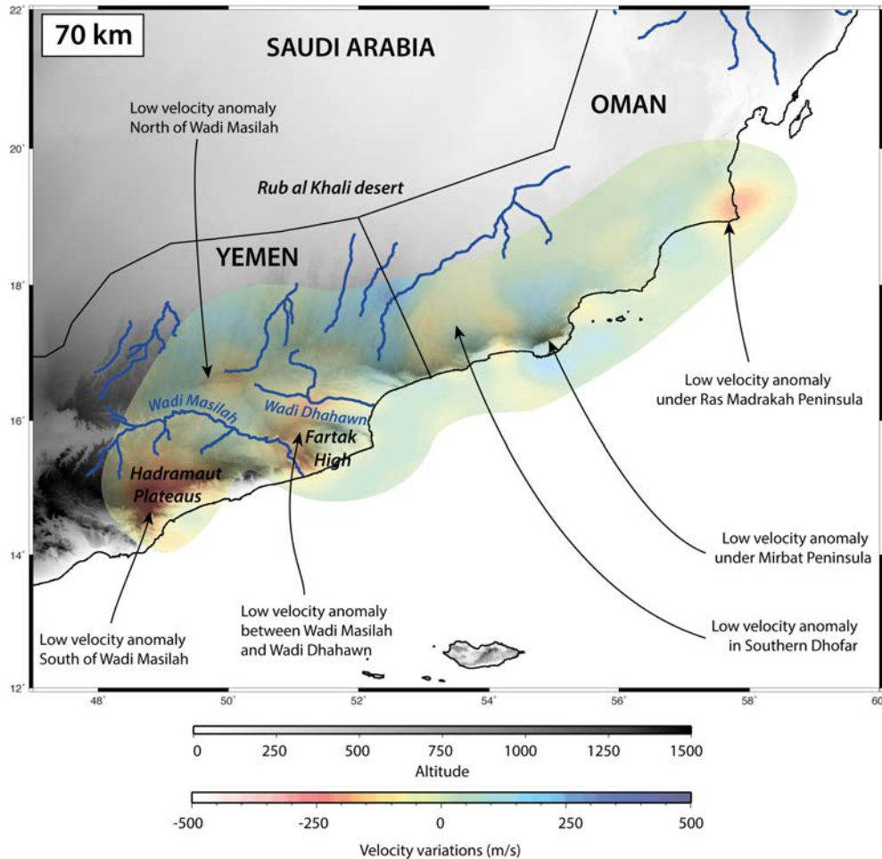
FIGURE IV.2.6: Map of the Oriental Gulf of Aden margin displaying the topography, rivers and a cross section of our solution model at 70 km depth. The bathymetry is not displayed in this figure.
