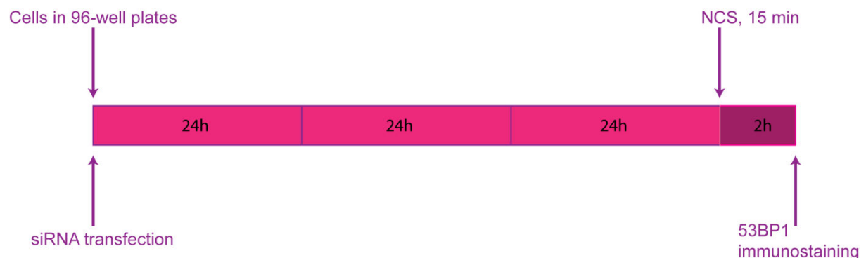
Figure 35- SiRNA screen
