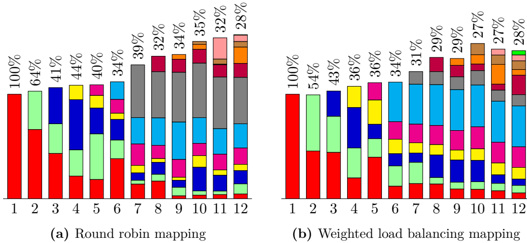
Figure 5.7: HEVC dataflow tasks load balancing using the Kimono input a fifo size of 8192 tokens for both mapping strategies. The X axis represents the number of dataflow tasks used to execute the application and the Y axis is the useful work executed by each dataflow task. The value on top of the plot, shows how many percents of the total work time are executed by the most loaded core.
