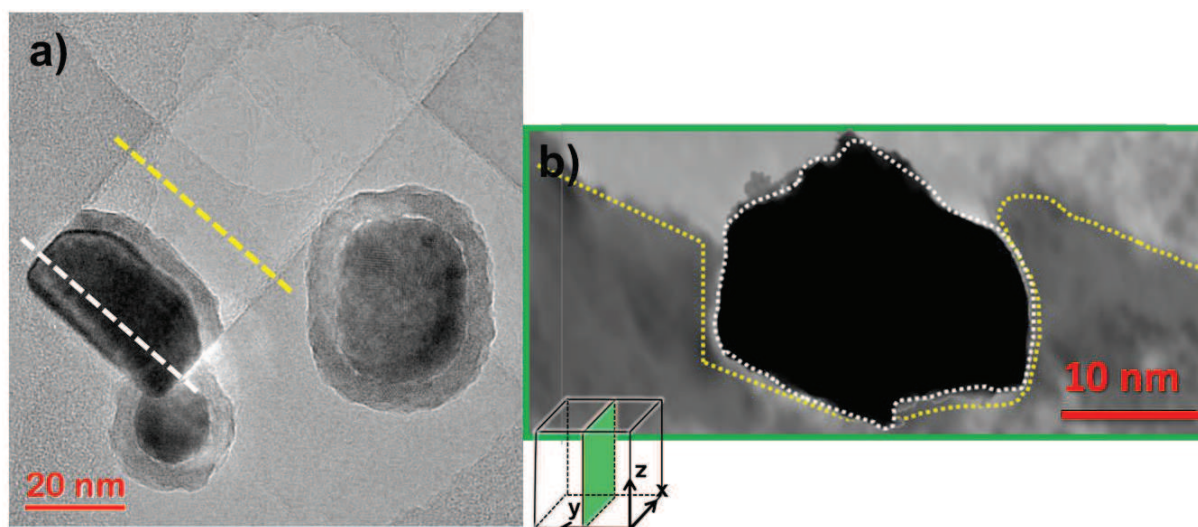
Figure 2.10. a) TEM projection of a channel and corresponding digging nanoparticle; b) Superposition of the xz slices of the nanoparticle (white line in Fig. 2.10a) and channel (yellow line) showing the close relationship between the 3D shape of the nanoparticle and the channel profile.
