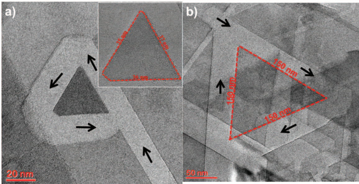
Figure 2.24. a) and b) Triangular patterns created by highly faceted \text{Fe}_x\text{N} nanoparticles due to their multiple turning points on uniform FLG surfaces.
