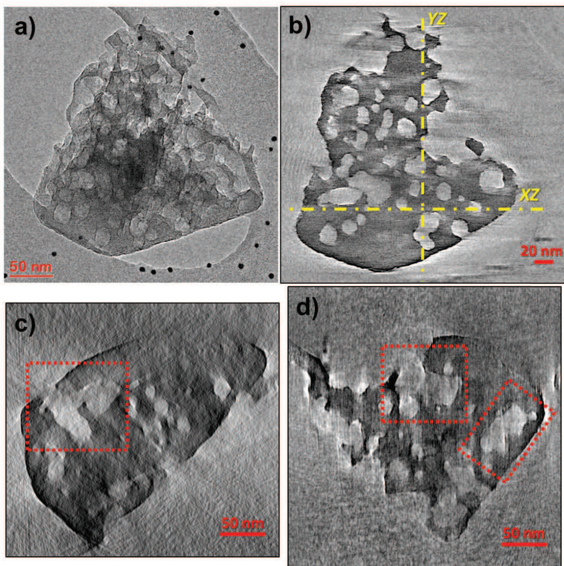
Figure 5.10. a) TEM projection (at 0^\circ ) of the zeolite grain selected for ET (F-ZSM-5-30 min). b) xy slice through the center of the reconstructed volume. The yellow lines highlight the cross-sectional directions presented in c) and d). c) and d) Slices in xz and yz directions, respectively, through the reconstructed volume at the positions highlighted in b).
