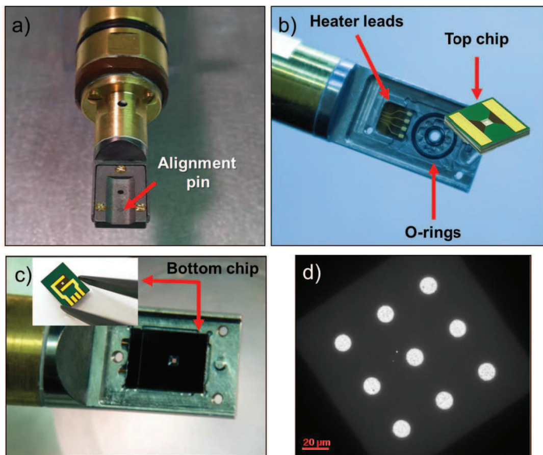
Figure 3.2. a) Bottom view of the Atmosphere E-cell holder compatible with JEOL UHP pole-piece configuration (2 mm gap). b) and c) Views of the inside of the E-cell. Images taken from Allard L. F. et al. 16 . d) Low-magnification image of the central part of the heating windows (SiC ceramic). The bright circles represent the analysis area covered only by SiN.
