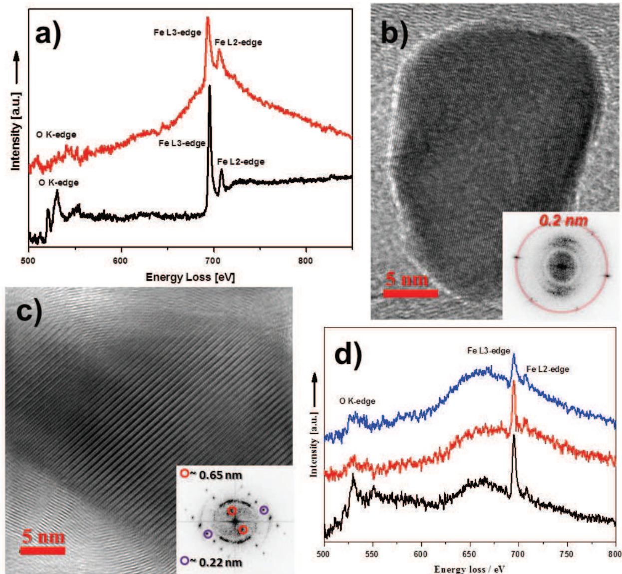
Figure 4.4. a) EELS spectra of the Fe based NPs filled CNT before (black line/ Fe 3-x O 4 ) and after (red line/metallic Fe and Fe x C y phases) the application of the voltage pulse.
