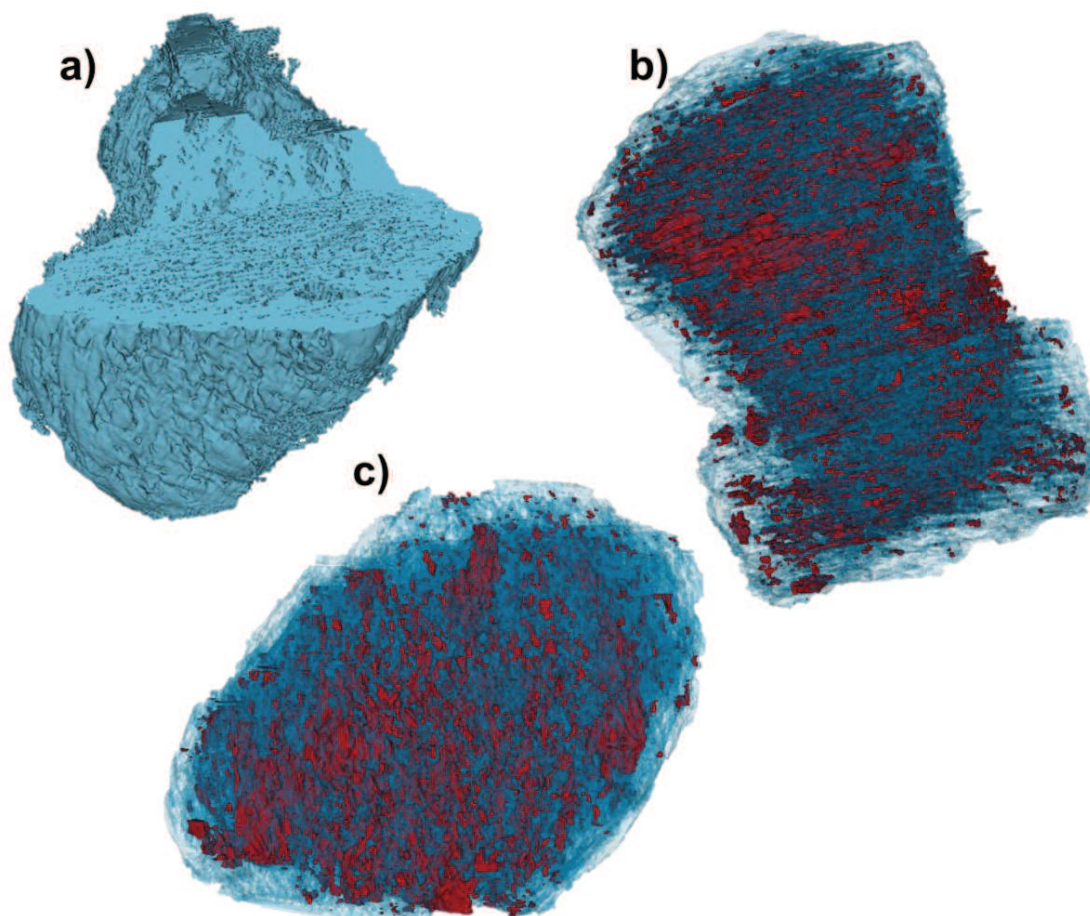
Figure 5.25. a) 3D model of the zeolite body cut in the xy and the yz directions. b) xy and c) xz oriented snapshots of the combined 3D models of zeolite body (transparent blue) and mesoporous network (red).
