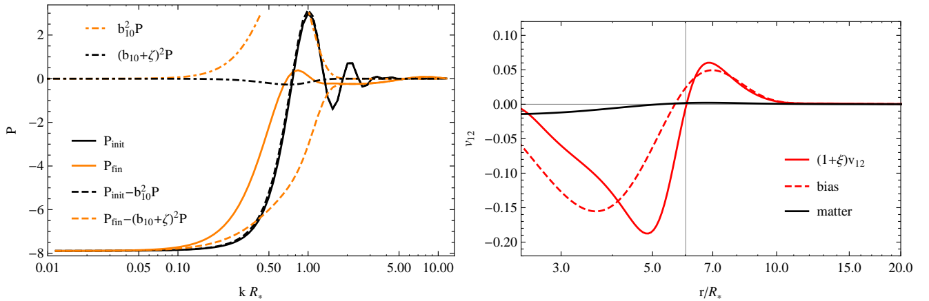
Figure 8. Left panel: Evolution of the peak-peak power spectrum and its noise component P_{\text{pk,pk}} - b^2 P from the initial conditions to the final configuration at \zeta = 7 . While the amplitude remains constant on large scales, the infall causes Right panel: Mean relative velocity v_{12} of 1D peaks (red solid). The peak velocities clearly deviate from the velocities of random dark matter particles (orange solid) on small scales. On large scales this deviation can be described by a linear velocity bias (red dashed), which however fails to describe the non-perturbative behaviour in the exclusion regime. We see that below r = 6R_* peaks are moving towards each other and away from each other for larger separations. The vertical gray line indicates the peak of the correlation function in Fig. 7. Note that on top of this mean flow, there is also a velocity dispersion.
