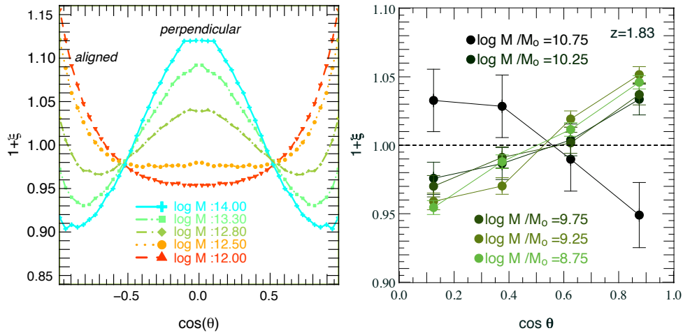
Figure 4.1: Left-hand panel: excess probability of alignment between the spin and the direction of the closest filament as measured from the 43 millions halos of the Horizon 4 \pi simulation ([Teyssier, 2002]) at redshift zero. Different colours correspond to different mass bins from 10^{12} (red) to 10^{14} M_\odot (blue) as labelled. A transition mass is detected at M_{\text{crit}}(z=0) \simeq 5(\pm 1) \times 10^{12} M_\odot : for halos with M > M_{\text{crit}} , the spin is more likely to be perpendicular to their host filament, whereas for halos with M < M_{\text{crit}} , the spin tends to be aligned with the closest filament. This figure is from [Codis et al., 2012] (see section 4.2). Right-hand panel: same as left panel for the 160 000 galaxies of the HORIZON-AGN hydrodynamical simulation at z = 1.8 ([Dubois et al., 2014]).
