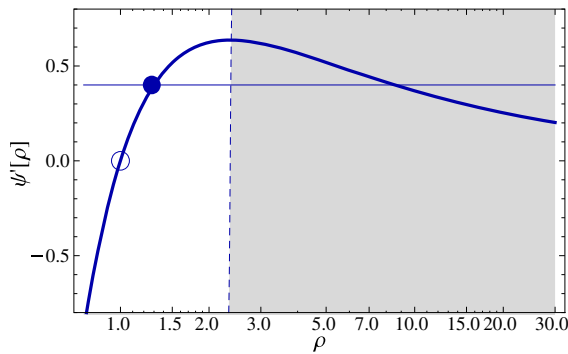
FIG. 1 (color online). A graphical representation of the one-dimensional stationary condition \lambda = \Psi'[\rho] . There is a maximum value for \lambda that corresponds to a critical value \rho_c for \rho defined in Eq. (42).
