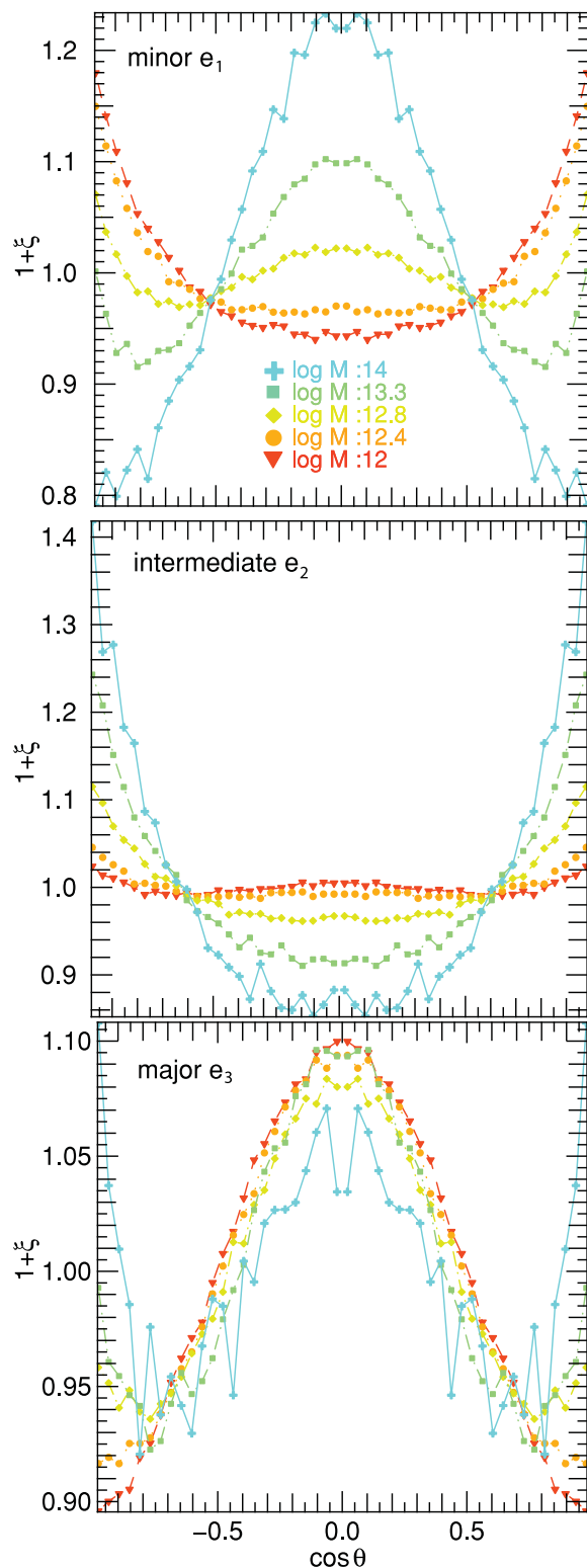
Figure A2. Excess probability of alignment between the spin and the minor/intermediate/major axis (from the top to bottom) of the tidal tensor in the Horizon 4 \pi simulation. Different mass bins are colour-coded from 10^{12} (red) to 10^{14} M_\odot (blue). A transition is detected: the spin of high-mass haloes tends to be aligned with the intermediate principal axis (middle panel), whereas the spin of low-mass haloes tends more likely to point along the minor axis (top panel).
