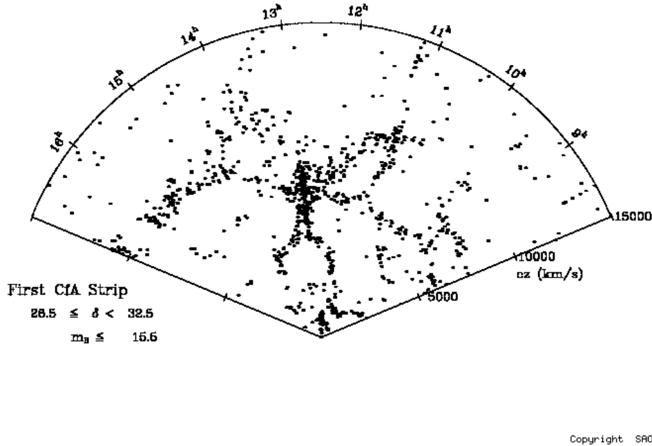
Figure 1.3: Galaxies are not uniformly distributed but form a bubble-like network as seen here in the CfA Redshift Survey ([de Lapparent et al., 1986]) where filaments of a few tens of megaparsecs join big clusters like the Coma cluster in the middle. The Coma Cluster looks elongated along the line-of-sight (creating the so-called “stickman” picture) because of redshift space distortions.
