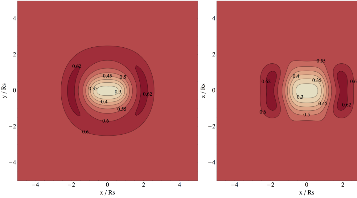
Figure 13. Alignment dispersion \tilde{\sigma} (defined in equation 29) around a typical filament-type saddle point of height \nu = 1.25\gamma , \lambda_1 = 0.31 , \lambda_2 = -0.56 , \lambda_3 = -1 for a power-law 3D power spectrum with spectral index n = -2 . The left-hand panel displays a cut along the plane, Oxy , of the saddle point and right-hand panel along the plane, Oxz , of the wall. The uncertainty on spin direction is smallest near the saddle.
