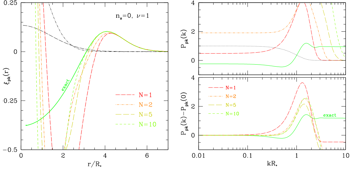
Figure 5. Left panel: Comparison between the exact correlation function of 1D peaks and perturbative series obtained upon truncating the peak bias expansion Eq.(23) at order N = 1, 2, 5 and 10. For illustration, the black curves show linear and quadratic local bias approximations and perform significantly worse than the peak bias expansion. A white noise power spectrum with Gaussian filtering and a peak height \nu = 1 were assumed. Top right: Exact peak power spectrum (solid) compared to various approximations obtained upon truncating the bias expansion at order N = 1, 2, 5 and 10. The solid curve is the density power spectrum. Bottom right: same as top panel but the zero-lag value P_{\text{pk}}(0) has been subtracted off from the power spectra. In all cases, a white noise power spectrum with Gaussian smoothing and a peak height of unity were assumed.
