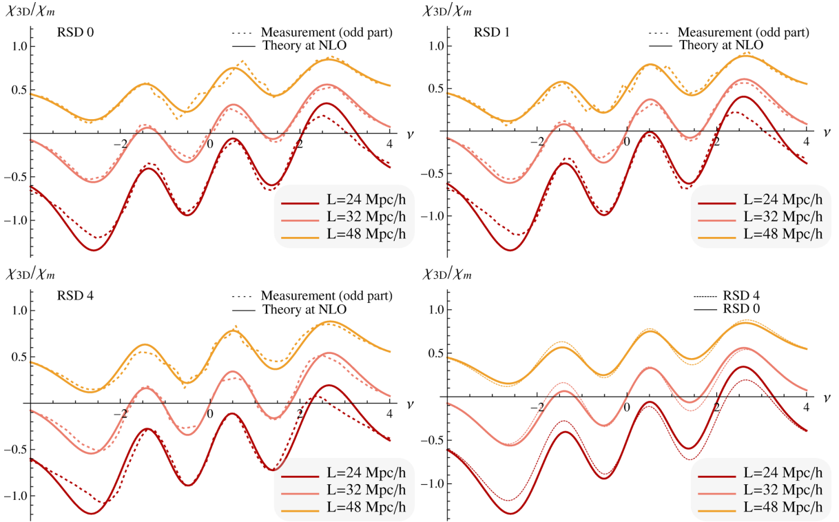
Figure 7. Top-left panel: first NG correction of the 3D Euler characteristic as a function of smoothing (as labelled) measured (dotted lines) and predicted (plain line) in HORIZON 4 \pi simulation in real space. Each curve has been normalized by the maximum of the Gaussian component of the Euler characteristic. Those corresponding to different smoothing lengths have been shifted for clarity. Top-right panel: same as the top-left panel, but in redshift space. Bottom-left panel: same as the top-right panel, but redshift displacements were boosted by a factor of 4. Bottom-right panel: theoretical prediction in real space and boosted redshift space. For these ranges of smoothing, the theory predicts well the Euler characteristic to first order in non-Gaussianity, in particular for low-intermediate thresholds. The difference in the Euler characteristic introduced by redshift distortion (even boosted by a factor of 4) is rather small.
