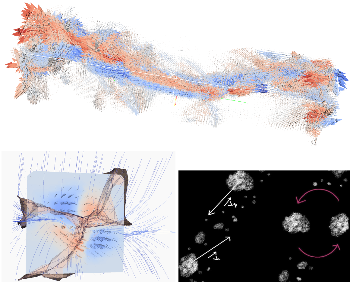
Figure 4.2: Top panel: Vorticity field along a filament colour-coded depending on its algebraic component parallel to the filament. Red arrows are going towards the left-hand side of the filament with blue arrows are pointing towards the right-hand side of that filament. Bottom left-hand panel: Typical cross section perpendicular to the filament. Bottom right-hand panel: Sketch of the merger of two halos along the filament. The orbital angular momentum is converted into an additional spin for the resulting object, that is perpendicular to the motion direction i.e perpendicular to the filament axis.
