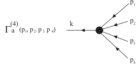
FIG. 2. Example of the multipoint propagator, \Gamma_a^{(4)} . A large filled circle symbolically represents all possible contributions that enter into the fully nonlinear propagator. A part of those contributions can be seen graphically using PT expansion (see Figs. 4 and 5 for three-point propagator \Gamma_a^{(2)} ).
