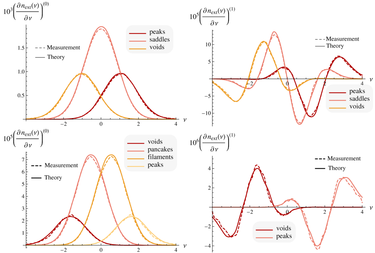
Figure B4. Top-left panel: the distribution of 2D extrema (voids, saddles and peaks as labelled) as a function of threshold \nu in redshift space for f = 1 as predicted at Gaussian order (solid) and measured (‘even part’ of the data only, see the main text for more details). Top-right panel: the corresponding NG correction ( f_{\text{nl}} = 0.05 ) estimated from 20 realizations of the corresponding scale-invariant ( n = -1 ) field of dimension 4096^2 smoothed over 4 pixels as predicted at first NG order (solid) and measured (‘odd part’ of the data only). Bottom panels: same as the top panels for the distribution of 3D extrema (voids, wall saddles, tube saddle and peaks as labelled) for NG scale-invariant ( n = -1 , 256^3 smoothed over 4 pixels) anisotropic field ( f_{\text{nl}} = 0.07 , f = 1 ).
