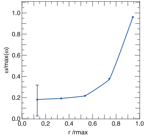
Figure 10. Azimuthal average of the radial profile of the vorticity. The profile is obtained by averaging on the sections of a complete filament (each section is associated with a filament segment, to which the section is perpendicular). Vorticity is clearly larger towards the caustic, and would theoretically become singular (as 1/\sqrt{1-r/r_{\text{max}}} ) at the caustic for a Zel'dovich mapping, as shown in Pichon & Bernardeau (1999). Here the profile is convolved by shape variations from one caustic to another and by the azimuthal average. The indicative error bar was computed as the average over a larger stack.
