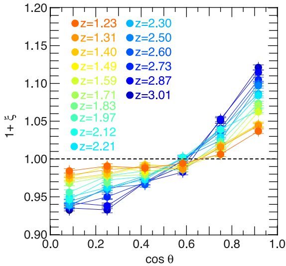
Figure 8. Excess probability \xi of the alignment between the spin of galaxies (with mass above 10^8 M_{\odot} ) and their closest filament as a function of redshift is shown. Dashed line is the zero excess probability \xi = 0 . The amplitude of the correlation shows an alignment which increases with redshift (i.e. decreases with cosmic time).
