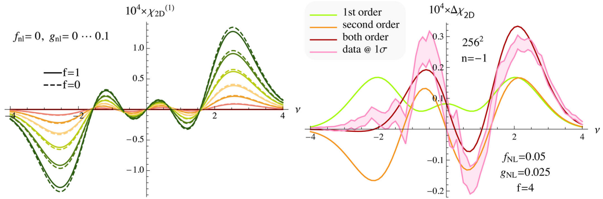
Figure B3. Left: variation with the amplitude of g_{\text{nl}} of the predicted Euler characteristic at NLO of a mildly 2D NG anisotropic field. Right: match between a given realization with f_{\text{nl}} and g_{\text{nl}} as labelled, and the corresponding model decomposed into first-order ( n = 3 ) and second-order ( n = 4 ) corrections.
