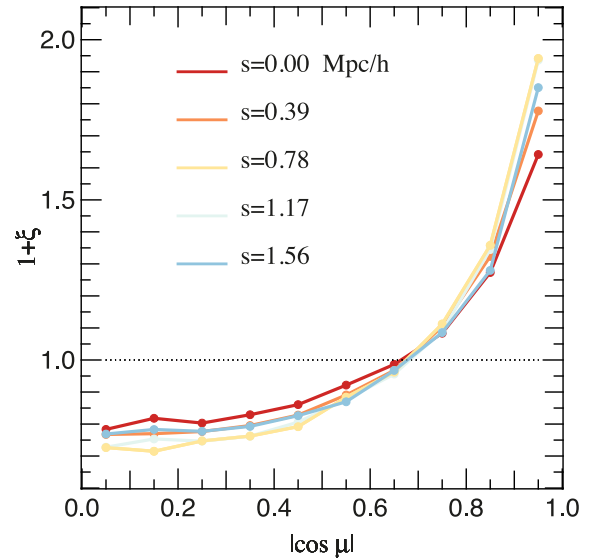
Figure D1. The probability distribution of the cosine of the angle between the vorticity and the direction of the filament, measured in S_{100}^{\text{CDM}} for various smoothing scales of the velocity field before computation of the vorticity. Smoothing scales are expressed in h^{-1} Mpc. The smoothing scale adopted in the main text is 0.39 h^{-1} Mpc.
