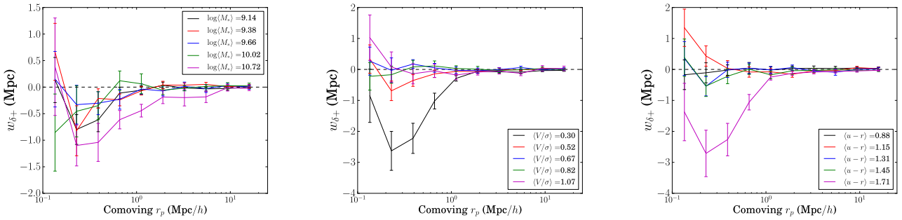
Figure 12. w_{\delta+} projected correlation functions for 5 bins of mass (left panel) and V/\sigma (middle panel) and u - r colour (right panel). The legend indicates the mean of the considered property in each bin, and the 5 bins are approximately equally populated. For simplicity, we only show the correlations that correspond to shape measurements using the simple inertia tensor. The impact of using the reduced inertia tensor is shown in Figure 11.
