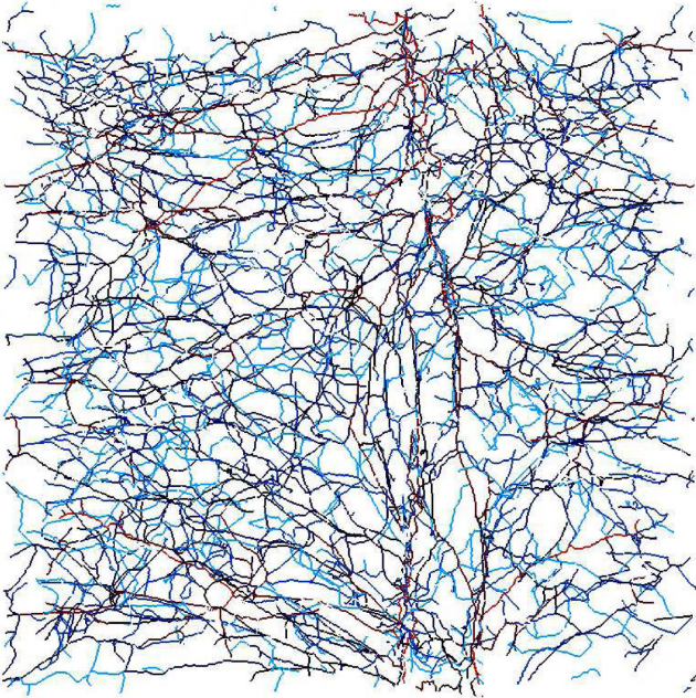
Figure C2. The skeleton measured in S_{20}^{\text{cool}}(0.7) for increasing persistence threshold, 0.06, 0.12, . . . , 2, from light blue to red; the skeleton has tree-like structure where the main branches correspond to the most persistent ones. The level of persistence of the main text corresponds to the dark blue and red branches.
