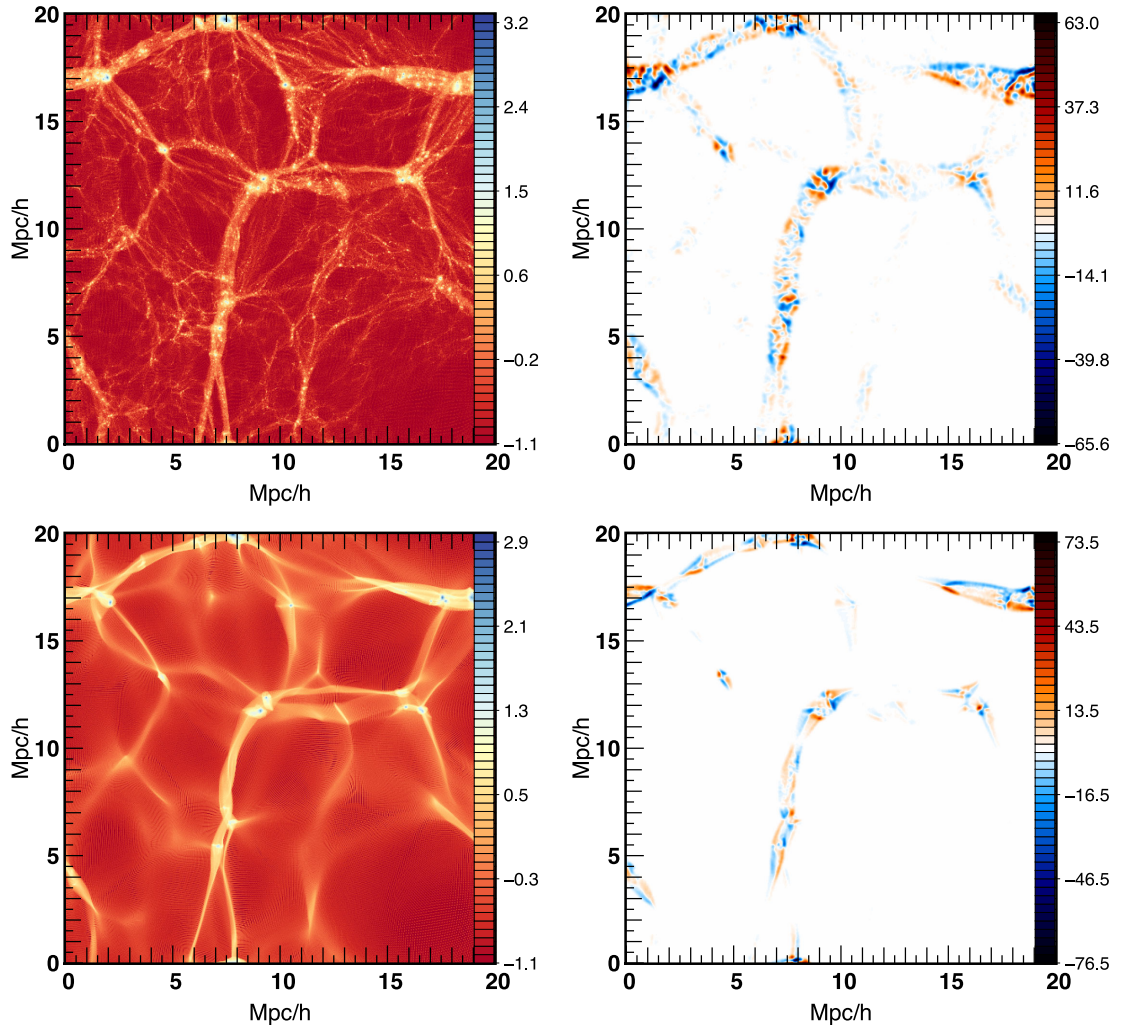
Figure 1. A thin slice ( 2h^{-1} Mpc thickness) of the projected DM density (left panels) and the projected vorticity along the normal to the slice in unit of h \text{ km s}^{-1} \text{ Mpc}^{-1} (right panels). DM density is plotted with a logarithmic scale. Vorticity is computed after smoothing of the velocity field with a Gaussian filter of 160 h^{-1} \text{ kpc} for this figure only. The geometry of the vorticity closely follows the LSS, but switches polarity across the walls/filaments (recalling that walls appear as filaments and filaments as peaks in such a cross-section). Note also how the vorticity is localized around filaments (the 2D peaks, as exemplified in Fig. 7). The two panels allow for a comparison between a section of \mathcal{S}_{20}^{\text{CDM}} (top) and \mathcal{S}_{20}^{\text{HDM}} (bottom). In \mathcal{S}_{20}^{\text{HDM}} , high-frequency modes are suppressed but the low-frequency vorticity is qualitatively consistent with that found in the realistic \mathcal{S}_{20}^{\text{CDM}} . On the bottom left panel, the density caustics are quite visible and correspond to the outer edge of the multi-flow region in the bottom right panel.
