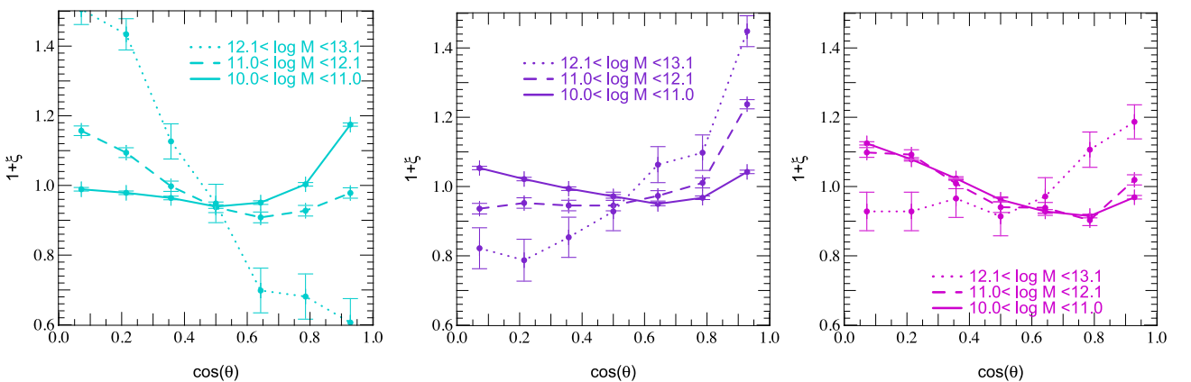
Figure A1. Same as Fig. 3 for DM haloes in the HORIZON-AGN simulation. The three different axes of the tidal tensor are colour coded from cyan ( e_1 ) through purple ( e_2 ) to magenta ( e_3 ). Different mass bins are coded from solid ( 10^{10} – 10^{11} M_\odot ) to dotted ( 10^{12} – 10^{13} M_\odot ) through dashed lines ( 10^{11} – 10^{12} M_\odot ). A transition is detected: the spin of high-mass haloes tends to be aligned with the intermediate (centre purple panel) and with less probability major (right-hand magenta panel) principal axis, whereas the spin of low-mass haloes is more likely to point along the minor axis (left-hand cyan panel). Those findings are consistent with previous studies of DM-only simulations.
