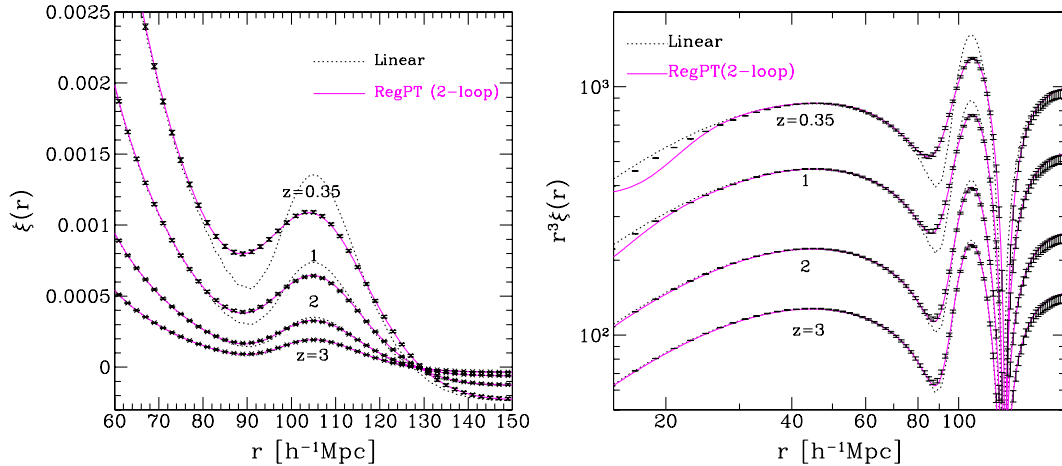
FIG. 10 (color online). Comparison of two-point correlation function between N -body and REGPT results at z = 3, 2, 1, and 0.35 (from bottom to top). In each panel, magenta solid, and black dotted lines represent the prediction from REGPT and linear theory calculations, respectively. Left panel focuses on the behavior around baryon acoustic peak in linear scales, while right panel shows the overall behavior in a wide range of separation in logarithmic scales. Note that in right panel, the resulting correlation function is multiplied by the cube of the separation for illustrative purpose.
