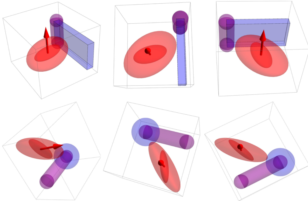
Figure 3. Sketch of main differential alignment between halo shapes and tidal tensor responsible for e_z - and e_\phi -component of momentum. Top: the two tensors in light and dark red, end up being misaligned as they feel differently the neighbouring wall (blue) and filament (purple), inducing a spin parallel to the filament (red arrow). Three projections are shown for clarity. Bottom: correspondingly, the differential pull from the filament (purple) and the density gradient towards the peak (blue) generates a spin (red arrow) along the azimuthal direction. By symmetry, the other peak(s) on the other side of the saddle point will spin-up massive haloes in the opposite direction.
