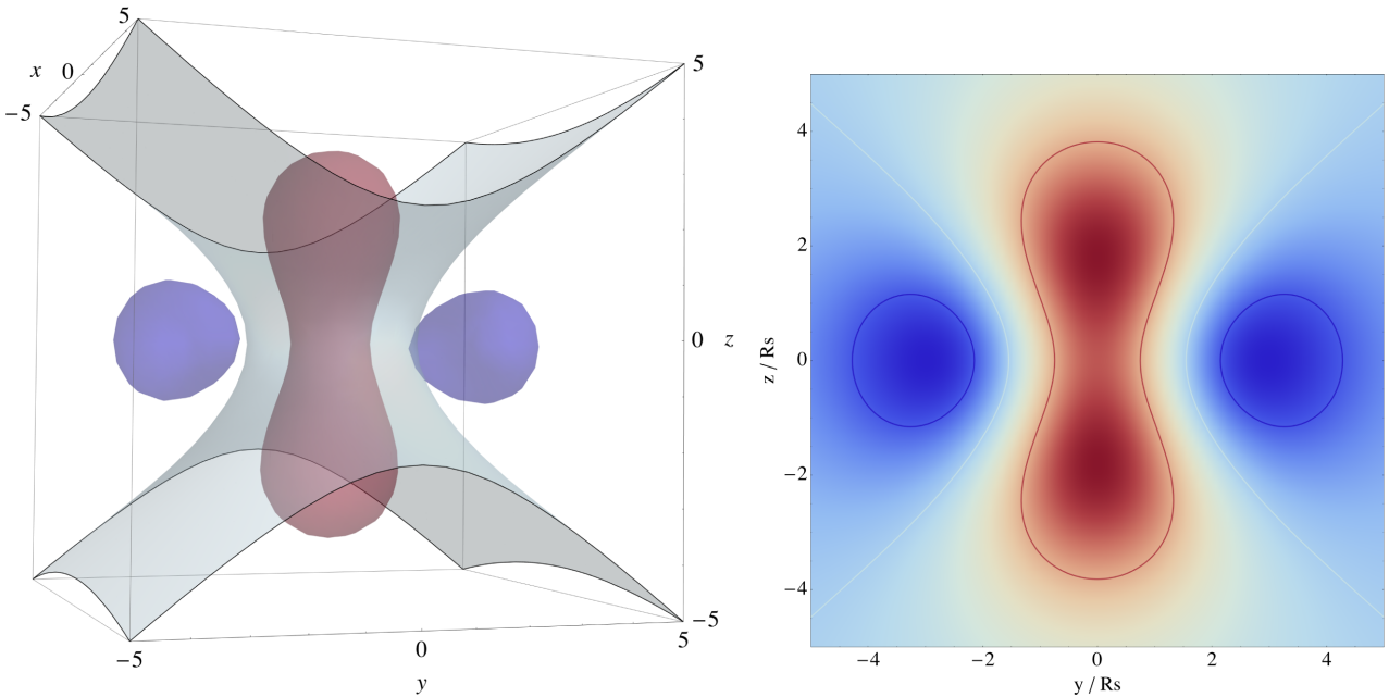
Figure 11. Mean density around a filament-saddle point of height \nu = 1.25\gamma , \lambda_1 = 0.31 , \lambda_2 = -0.56 , \lambda_3 = -1 for a power-law 3D power spectrum with spectral index n = -2 , i.e. \gamma = \sqrt{3}/3 . The O_x -, O_y - and O_z -axes are in units of the smoothing length and z is the direction of the filament while the wall is in the plane Oxz . Contours represent the isocontours of the density \delta = -0.3, 0, 0.5 from blue to red. A 3D view is displayed on the left-hand panel and a cut in the plane Oyz is shown on the right-hand panel.
