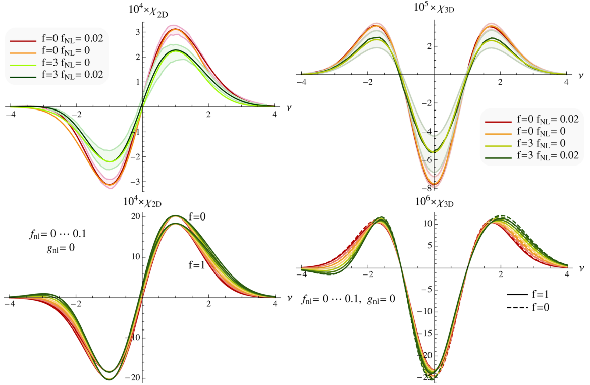
Figure B1. 2D (left) and 3D (right) Euler characteristic of a mildly NG anisotropic field in a toy model. Top left: comparison with measurements for different values of the quadratic parameter f_{\text{NL}} and anisotropy f , as labelled. The shaded area corresponds to the one-sigma measurement error on realizations of the NG fields. The overall amplitude has been rescaled by 10^4 . Note both the change in amplitude with f and the distortion in the tails of the distribution with f_{\text{NL}} which are well fitted by the model. Bottom-left panel: theoretical evolution of the 2D Euler characteristic as a function of f_{\text{NL}} as labelled for f=0 and 1. For this level of anisotropy, the difference in amplitude is less significant. Top-right and bottom-right panels: same as the corresponding left-hand panels in 3D.
