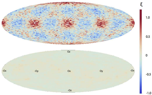
Figure A3. Distribution of spins (top panel) and separation vectors of galaxy pairs separated by less than 25 \text{ Mpc}/h (bottom panel) on the sphere. The excess probability \xi defined so that the PDF reads P(\cos \theta, \phi) = (1 + \xi)/4\pi is colour-coded from dark blue (-1) to dark red (+1). If the spins are clearly correlated with the box axes, this is not the case of the separation vectors for which the magnitude of the excess probability is smaller (lighter colours) and the pattern does not seem to be correlated with the grid.
