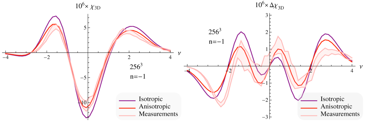
Figure 3. Left-hand panel: 3D Euler characteristic of a mildly NG scale-invariant cosmological field ( n = -1 , f = 1 , \sigma = 0.18 ). The prediction to first order in non-Gaussianity given by equation (35) corresponds to the red solid line and the prediction assuming isotropy (see equation 38) to the purple line. The one-sigma shaded area is the measurement. Right-hand panel: same as the left-hand panel for the first-order correction to the Gaussian distribution only.
