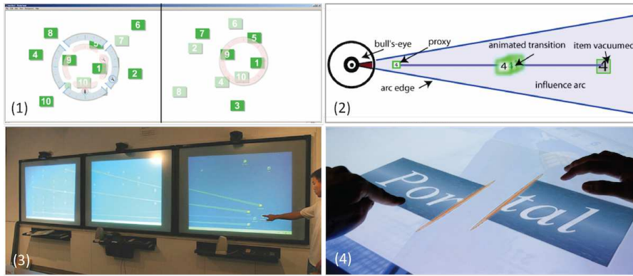
Figure 61: Examples of techniques for remote interaction on large displays. (1) Frisbee: the left widget is the “Telescope” and the right widget is the “target” [63]; (2) The Vacuum: the proxy of target 4 is generated close to the circular widget [11]; (3) Drag-and-Pop: proxies of remote targets are generated close to the moving object [25]; and (4) Dynamic Portals: portals are created by drawing lines on the display, and the content dragged into one portal comes out from the others [112].
