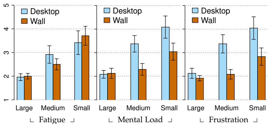
Figure 45: Physical fatigue, mental load and frustration on a five-point Likert item (1 is best, 5 is worst) for each LABELSIZE condition.
