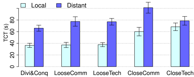
Figure 52: Mean Task Completion Time by STYLE × LAYOUT conditions.
