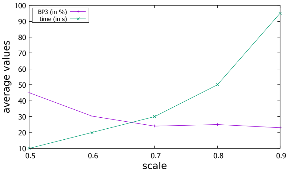
Figure 4.6: Percentage of average bad-pixels at AEPE threshold of 3 pixels (BP3) and average computation time as a function of the scale-factor ( \alpha_{scale} ). The values are given for a combined MATLAB/C- implementation of the proposed algorithm ( ROF-NND with k = 1 ) tested on large displacement image pairs (#117, #144, #147 and #181) of the KITTI training dataset.
