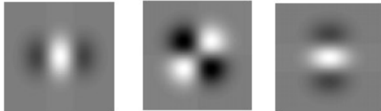
Figure 3.2: Representation of Riesz wavelet basis filters of order 2 ( N = 2 ).
