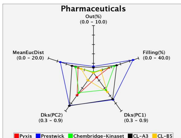
Figure 10: radar graph of the DRCS based diversity indices computed for five chemical libraries. The DRCS model and the pharmaceuticals contour were used for all the calculations.
