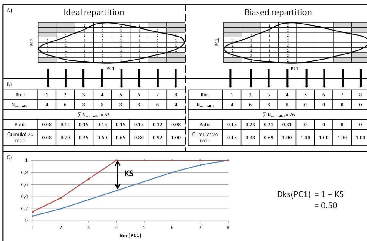
Figure S7: For two fictive libraries made of 52 products (then 52 cells inside the DRCS), description of the successive steps for the D_{\text{ks}}(\text{PC1}) indice calculation. A) compounds are projected inside the DRCS and associated to a cell of the optimized grid. B) for PC1, each column of the grid is considered as a bin. For each bin i the ratio between the number of occupied cells in the bin and the total number of occupied cells in the DRCS is computed. Then the cumulative ratio from the first to the last bin is obtained. C) the experimental (here biased) cumulative ratio is compared to the cumulative ratio for the ideal repartition to obtain the KS. The D_{\text{ks}}(\text{PC1}) index is deduced from the KS value.
