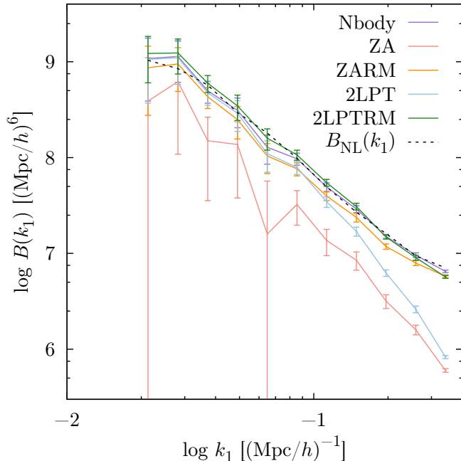
Figure 2.6: Redshift-zero dark matter bispectra for equilateral triangle shape, in 1024 \text{Mpc}/h simulations, with density fields computed on mesh of 8 \text{ Mpc}/h size. The particle distribution is determined using: a full N -body simulation (purple curve), the Zel’dovich approximation, alone (ZA, light red curve) and after remapping (ZARM, orange curve), second-order Lagrangian perturbation theory, alone (2LPT, light blue curve) and after remapping (2LPTRM, green curve). The dashed line, B_{\text{NL}}(k) , corresponds to theoretical predictions for the bispectrum, found using the fitting formula of (Gil-Marín et al. , 2012). Note that both ZARM and 2LPTRM show increased bispectrum in the mildly non-linear regime compared to ZA and 2LPT, indicating an improvement of three-point statistics with the remapping procedure.
