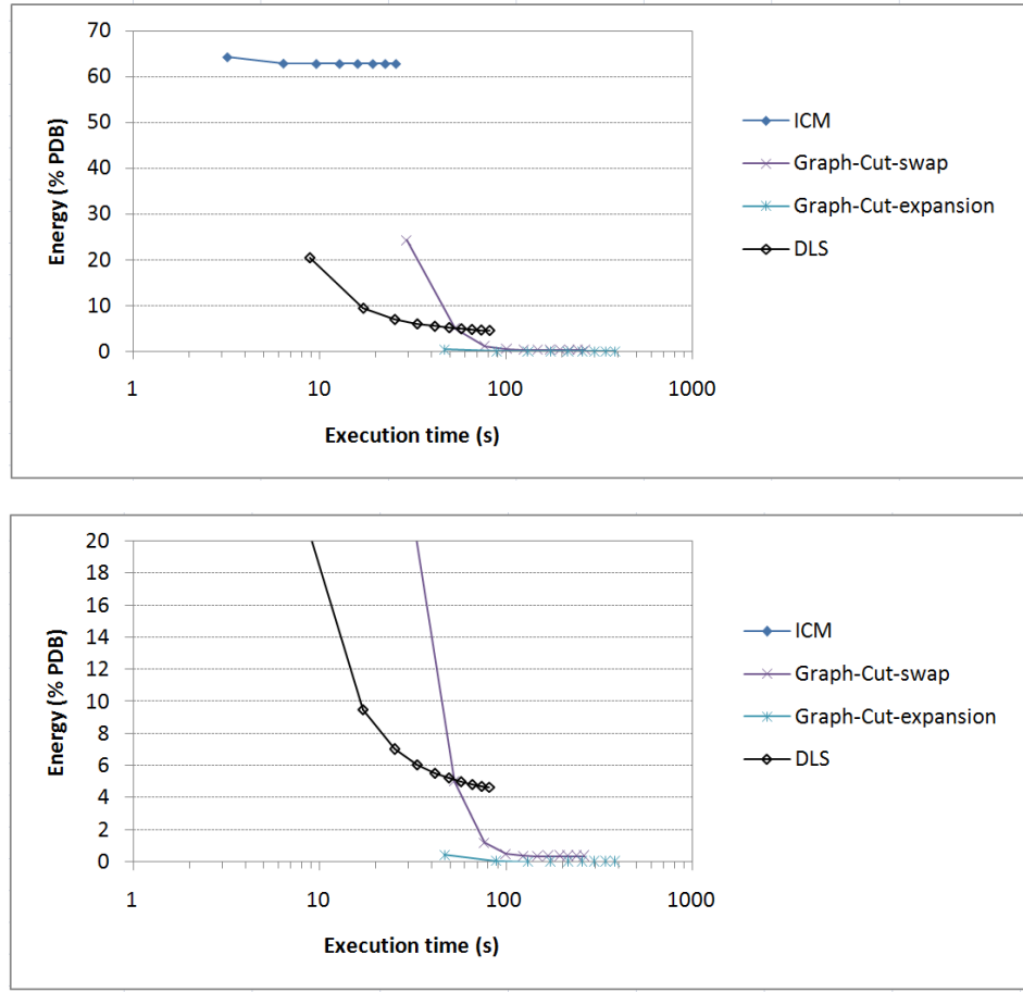
FIGURE 7.6: Different energy minimization methods on half size Teddy ( 900 \times 750 ) stereo matching benchmark with large disparity range. The disparity range is set to 128 pixels. Note that the execution time is shown on the x -axis using a log scale. The lower chart is a zoom-in of the upper chart.
