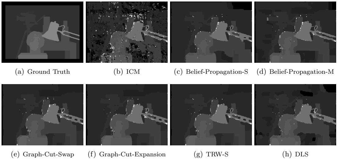
FIGURE 7.7: Disparity maps for Tsukuba ( 384 \times 288 ) benchmark obtained with different energy minimization methods. The disparity range is set to 64 pixels.
