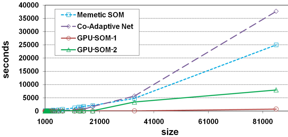
(b) execution time according to instance size
