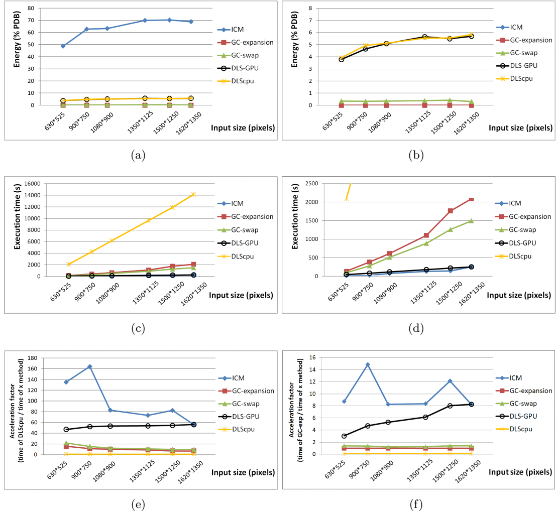
FIGURE 7.9: Stereo matching on Teddy benchmarks with different sizes. (b) and (d) are zoom-in parts of (a) and (c). The plot in (e) illustrates the acceleration factor computed according to the slowest method (DLScpu), while the plot in (f) illustrates the acceleration factor computed according to the method (GC-expansion) that gets the lowest energy. For the stop condition, the ICM method, and the graph cuts based methods (GC-expansion and GC-swap) run until convergence when no lower energy can be further found; the DLS methods (DLS-GPU and DLScpu) run for 100 iterations. The disparity range is set to 128 pixels.
