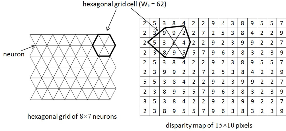
FIGURE 2.4: Hexagonal structured mesh with honeycomb cells and triangular subdivision (left part). Disparity map covered with a single honeycomb cell with weight W_k = 62 (right part).
