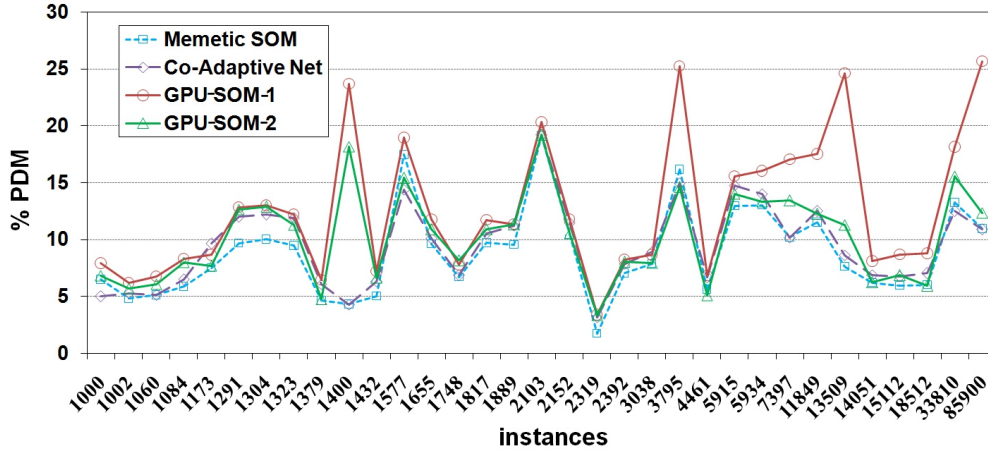
(a) percentage deviation of the mean solution value over 10 runs
