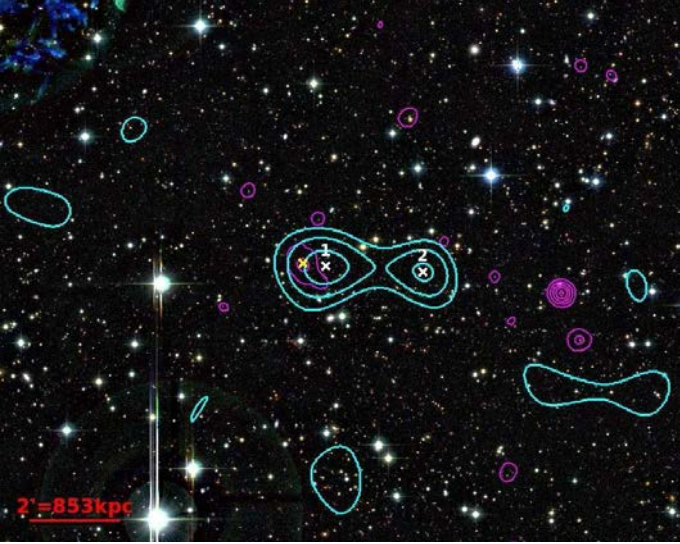
Fig. 11. Same as Fig 5 for NEP200 on the 3-color CFHT/MegaCam image. We expect 1.6 fake peaks above 3\sigma_\kappa and 0.3 above 4\sigma_\kappa in the displayed field (see Sect. 4.2 for details).
