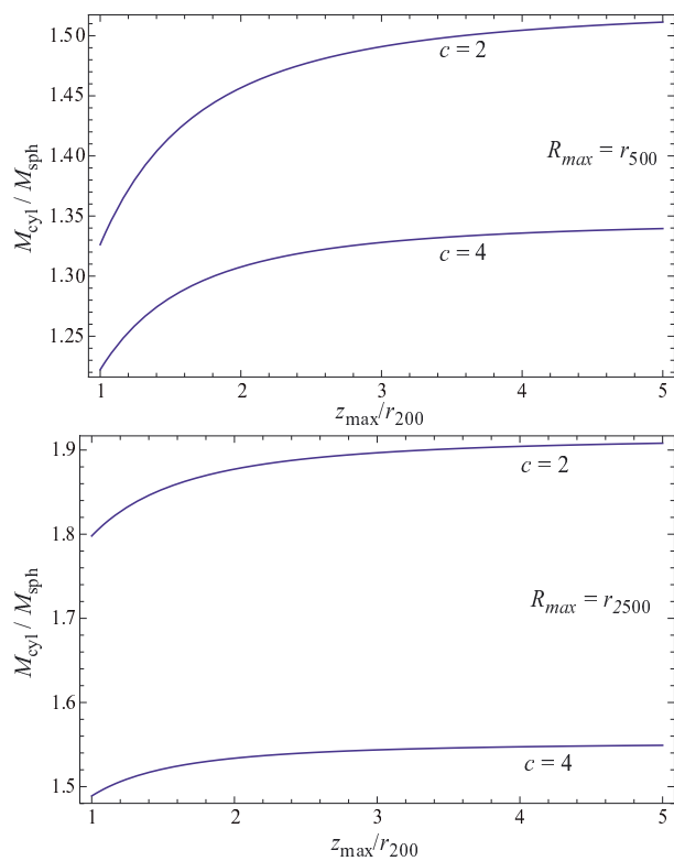
Fig. B.1. Upper panel: for a fixed R_{\text{max}} = r_{500} , mass excess as a function of z_{\text{max}} / r_{200} , for two NFW concentration parameters c . Lower panel: same as upper panel but for R_{\text{max}} = r_{2500} .
