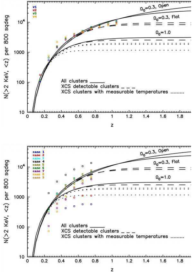
Fig. 3. Cumulative number of clusters hotter than 2 keV expected in a region of 800 deg 2 for different cosmologies as a function of redshift, taken from Romer et al. (2001), Fig. 5. The numbers of clusters in the four CFHTLS-Wide fields are shown in the top figure, and the numbers detected in Stripe 82 for the various cases described in Table 1 (see text) are plotted in the bottom figure. Only clusters detected at a 4\sigma level and above are taken into account.
