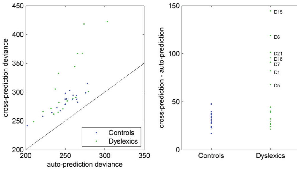
Figure 4. Auto- and cross-predictions for all participants. Left panel: cross-prediction deviance as a function of auto-prediction deviance. The dotted line indicates the cross-prediction = auto-prediction line. Right panel: difference between cross- and auto-prediction deviances for the two groups.
