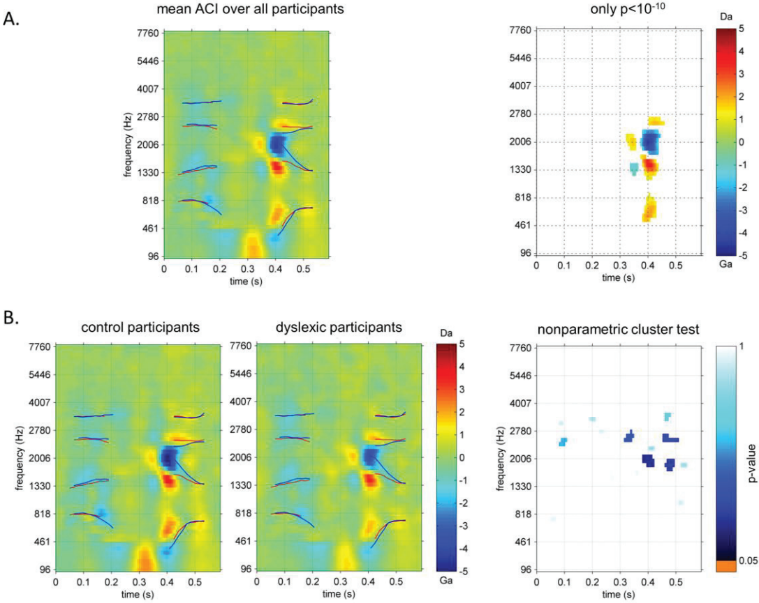
Figure 3. Diagram of the group-analysis of ACIs used in this study. A. mean ACI over all participants (left) and same ACI with all non-significant pixels ( p > 10^{-10} ) plotted in white (right panel) defining the regions used in the ROI analysis. B. mean ACIs for the control (left panel) and dyslexic (center panel) groups and output of the cluster-based non-parametric test (right panel). In the ACIs, lines correspond to mean formant trajectories for /alda/ and /aʁda/ (red) and for /alga/ and /aʁga/ (blue).
