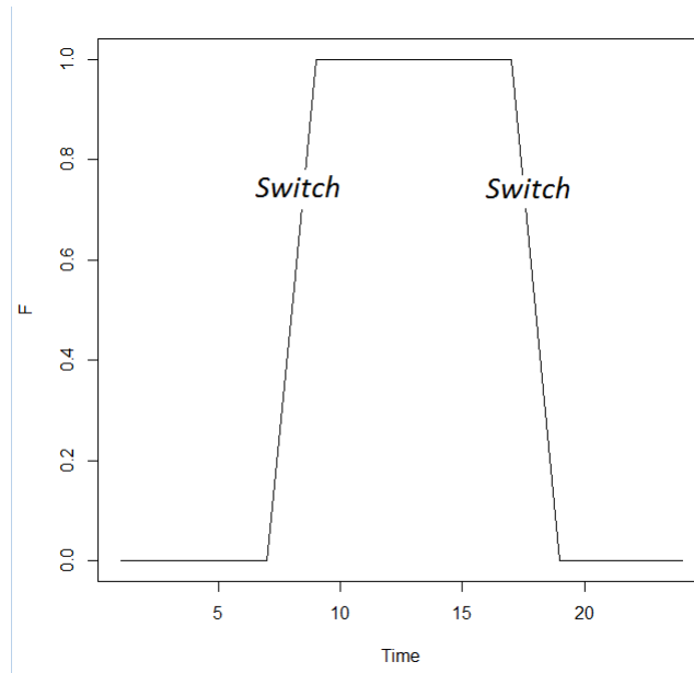
FIGURE III.21 – Fonction H
