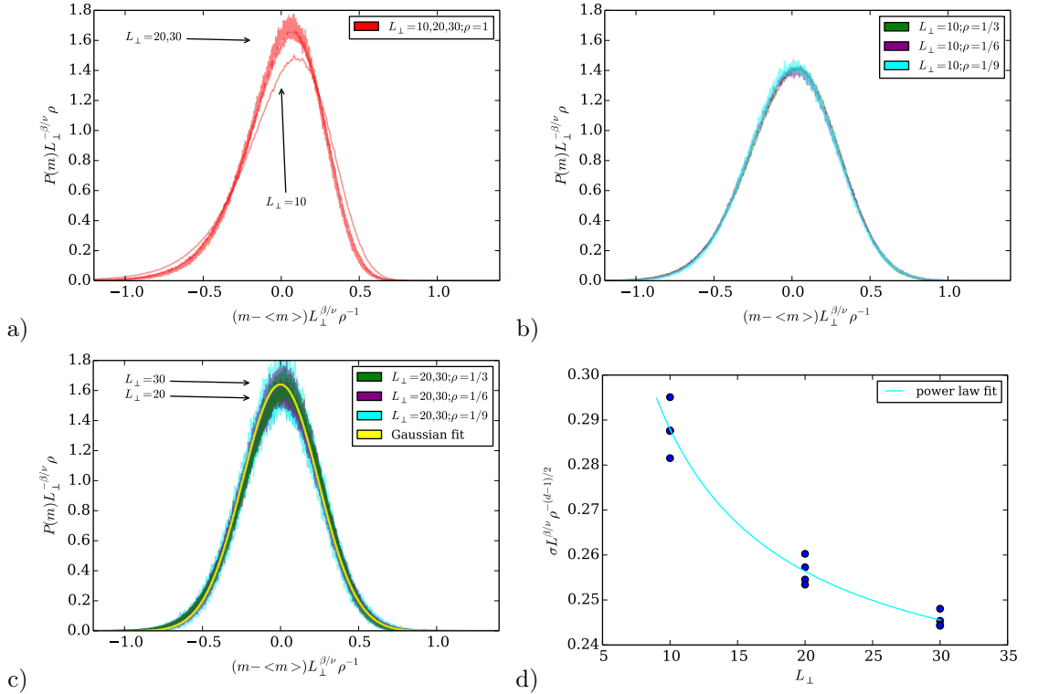
Figure 3.6: Results obtained by Monte-Carlo simulation of 3D Ising system with fixed (+) BC for various system thicknesses L_\perp and aspect ratios \rho at the critical temperature T = T_c^{3D} . a,b,c ) L_\perp^{-\beta/\nu}\rho P(m - \langle m \rangle) versus (m - \langle m \rangle)L_\perp^{\beta/\nu}\rho^{-1} . For the sake of visibility, we have separated the most skewed distribution for \rho = 1 ( a ) and the smallest system thickness L_\perp = 10 for which the variance is notably different from larger system thickness ( b ). For systems with L_\perp \geq 20 and \rho < 1 , we obtain a convincing collapse within the current precision ( c ). The continuous line is a Gaussian fit on data obtained with the largest system available. d ) We can verify that the standard deviation follows Eq.3.7 by plotting \sigma as a function of L_\perp^{-\beta/\nu}\rho . The points for which this relation seems less verified are for the smallest system thickness L_\perp = 10 , confirming previous observations. Points color give L_\perp . The continuous line is a linear evolution based on data for L_\perp = 30 .
