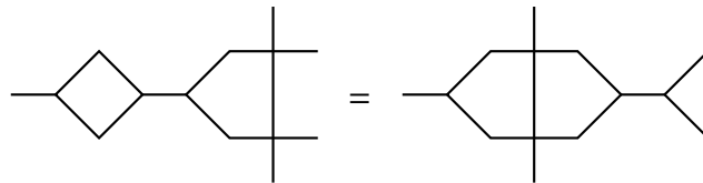
FIGURE B.6 – Attaching Y to the Yang–Baxter equation Fig. B.5 where z_1 = z_2 q^{-2} .
