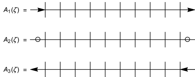
FIGURE 1.4 – Graphical representation of the A_1 (top), A_2 (middle) and A_3 (bottom) operators.
