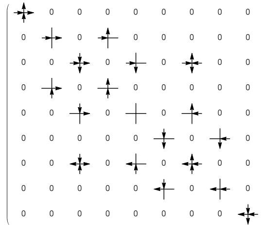
FIGURE 1.3 – The nineteen vertices of the R -matrix are the nonzero elements here. Their Boltzmann weights can be read off from Eq. (1.3).
