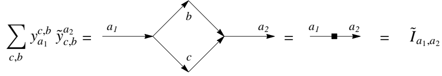
FIGURE B.4 – Unitarity relation for Y^T and Y .
