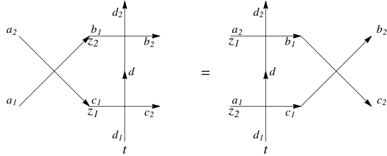
FIGURE B.5 – The Yang–Baxter equation with the \check{R} .
