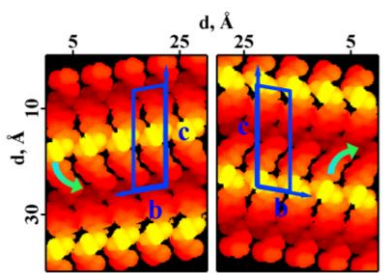
Figure II.1.5. Calculated topography of the PTT crystal bc -plane reveals two different chiral conformations when viewed along the positive and negative crystallographic a -axis. ( left ) view on the negative bc -plane, ( right ) view on the positive bc -plane,
