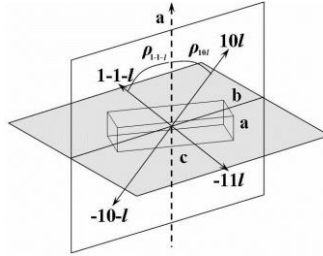
Figure III.3.3 Cartoon showing the position of the off-meridional doublets of the first layer line in respect to the a -axis (dotted arrow). The two corresponding vectors and the a -axis are lying in one plane (depicted in gray), while the azimuthal angle \rho is almost identical for the two corresponding vectors.
