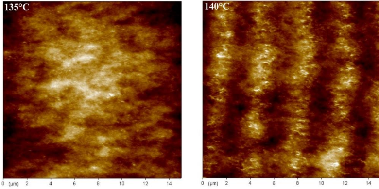
Figure IV.4.3. AFM images of the free-standing films of PTT crystallized from the melt at 135°C (left) and 140°C (right). The micrograph in the left panel does not reveal any banded spherulite morphology.
