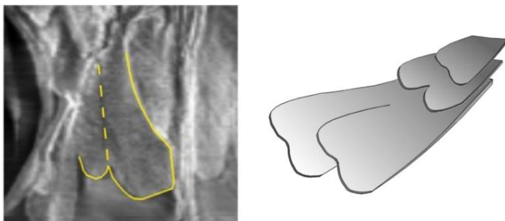
Figure IV.4.30. High-temperature AFM micrograph of a growth front of PTT-lamellar crystal at 210°C showing splitting of the lamella tip while growing radially [28] ( left ). Cartoon depicting the mechanism of crystal splaying due to surface stresses ( right ).
