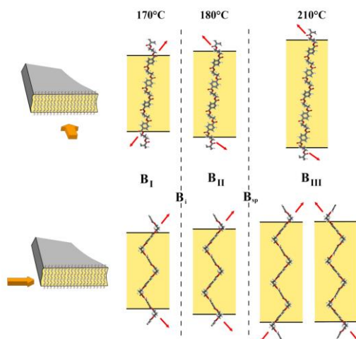
Figure IV.4.21. Cartoon depicting an idealized molecular model of the PTT lamellae below and above inversion temperature B_I and the unlocking temperature B_{sp} . Projections parallel ( top ) and perpendicular to ( bottom ) the crystal growth direction.
