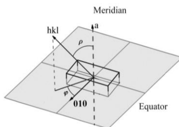
Figure III.3.2. Schematic drawing of an arbitrary reflection \mathbf{hkl} and its angle with respect to the meridian \mathbf{a} (azimuthal angle \rho ) and the angle between the projections the \mathbf{hkl} vector on the plane normal to the meridian and \mathbf{010} vector (fiber angle \varphi ).
