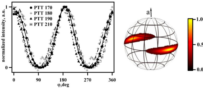
Figure V.4.11. Normalized integral intensity of the 010 reflection as a function of the fiber angle \varphi for different crystallization temperatures of PTT indicated on the graph (left). The curves reveal virtually no variation of the fiber-angle broadening with crystallization temperature. Pole figure corresponding to the 010 reflection (right).
