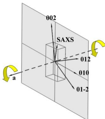
Figure IV.4.10. Crystallographic model of the lamellar twisting in a PTT film crystallized at 190°C. The rotation axis is parallel to the crystallographic a -axis. The vectors corresponding to the equatorial 0kl reflections rotate in the b * c *-plane. The sense of the crystal rotation is indicated by the yellow arrows.
