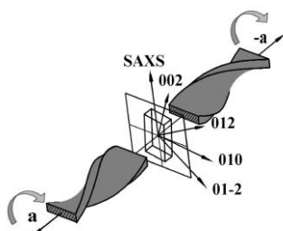
Figure III.3.12 Vector model illustrating the rotating unit cell. The axis of rotation corresponds to the crystallographic \mathbf{a} -axis. All 0kl reflexes rotate about \mathbf{a} in the plane perpendicular to \mathbf{a} . The light gray arrows indicate the rotation direction of the unit cell. The sense of twist is right for growth along the negative growth direction ( -\mathbf{a} ) while it is left for the positive direction ( \mathbf{a} ).
