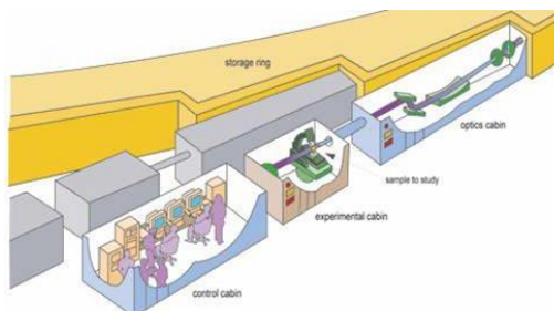
Figure II.2.4. Schematic drawing of a layout of a conventional beamline at the ESRF [52].
