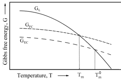
Figure I.1.2. Gibbs free energy G variation with temperature for the liquid state L (black), folded-chain FC (short dashes) and extended-chain EC (long dashes) polymer crystal.
