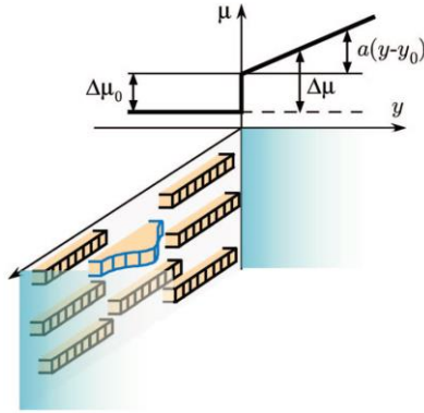
Figure 1.3.2. Cartoon depicting the gradient field spontaneously generated ahead the growth front of a stack of lamellar crystals as proposed by Mullins and Sekerka [80]. The corresponding change of the chemical potential \Delta\mu by the gradient is indicated, reprinted from [76].
