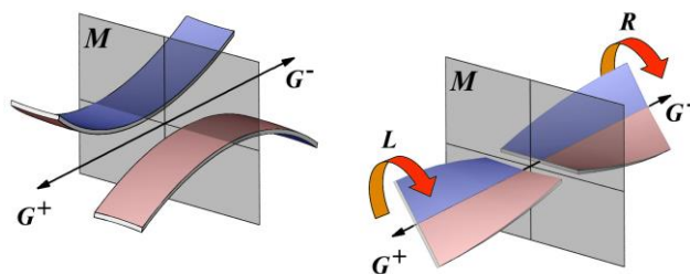
Figure I.2.8. Cartoon showing bending of two disconnected ribbons having opposite surface stresses according to the Keith and Padden model [25] ( left ). The positive surface pressure is depicted in the red overlay while the negative surface pressure is given in blue. The bending deformation keeps the mirror symmetry defined by the mirror plane M as well as point symmetry. Resulting torsional deformation of the ribbons when connected along the center line due to the unbalanced longitudinal surface stresses ( right ). The sense of deformation depends on the growth direction G . In the indicated stress distribution the positive growth direction G^+ is linked to a left-handed torque, while the negative growth direction G^- is linked to a right-handed torque keeping the symmetry operations discussed above.
