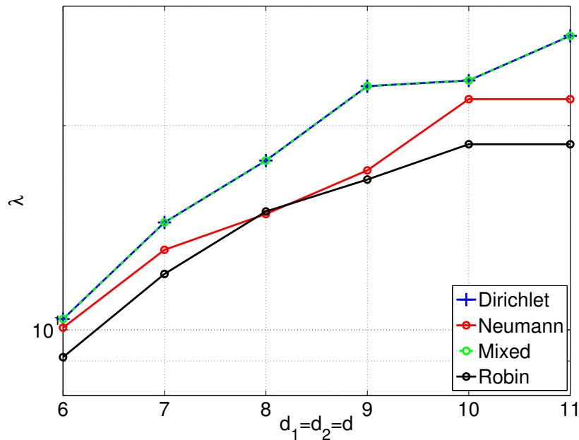
Figure 7.2. Maximum \lambda as a function of polynomial degree d_1 = d_2 = d for which the conditions of Theorem 7.5 are feasible, thereby implying the existence of an exponentially stabilizing output feedback controller for Equation (7.57).
