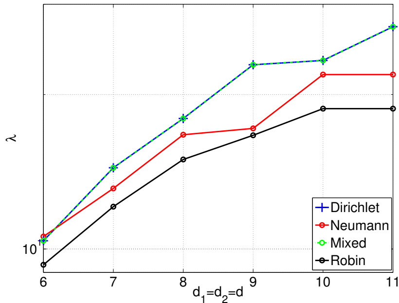
Figure 6.1. Maximum \lambda as a function of polynomial degree d_1 = d_2 = d for which the conditions of Theorem 6.4 are feasible, thereby implying the existence of an exponentially stabilizing controller for Equation (6.15).
