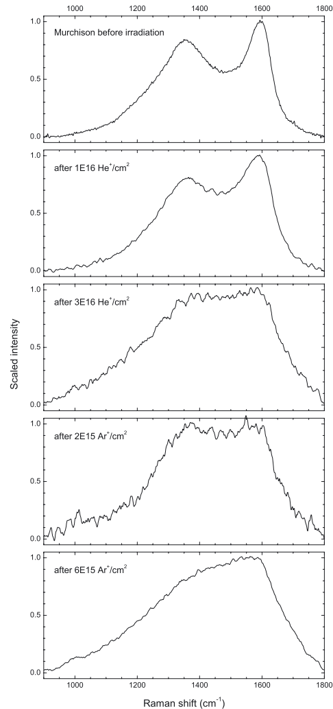
Fig. 6. Raman spectra of the unirradiated area ( top ) and for irradiated areas with 1 \times 10^{16} and 3 \times 10^{16} \text{ He}^+ , 2 \times 10^{15} and 6 \times 10^{15} \text{ Ar}^+ ( from top to bottom ) ions/ \text{cm}^2 .
