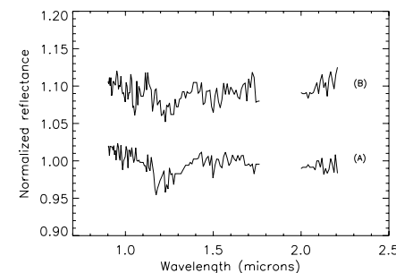
Fig. 2. NIR spectra of Ceres, shifted by 0.1 in reflectance for clarity. Regions affected by strong atmospheric absorption have been cut out.
