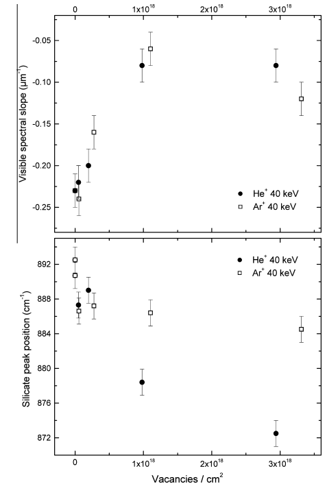
Fig. 8. Evolution of the visible spectral slope (top) and of the main IR olivine band peak position (bottom) as a function of the number of vacancies per cm 2 produced by He + and Ar + beams in the Allende target. Following the method by Lazzarin et al. (2006), the slope is evaluated by a linear fit in the 0.52–0.92 μm range of the reflectance spectra scaled to unity at 0.55 μm.
