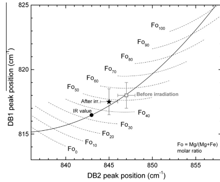
Fig. A5. The peak position of the \sim 820 \text{ cm}^{-1} olivine band (DB1) is reported as a function of the \sim 850 \text{ cm}^{-1} band position (DB2); we show the average composition we observed for unirradiated Allende along with the composition for one irradiated area ( 3\text{E}16 \text{ He}^+ /cm ^2 ); we overlaid the calibration curves extracted from Kuebler et al. (2006) and a point showing the composition obtained by IR after the same irradiation.
