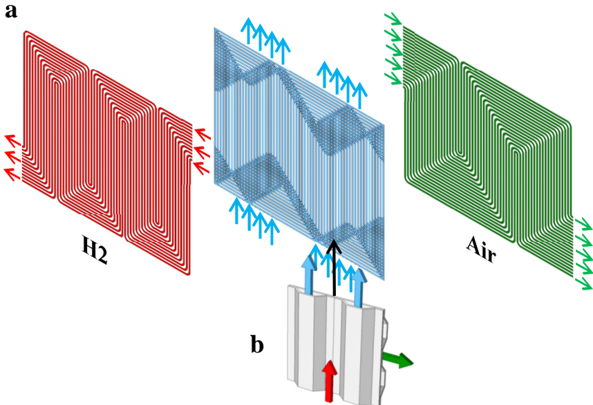
Figure II.3: (a) Presentation of the hydrogen, cooling water and air flow field designs (b) Zoom of the BP geometry in a cross-flow zone
