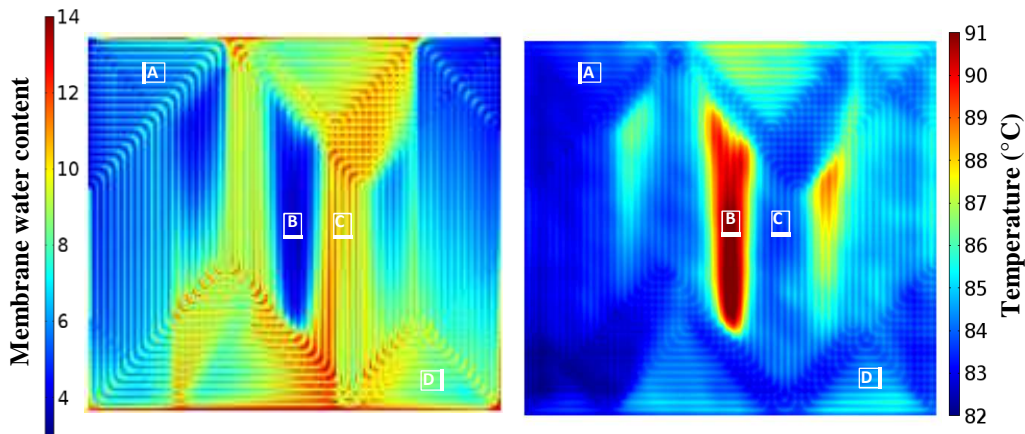
Different cut zones superposed on water content and temperature distribution simulated over the membrane surface
