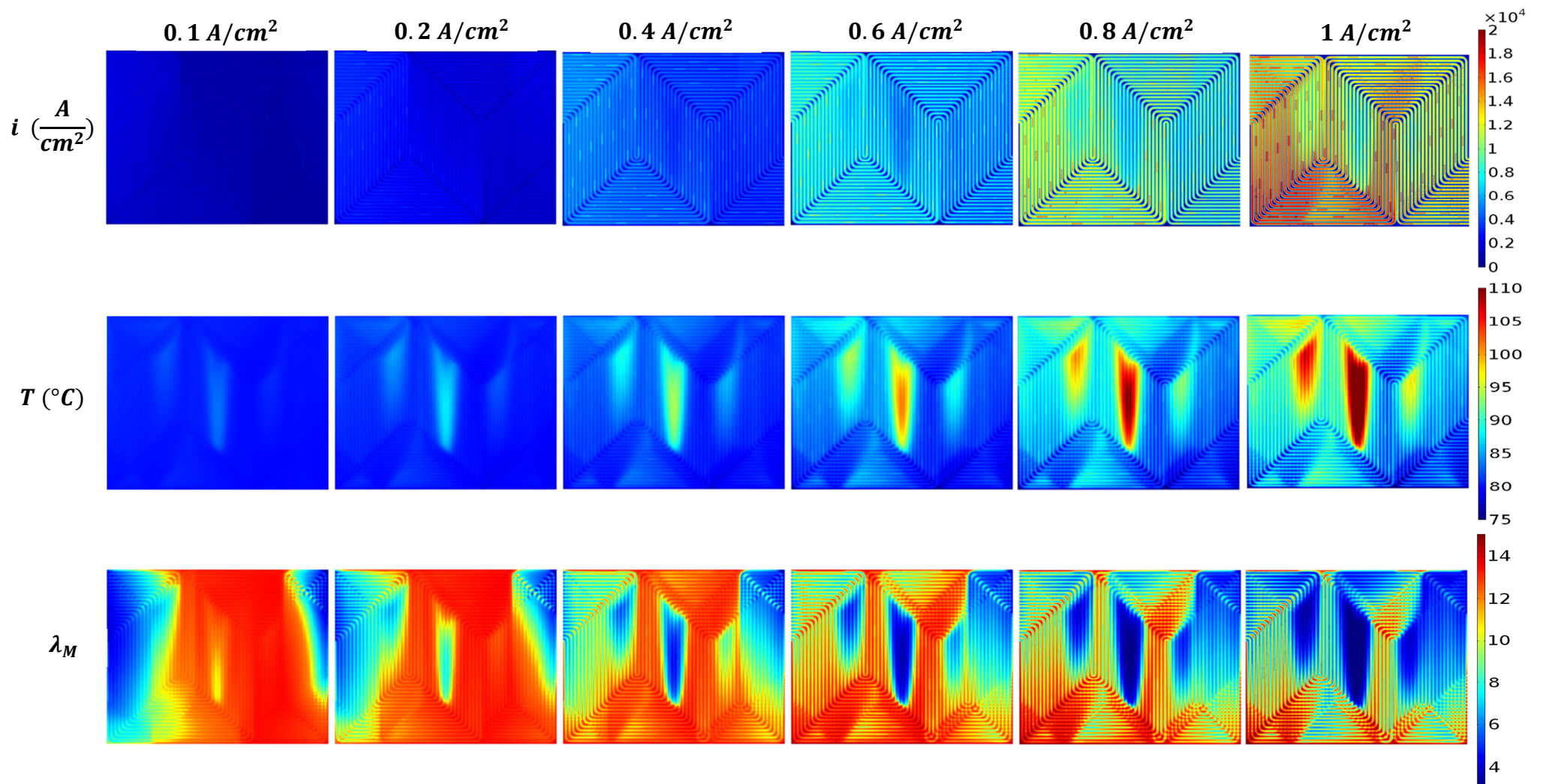
Figure IV.14 : Current density, temperature and water content in the membrane at the different operating currents
