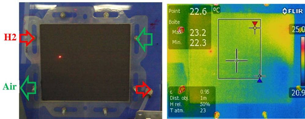
Figure V.12 : a) Aged MEA in the hydrogen box for the IR camera test (b) Infrared image of the aged MEA
