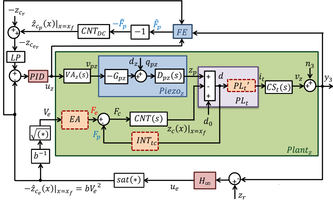
Figure 7.12: Closed-loop control of the vertical subsystem. The tunneling gap d = z_t - z_c(x_f) = d_0 + z_p - z_c(x_f) is regulated by the \mathcal{H}_\infty controller via cantilever position z_c(x_f) = z_{c_p}(x_f) + z_{c_e}(x_f) by keeping the tunneling voltage y_3 (and as a result the tunneling gap) on the constant level of z_r . The interaction (proximity) force F_p between the tip and the cantilever is estimated via FE subsystem from the tunneling voltage y_3 and the control signals u_z and u_e and eliminated by adjusting the position of the tunneling tip z_p via outer closed-loop with PID controller, tuned automatically using Matlab & Simulink software.
