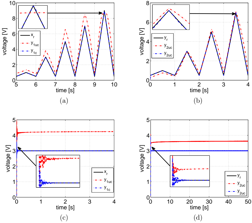
Figure 3.13: Reference tracking using observer-based approach for X (left) and Y (right) directions: (a), (b) Triangle of variable amplitude. (c), (d) Step response.
