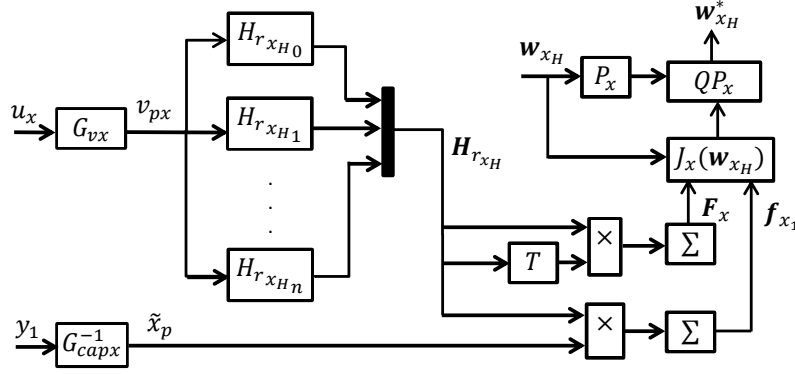
Figure 3.3: Identification procedure for X direction (PI approach).
