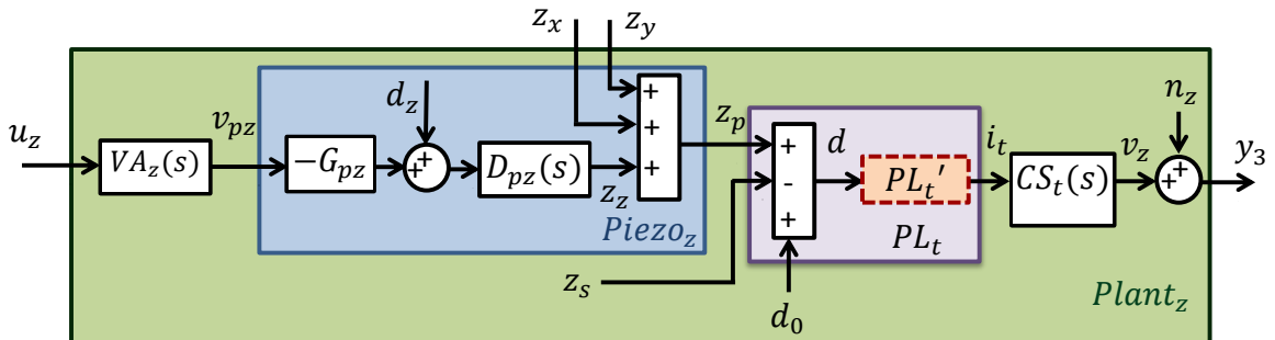
Figure 5.1: Block scheme of nonlinear plant in vertical Z direction.
