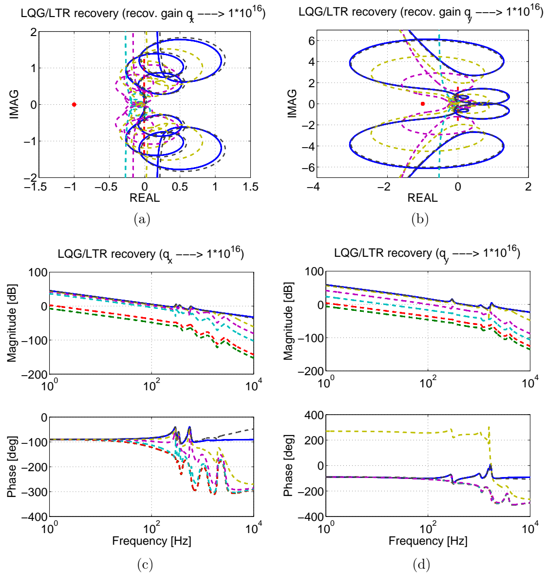
Figure 4.9: LTR with increasing recovery gain q_i = [1, 10, 10^2, 10^6, 10^8, 10^{10}, 10^{16}] ( LTF_{P_{2_i}}(s) is in dashed line from green to black, the desired LTF_{P_{1_i}}(s) is in solid blue line): a) Nyquist plot for i = x . b) Nyquist plot for i = y . c) Bode plot for i = x . d) Bode plot for i = y .
