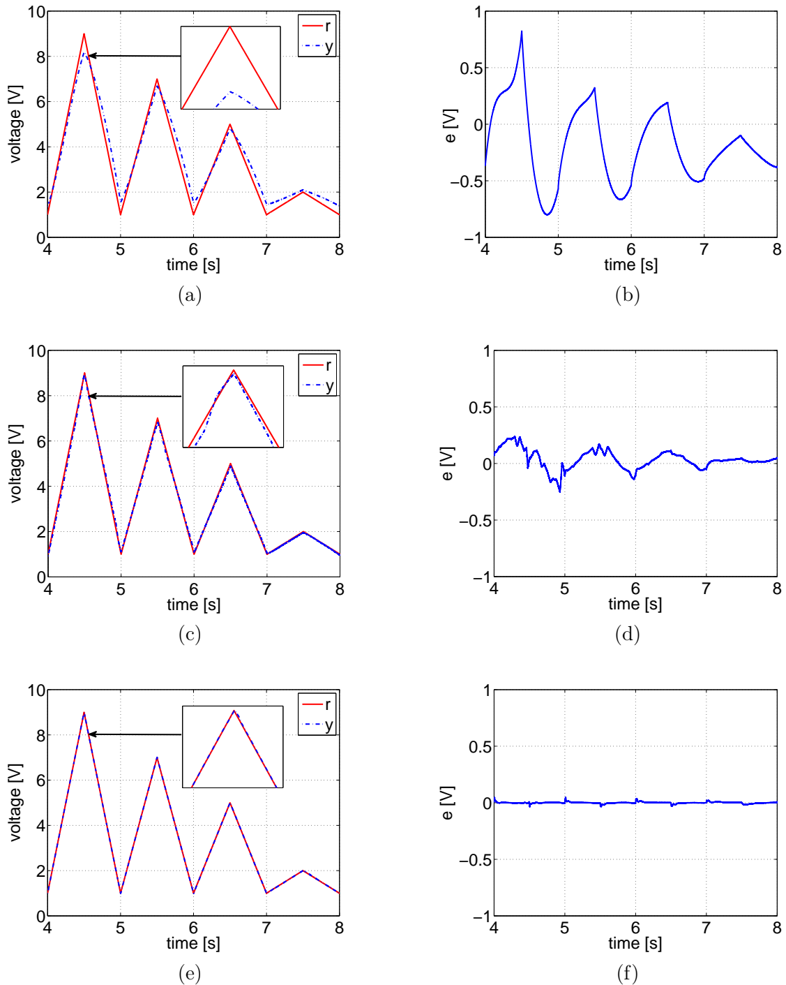
Figure 3.23: Experimental results for tracking triangular reference of variable amplitude: (a), (c), (e) Without any compensation, with MPI and with the proposed adaptive compensator, respectively. (b), (d), (f) Corresponding tracking errors.
