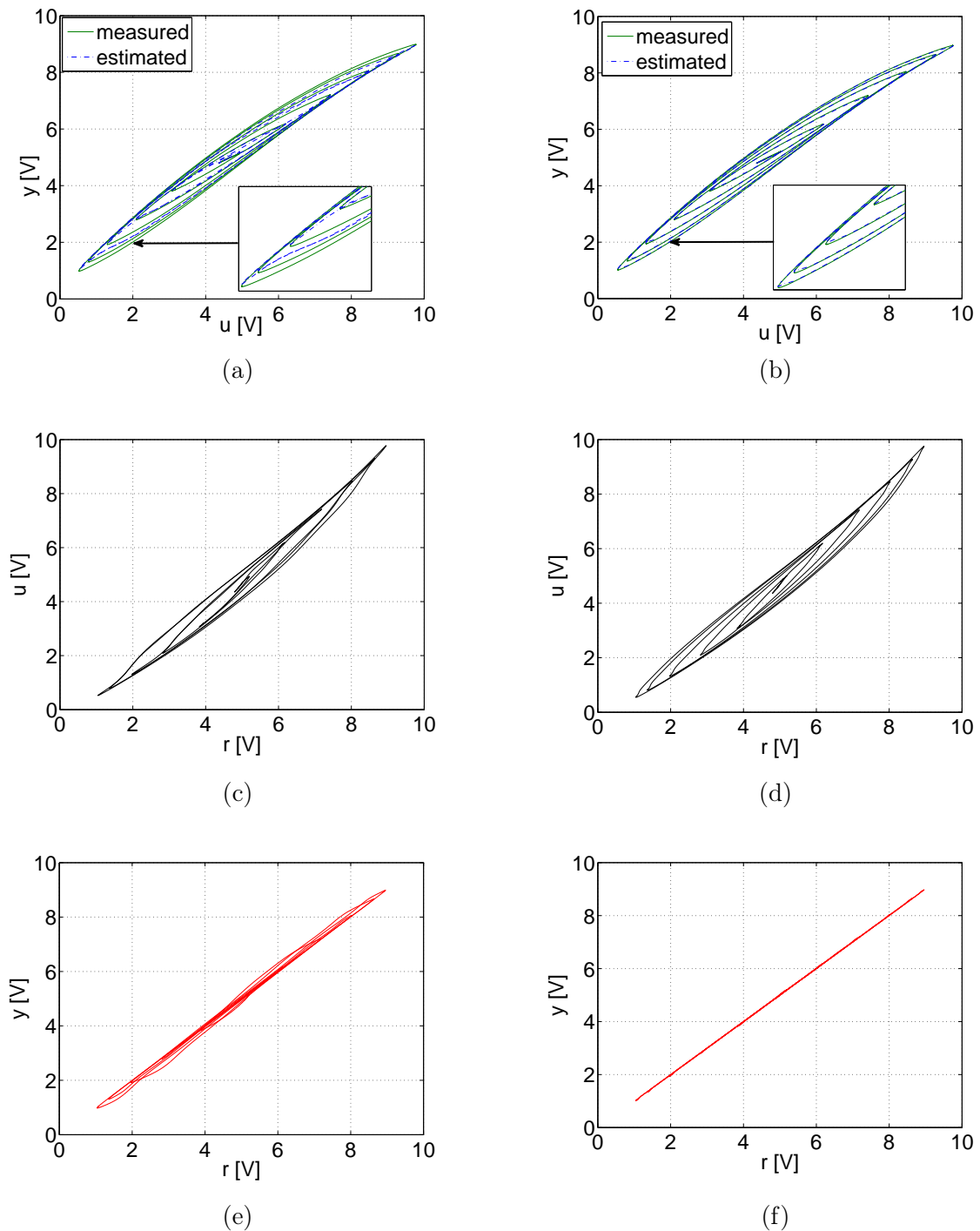
Figure 3.21: Experimental results of hysteresis compensation for sinusoidal reference of variable amplitude x_r(t) = 5 + 2\sin(2\pi t) + 2\sin(2\pi 1.2t + \pi) for \rho = 0.4 (left) and \rho = 0.8 (right): (a), (b) Measured and estimated hysteresis. (c), (d) Inverted model. (e), (f) Compensation.
