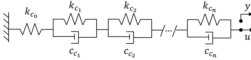
Figure 1.6: Viscoelastic creep model [Croft et al., 2001].
