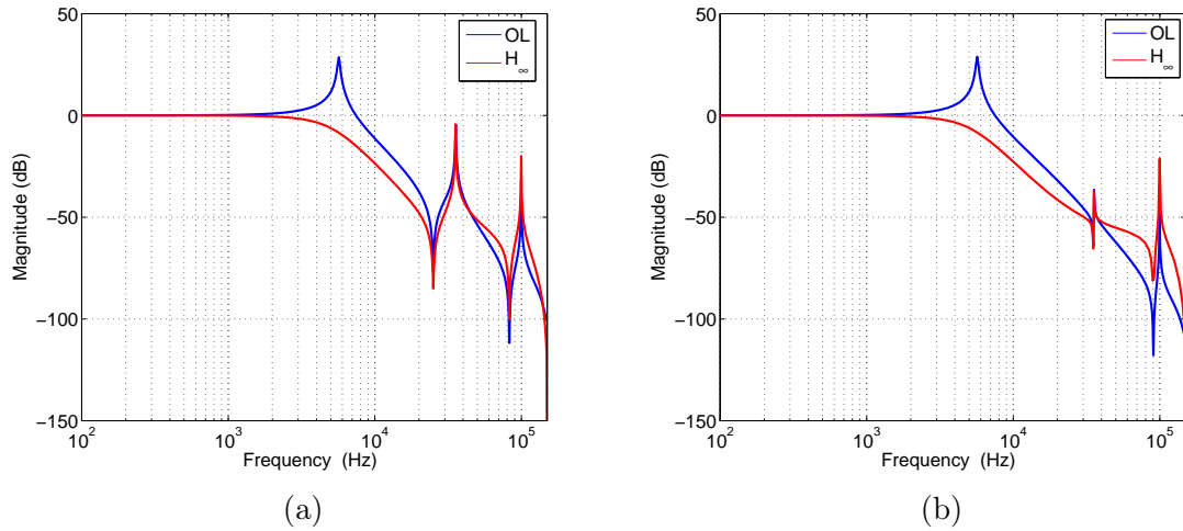
Figure 7.17: Bode diagrams of the scaled open-loop (OL) and closed-loop system with H_\infty controller (with 5 th order weight W_\Delta(s) ) and the perturbed plant model: (a) x = x_f = L = 500 \mu\text{m} . (b) x = x_f = 0.81L = 405 \mu\text{m} .
