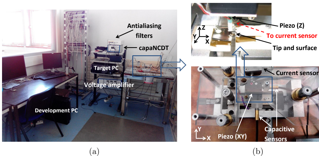
Figure 2.2: Experimental setup of 3D nanomanipulation platform: (a) General view. (b) The heart of the platform.
