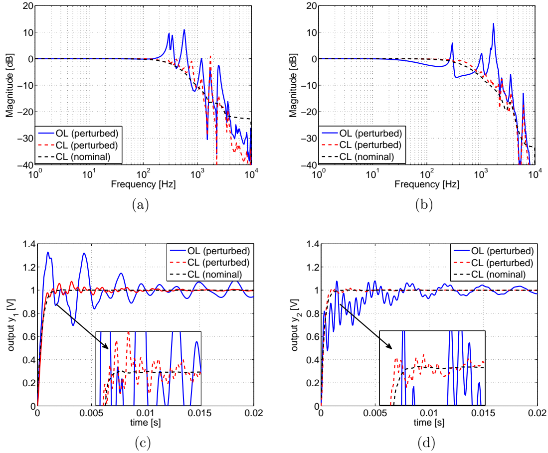
Figure 4.14: Performance of SISO H_\infty controllers: a), b) Magnitude response of the system in open-loop and closed-loop (with real and nominal system) for X and Y axis, respectively. c), d) Step response of the system in open-loop and closed-loop (with real and nominal system) for X and Y axis, respectively.
