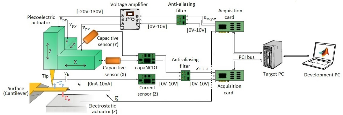
Figure 2.1: Schema of the experimental setup.
