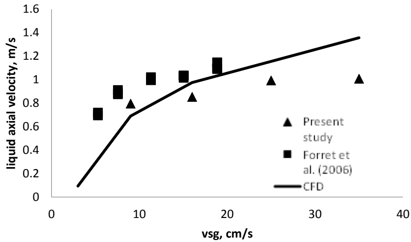
Figure 5.19 : Comparison between experimental liquid axial velocity on the column axis and CFD simulations, with the drag law of Tomiyama and the modified Simmonet swarm factor, Phi 1000 column in the range of v_{sg} [3-35 cm/s].
