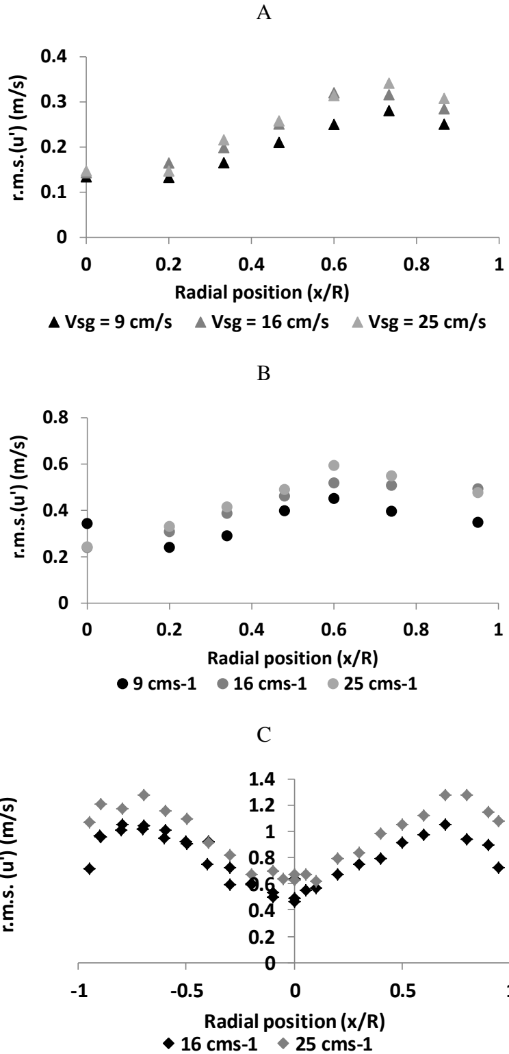
Figure 4.41 – Radial profiles of the axial liquid velocity r.m.s.(u') for several superficial gas velocities in the columns: A) Phi 150 ( h/D=2.5 ); B) Phi 400 ( h/D=2.5 ) C) Phi 3000 ( h/D=1.5 ) (measurements obtained using the 8Hz bandwidth pressure sensors)
