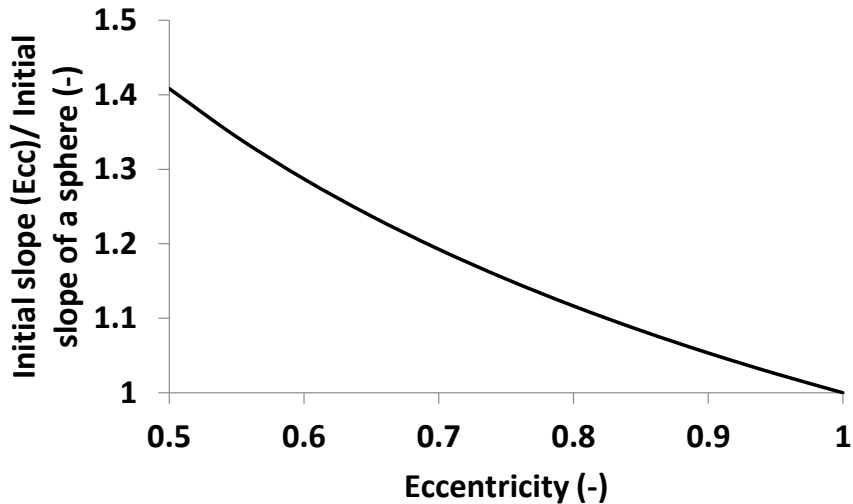
Figure 3.24 – Evolution of the ratio “Initial slope (Ecc)/Initial slope of a sphere” with the eccentricity for prolate shaped bubbles.
