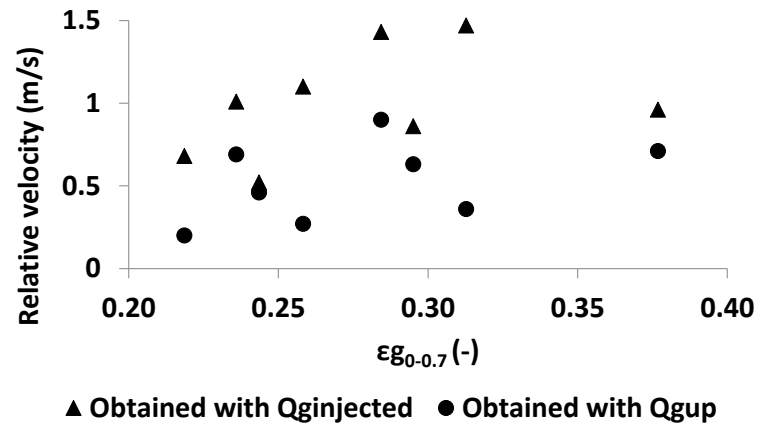
Figure 4.55 – Evolution of the relative velocity with \varepsilon g_{0.7} for the columns Phi 150, Phi 400 and Phi 1000. (Calculated by Eq. (4.16))
