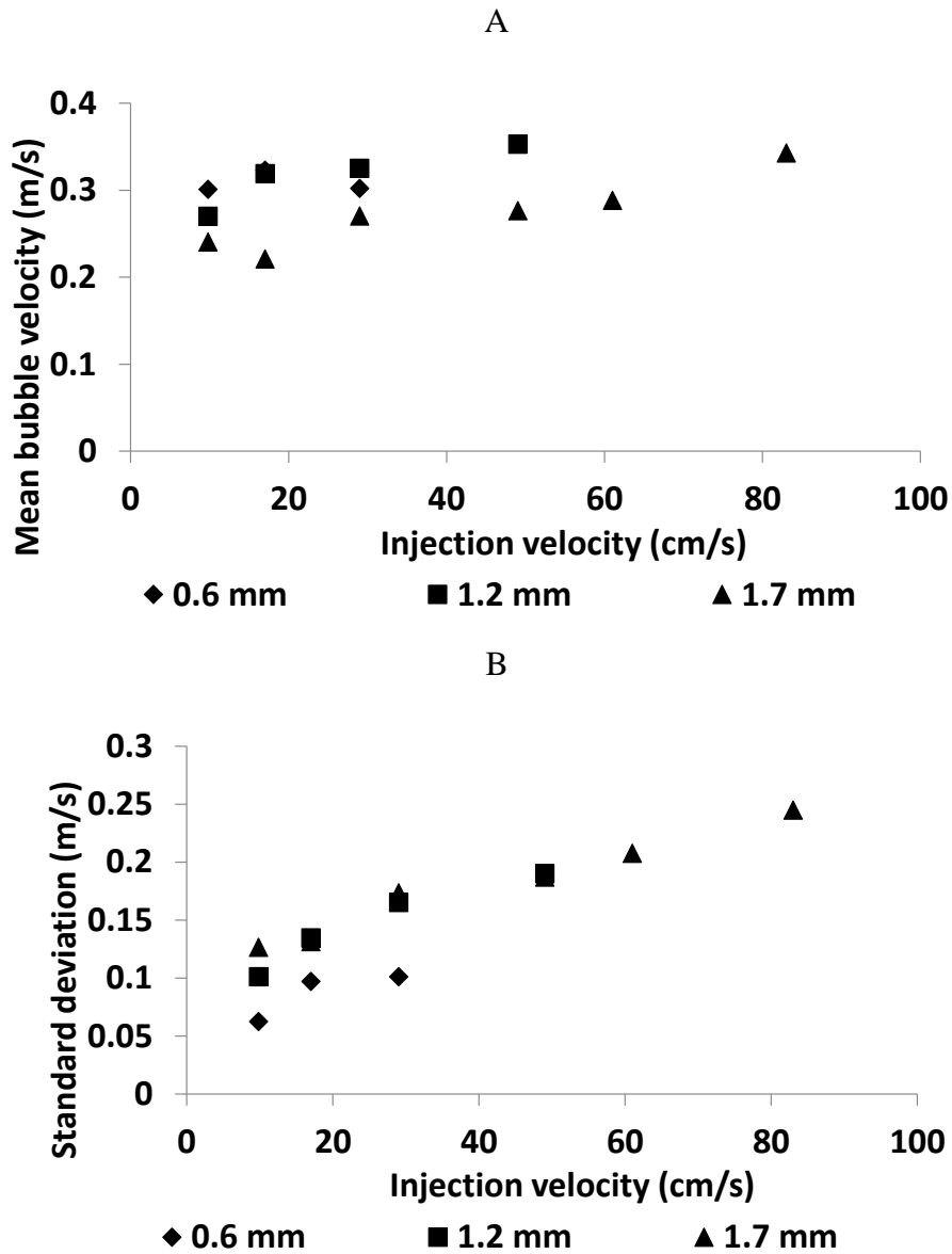
Figure 2.7 - A) Evolution of bubbles mean velocity with gas injection velocity B) Evolution of the standard deviation of the bubble velocity distribution with gas injection velocity. Measurements for several injector with internal diameters ranging from 0.6 mm to 1.7mm, measurements at an elevation of 0.16m from the injector.
