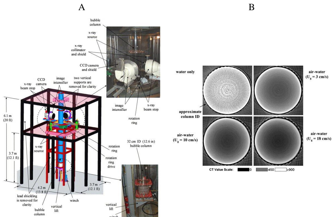
Figure 1.30 – A) A schematic representation of X-ray tomography system. B) Hold up cross-section profiles measured by of X-ray tomography (Hubers, 2005)
