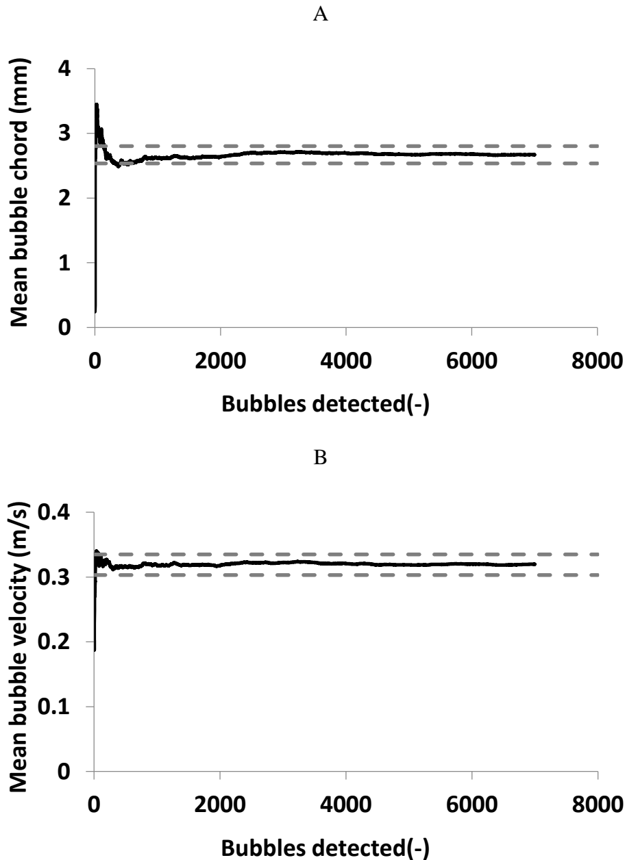
Figure 2.2 – Convergence of the cumulative average of: A) bubble chord B) bubble velocity. (Dashed lines- \pm 5\% convergence)(I.d. injector =1.2 mm at 0.16 m from the injector and V_i=17 m/s)
