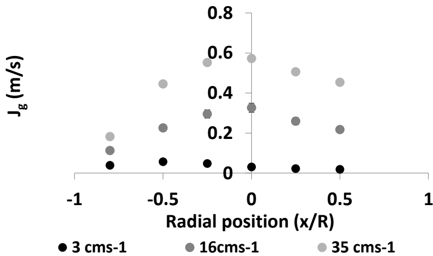
Figure 3.54 – Evolution of the local gas flux measured by the optical probe along the column radius. (Measurements performed in the Phi 400 column at h/D=2.5 )
