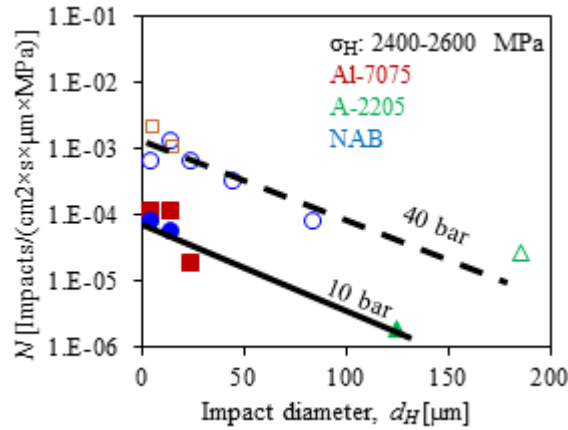
Fig. 3.12 Normalized impact frequency, N (Number of impacts/cm 2 /sec/ \mu\text{m} /MPa) plotted as a function of the impact diameter d_H for the hydrodynamic impact loads estimated at 10 and 40 bar. N is estimated at different ranges in the values of d_H (with a band width of 10 \mu\text{m} ) for a given range of \sigma_H = 2400\text{-}2600 MPa. The vertical axis is on log-scale. Nanoindentation material properties extrapolated at strain rate 10^6 \text{ s}^{-1} were used for FE simulations in the inverse method.
