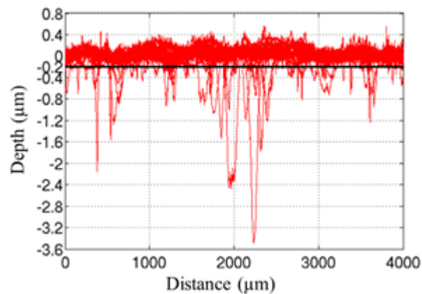
Fig. 2.15 Twenty profiles along different lines on the pitting tested surface are plotted together. Maximum noise level is approximately -0.2\ \mu\text{m} as shown by black the line. Al-7075 material cavitation tested at flow pressure of 40 bar for 2 sec.
