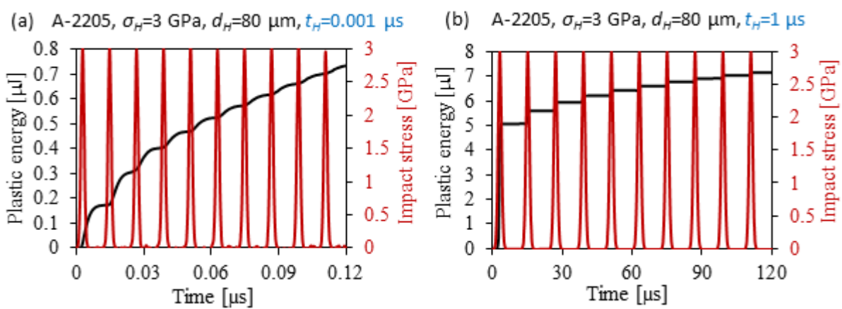
Fig. 5.11 Effect of cavitation impact duration on strain accumulation is shown for A-2205, \sigma_H = 3 \text{ GPa} , d_H = 80 \text{ }\mu\text{m} , (a) t_H = 0.001 \text{ }\mu\text{s} and (b) t_H = 1 \text{ }\mu\text{s} .
