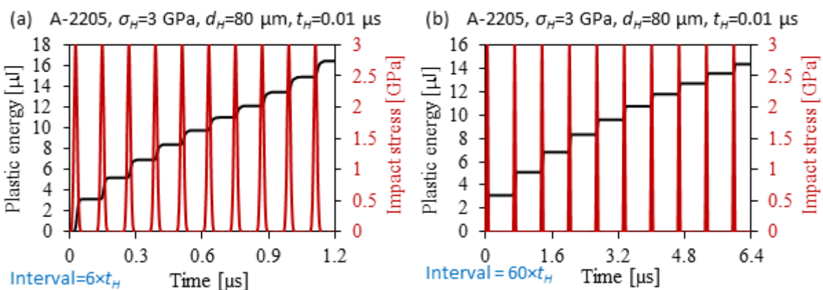
Fig. 5.12 Effect of interval between cavitation impacts on strain accumulation is shown for A-2205, \sigma_H = 3 \text{ GPa} , d_H = 80 \text{ }\mu\text{m} , t_H = 0.01 \text{ }\mu\text{s} and (a) interval = 6 \times t_H and (b) interval = 60 \times t_H .
