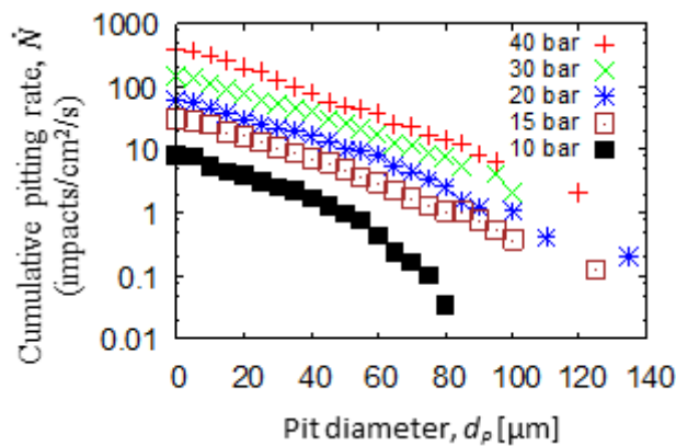
Fig. 2.25 Cumulative pitting rate of Al 7075 material as a function of pit diameter for different values of upstream pressure and constant cavitation number. Pit detected by using a constant cut-off depth of 0.5 \mu\text{m} and diameter measured at fractional cut-off depth of 50.0%. Straight lines on semi-log plot represent exponential distribution.
