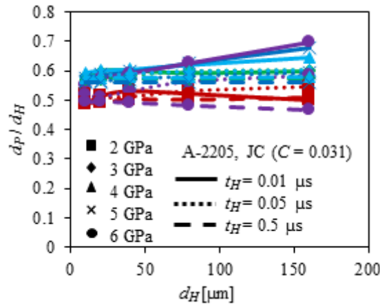
Fig. 4.15 Ratio of pit diameter to impact diameter ( d_p/d_H ) as a function of impact diameter d_H for different values of \sigma_H (2-6 GPa) and t_H = 0.01, 0.05 & 0.5 \mu s . Each line joins the iso- \sigma_H data points where different line types indicate different values of t_H and different point types indicate different \sigma_H .
