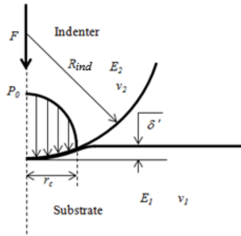
Fig. 2.2 Hertzian type of elastic contact of a spherical indenter with flat surface
