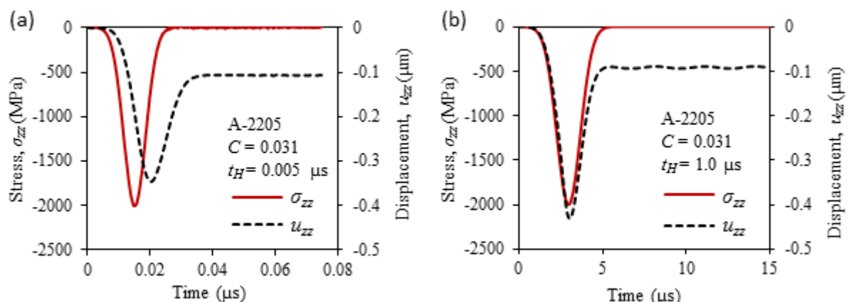
Fig. 4.2 Represents evolution of applied stress ( \sigma_{zz} ) and deformation depth ( u_{zz} ) with time during hydrodynamic impact. Material: A-2205, \sigma_H = 2 GPa and d_H = 40 \mu\text{m} (a) t_H = 0.005 \mu\text{s} (b) t_H = 1.0 \mu\text{s} .
