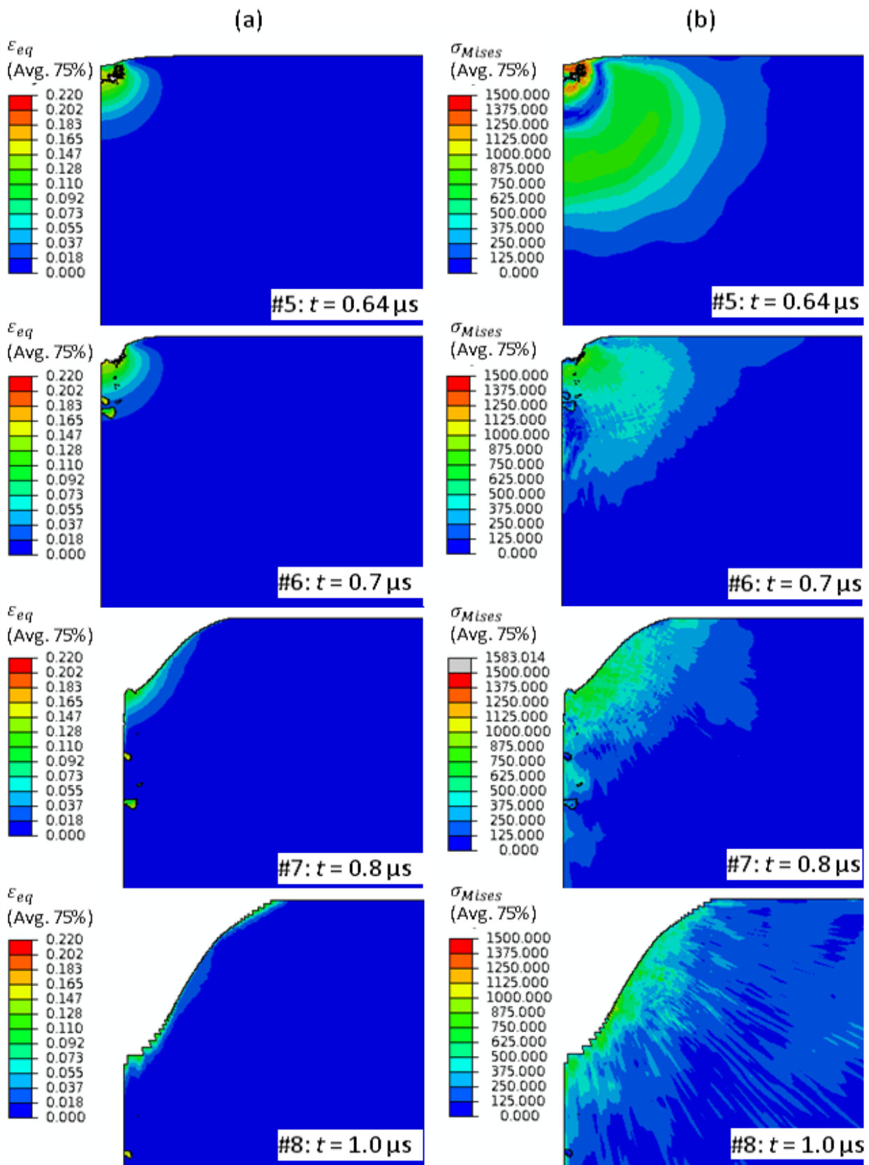
Fig. 5.14 Simulation of cavitation erosion. Multiple impacts of the same impact load ( \sigma_H = 4 \text{ GPa} , d_H = 80 \mu\text{m} and t_H = 0.01 \mu\text{s} ) on the same location shows fatigue behavior of cavitation that lead to strain accumulation and damage in A-2205 material. Frames (#1-#8) on the left show plastic strain accumulation with time, whereas the corresponding equivalent stresses are shown in frames on the right. The debris on the figures are the damaged materials.
