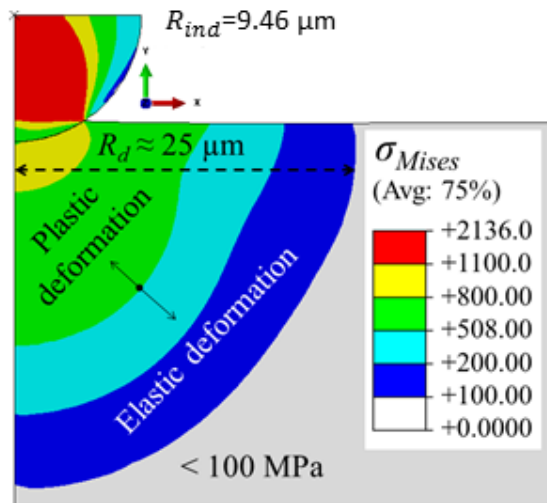
Fig. 3.15 Nanoindentation simulation of A-2205 with a spherical diamond indenter of radius R_{ind}=9.46 \mu\text{m} . Distribution of von Mises equivalent stress ( \sigma_{Mises} ) is shown highlighting the extent of effectively deformed region beneath the indenter.
