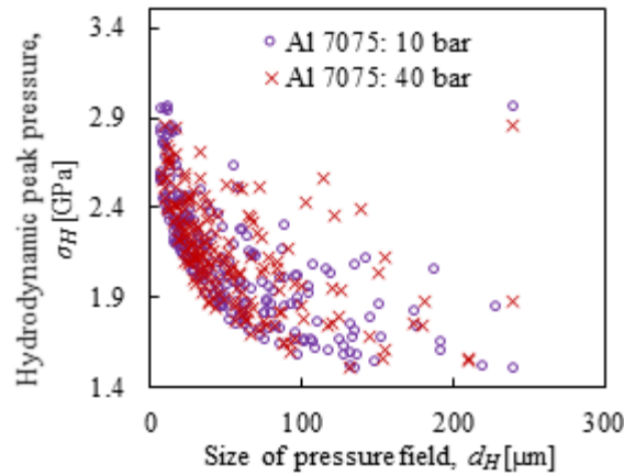
Fig. 2.22 Distribution of peak hydrodynamic pressures and corresponding sizes of pressure field associated with bubbles formed at different flow pressures, 10 bar and 40 bar.
