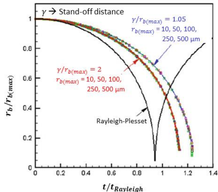
Fig. 6.1 Comparison of the time history of the normalized bubble equivalent radius for initial bubble maximum radii of 10, 50, 100, 250 and 500 \mu\text{m} at \gamma/r_{b(\text{max})} = 1.05 (blue line) and \gamma/r_{b(\text{max})} = 2.0 (red line). All the bubbles have an initial gas pressure of 1 atm ( \sim 1.01 bar) and are subjected to an ambient pressure of 34.5 atm ( \sim 34.95 bar) to simulate the bubble collapse. The bubble equivalent radius is normalized by r_{b(\text{max})} while the time scale is normalized by the Rayleigh time [81].
