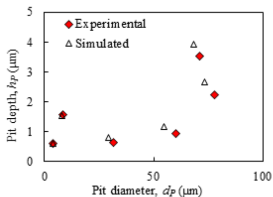
Fig. 2.11 Comparison of experimental pit depth and diameter with that of simulated. Input parameters for simulation \sigma_H and r_H were predicted using analytical method (Eq. (2.9) and Eq. (2.10)).
