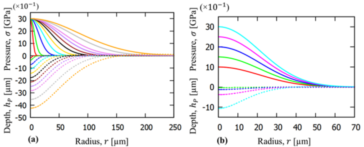
Fig. 2.7 Applied Gaussian loads and corresponding unloaded deformed geometry represent simulated pit shape. (a) At \sigma_H = 3 GPa for r_H = 5 to 120 \mu\text{m} and (b) At r_H = 30 \mu\text{m} for \sigma_H = 1 to 3 GPa, no pit formed at 1 GPa.
