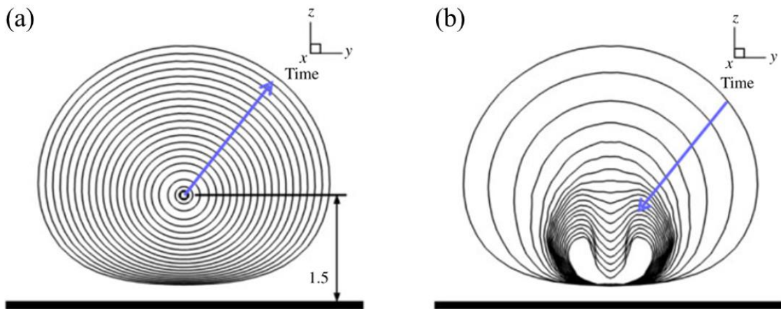
Fig. 1.3 Evolution of bubble shape with time showing (a) bubble growth and (b) bubble collapse. The arrow indicate increase in time. 3D boundary element method (BEM) simulation of initial nuclei of 50 \mu\text{m} at a distance of 1.5 mm undergoes a pressure difference of 10 MPa in a period of 2.415 ms. Standoff distance at maximum bubble radius is 0.75 [28].
