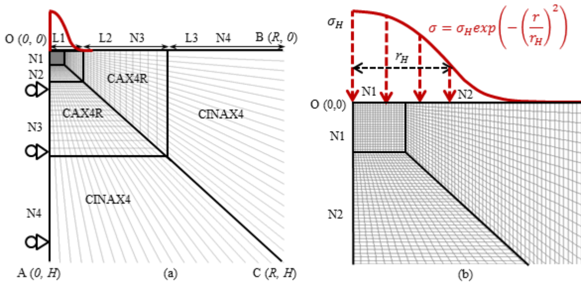
Fig. 2.1 (a) 2-D axisymmetric mesh used for numerical simulation. L represents length of one or more section as shown by arrow. N represents number of elements on the surface of different section. Number of elements ( N1 , N2 , N3 and N4 ) in different section is always constant, but section lengths ( L1 , L2 and L3 ) are parameterized from radius of hydrodynamic pressure field, r_H , e.g. if r_H = 10 \mu\text{m} , N1 = 20 , N2 = 60 , N3 = 40 and N4 = 1 then, L1 = 1.5 \times r_H = 15 \mu\text{m} , L1+L2 = L3 = R/2 = 8 \times L1 = 120 \mu\text{m} , H = R = 240 \mu\text{m} using geometric progression with common ratio of 1.01. (b) Shows magnified view of the loading region. Minimum element size is 0.123 \mu\text{m} for r_H = 10 \mu\text{m} .
