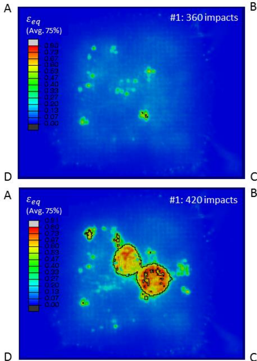
Fig. 5.18 Cavitation erosion simulation on A-2205 material. Characteristic impact duration t_H = 0.01 \mu\text{s} and t_{max} = 3 \times t_H are assumed. Mass-loss started after 360 impacts at some locations. The plastic strain at the damage initiation and failure is defined as 80% and 90% respectively, along with a linear evolution. This choice is arbitrary. As the mesh is coarse (minimum size is 3.33 \mu\text{m} ) compared to the smaller impact diameters of 5 or 10 \mu\text{m} , a higher value of strain was required to use to avoid numerical problems. Only the region ABCD on of the mesh is shown here. As can be seen, the regions from where the material has been removed is surrounded by black lines.
