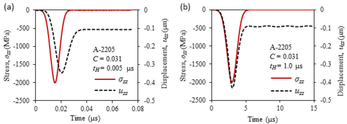
Fig. 4.2 Represents evolution of applied stress ( \sigma_{zz} ) and deformation depth ( u_{zz} ) with time during hydrodynamic impact. Material: A-2205, \sigma_H = 2 GPa and d_H = 40 \mu m (a) t_H = 0.005 \mu s (b) t_H = 1.0 \mu s .
