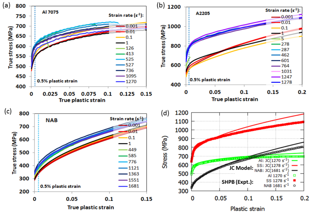
Figure A.4 (a)-(c) Stress-strain curves obtained by SHPB tests are plotted together along with compression tests curves. Stress-strain curves at strain rates < 10 s^{-1} are obtained by servo-hydraulic compression testing machine, whereas curves at strain rates > 100 s^{-1} are SHPB data.
