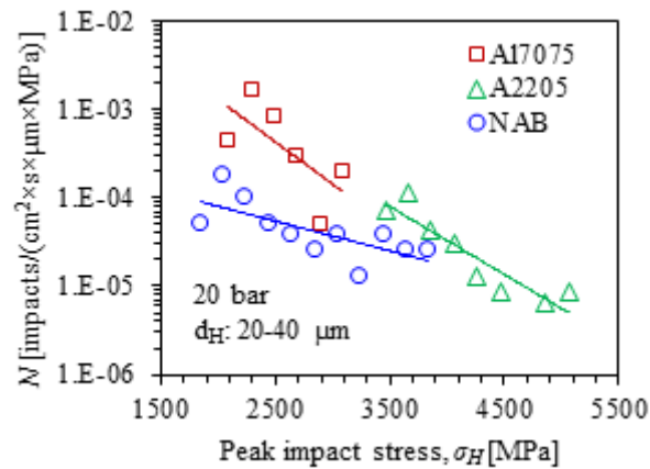
Fig. 3.10 Normalized impact frequency, N (Number of impacts/cm 2 /sec/μm/MPa) is plotted as a function of peak impact stress \sigma_H for the hydrodynamic impact loads estimated at 20 bar. N is estimated at different ranges in the values of \sigma_H (with a band width of 200 MPa) for a given range of d_H=20-40 \mu\text{m} . The vertical axis is on log-scale. Compressive material properties extrapolated at strain rate 10^6 \text{ s}^{-1} were used for FE simulations in the inverse method.
