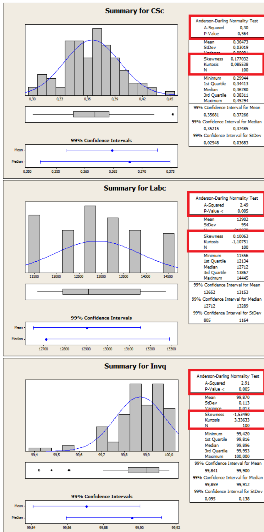
Figure 6.5: Anderson-Darling normality test for three indicators.
