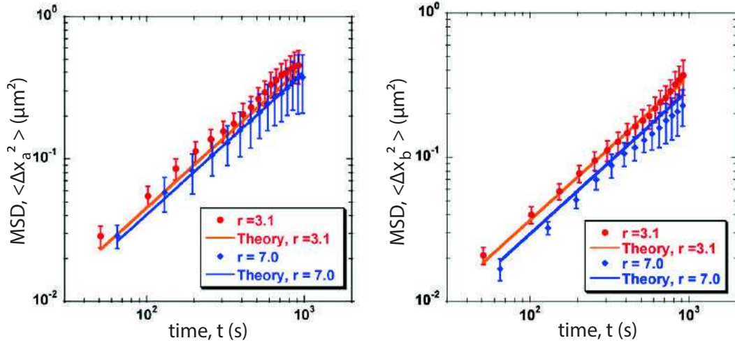
Figure 1.15: MSD vs. time lag for spheroidal particles totally immersed in a fluid, viscous phase. The displacements are here directly measured, by confocal microscopy, along the long (a) and the short (b) axes of the particle. Two aspect ratios are considered in this experience: \phi = 3.1 (red points) and \phi = 7.0 (blue points). The experimental data are compared with the theoretical predictions (solid lines), showing a strong agreement. Measurements and graphs from Mukhija et al., J Colloid Interface Sci, 314, 98106 (2007) [5].
