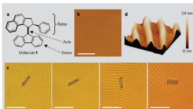
Figure 28 | a) Structure of the motor. b) Polygonal texture of a liquid-crystal film doped with motor (1 % by weight). c) Glass rod rotating on the liquid crystal during irradiation with ultraviolet light. Frames 1-4 (from left) were taken at 15-s intervals and show clockwise rotations of 28^\circ (frame 2), 141^\circ (frame 3) and 226^\circ (frame 4) of the rod relative to the position in frame 1. Scale bars, 50\ \mu\text{m} . d) Atomic force microscopy image of surface structure of the liquid-crystal film. [60]
