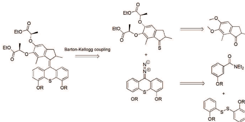
Figure 30 | Retrosynthetic analysis of the target motor
