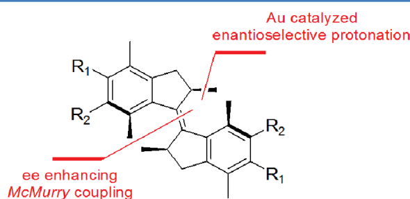
Figure 15 | Asymmetric synthesis of functionalized first generation motors. [30]
