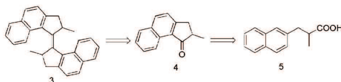
Scheme 1 | Retrosynthesis of motor 3 [27]
