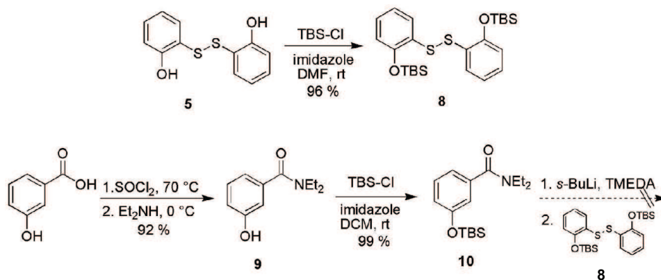
Scheme 7 | Synthesis of TBS protected lower part
