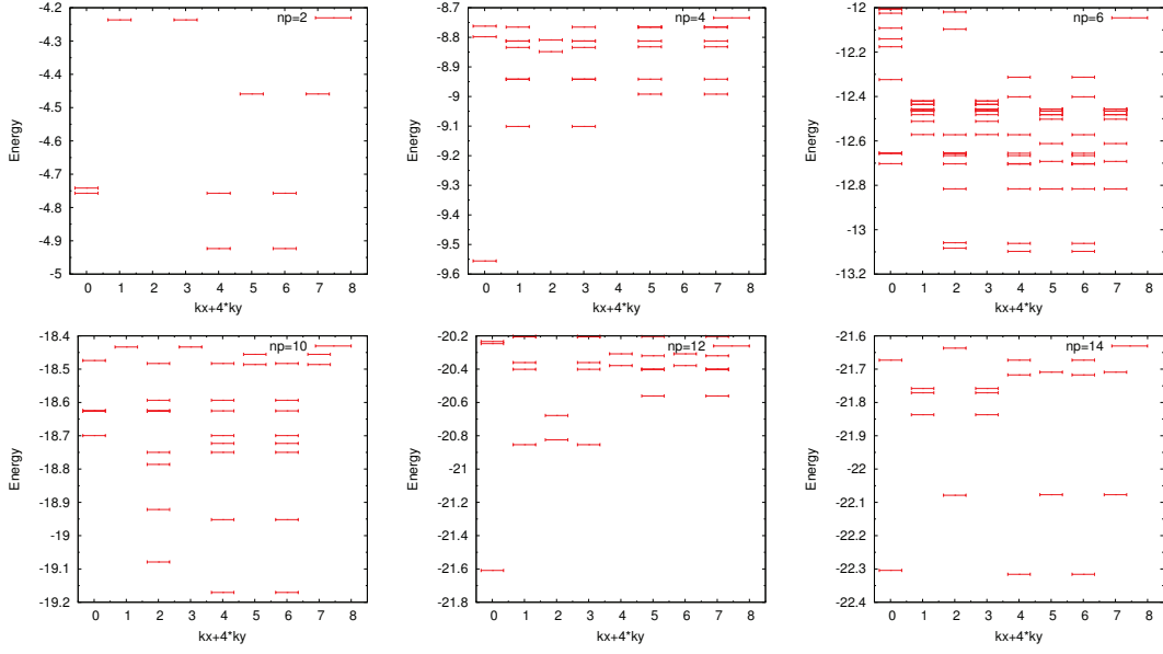
Figure 3.23: Exact diagonalization spectrum for 2, 4, 6, 10, 12 and 14 particles ( np as number of particles) on the 4 \times 2 plaquettes on torus at the pure spin-orbit coupling limit t = 0, t' = 1 .
