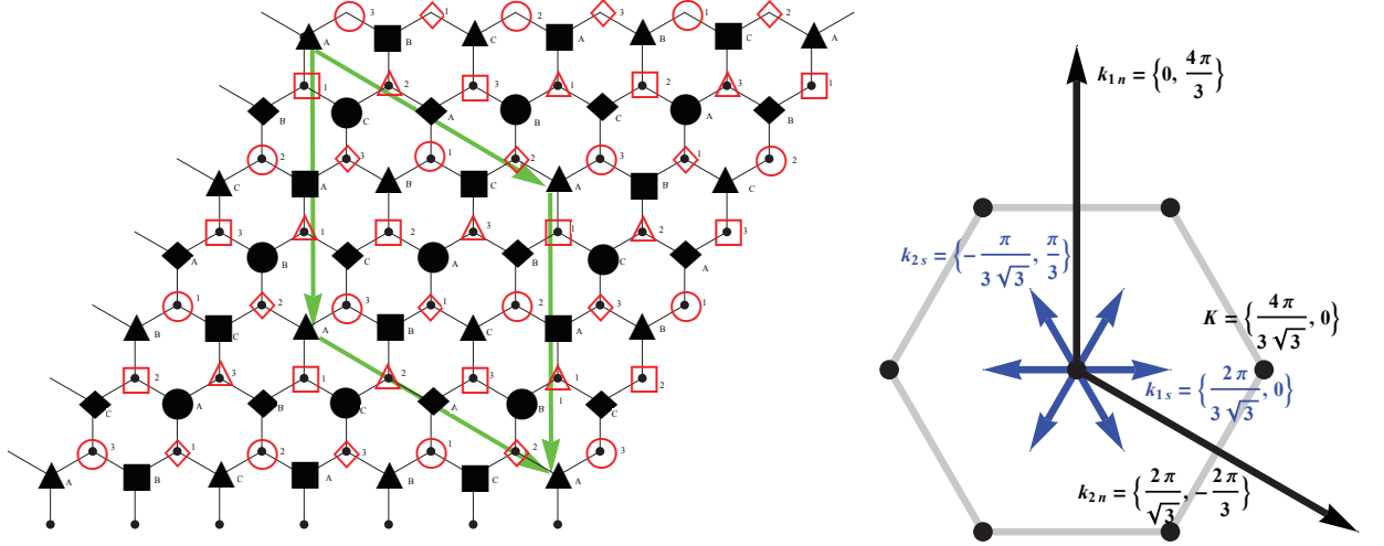
Figure 2.10: The global transformation brings the J_2 anisotropic magnetic model to an anti-ferromagnetic spin model on triangular lattices with four patterns: \square\diamond\bigcirc\triangle with black patterns on one sublattice and red patterns on the other. The nearest-neighbor J_1 Heisenberg coupling locks the angles between two copies of spiral orders and fixing the relative arrangement of the 4 patterns between the two sublattices as shown in the figure. The sites on which we studied the nearest-neighbor Heisenberg coupling namely the local fields \vec{h}_{\triangle}^1 , \vec{h}_{\square}^2 and \vec{h}_{\bigcirc}^3 in Eqs. 2.2.15, 2.2.16 and 2.2.17 are painted in red color with their number indicating the sublattice for the transformed 120^\circ Néel order. In Green, we depict the 12 sublattices (sites) on each triangular sublattice with 4 patterns, which finally constitutes 24 sublattices for the elementary cell of the magnetic order. We also represent the wave-vectors associated with the Spiral phase (in blue) and with the Néel phase (in black). The grey hexagon connects the Dirac points.
