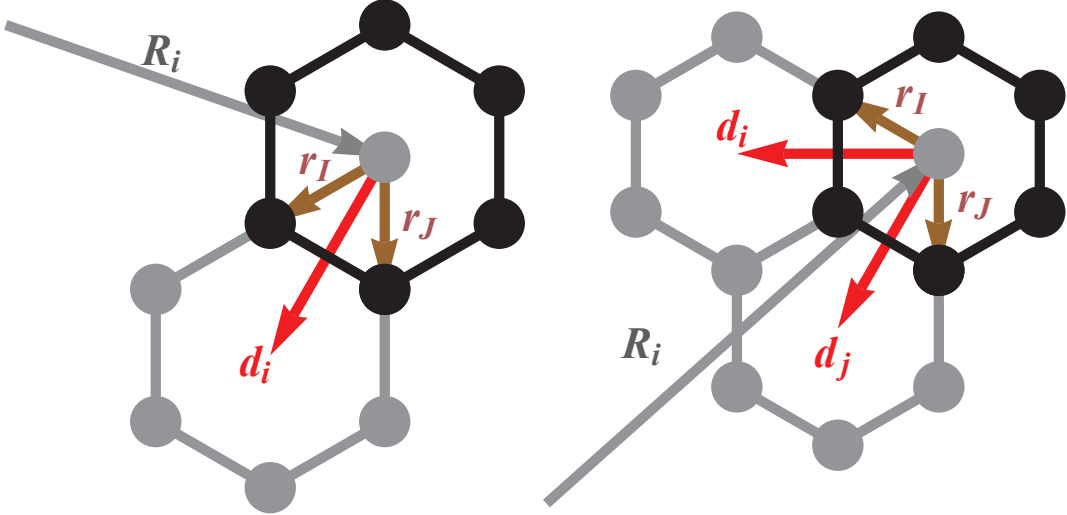
Figure 2.12: The configuration of \vec{r}_I , \vec{r}_J and \vec{R}_i related to Eq. 2.3.26, in which \vec{r}_I , \vec{r}_J are vectors connecting the plaquette centers to its vertices and |\vec{r}_I - \vec{r}_J| denotes the first neighbour link; \vec{R}_i gives the coordinates of the studied plaquette. We have to pay special attention to coordinates in Eq. 2.3.26: \vec{r}_i = \vec{r}_I + \vec{R}_i and \vec{r}_j = \vec{r}_J + \vec{R}_i . The sum over the coordinates of the studied plaquette at \vec{R}_i in Eq. (2.3.26) shall induce the momentum conservation \vec{k} - \vec{k}' = \vec{q} of the spinon excitations under the monopole insertion. The vectors \vec{d}_I and \vec{d}_J are vectors connecting the plaquettes for the configuration of gauge fields on the honeycomb lattice; see section 2.4.
