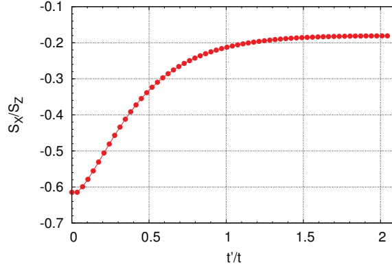
Figure 2.15: The ratio of S_x/S_z on site 1 in Fig. 2.13 as a function of t'/t . This indicates that there are two spin textures when varying t'/t : 1. The subordinate spin polarization have an opposite component as the dominant polarization S_x = S_y = -0.6S_z when t' is small compared to t ; and 2. S_z \gg (S_x, S_y) when t' > t .
