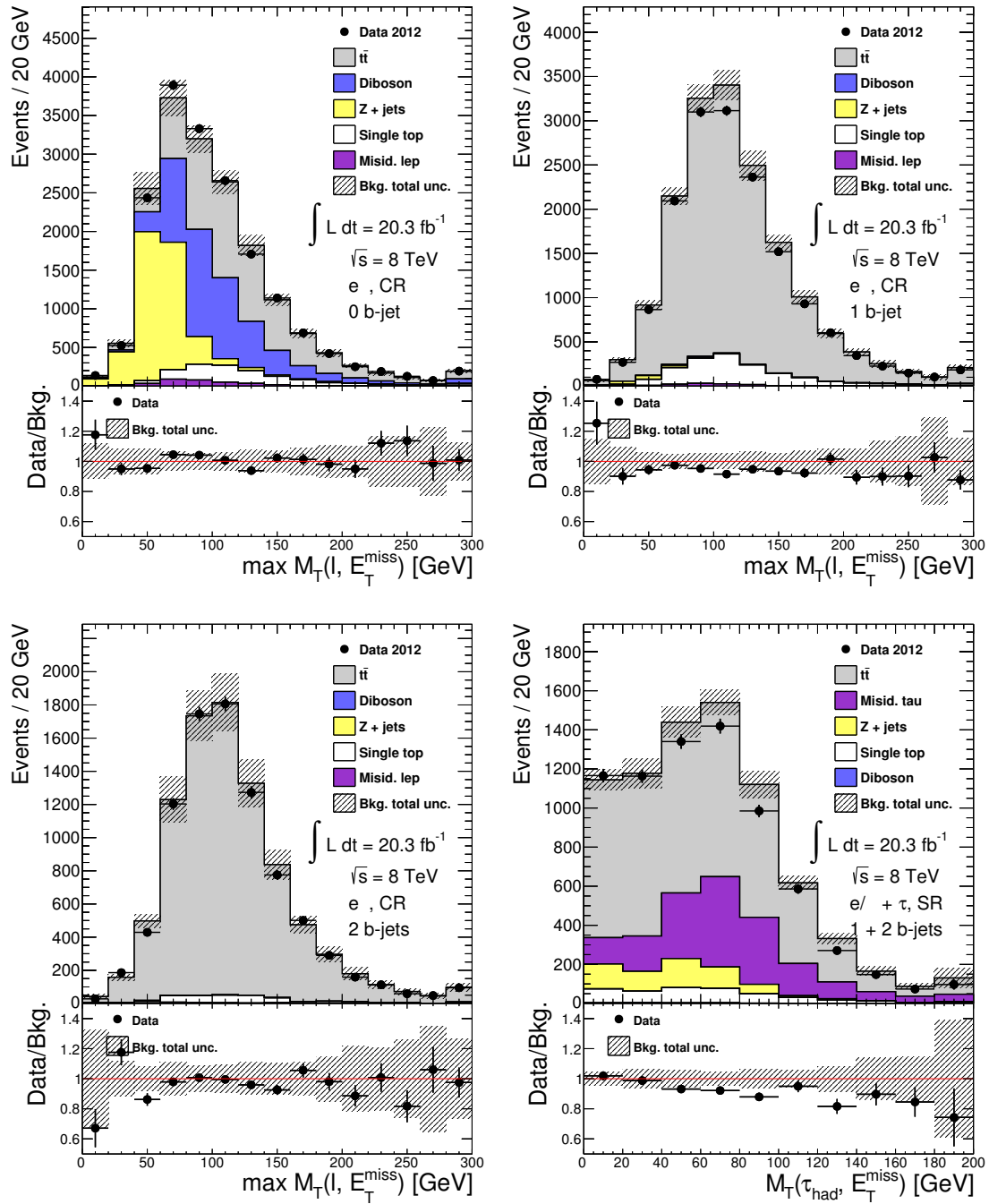
Figure 7.5. The inputs to the fit: the maximum transverse mass of dilepton events passing the CR selection with 0 b -tagged jets (top left), 1 b -tagged jet (top right), and 2 b -tagged jets (bottom left), as well as the transverse mass of lepton + \tau_{\text{had}} events passing the SR selection with one or two b -tagged jets. In all plots, the last bin includes overflow.
