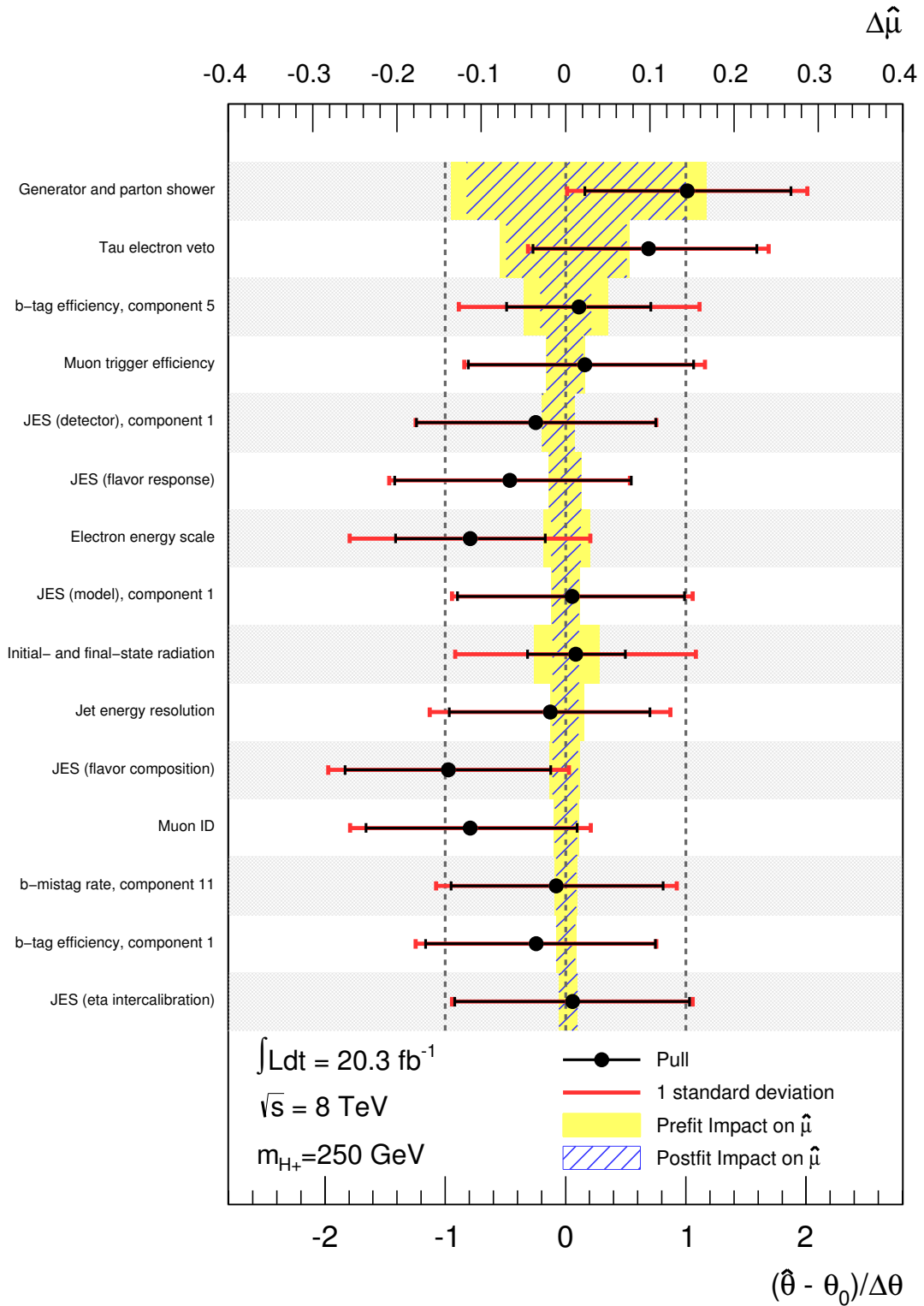
Figure 7.8. Pull distribution for the m_{H^+} = 250 \text{ GeV} hypothesis. The black markers indicate the shift of the best-fit value of each parameter with respect to its nominal value in units of one standard deviation (red) as indicated on the bottom axis, while the yellow and hatched blue bands respectively show the pre- and post-fit impacts on the fitted signal strength as indicated on the top axis. The 15 most important parameters are shown. Some of the uncertainties related to the jet energy scale (JES) or b -tagging are split into several effective components.
