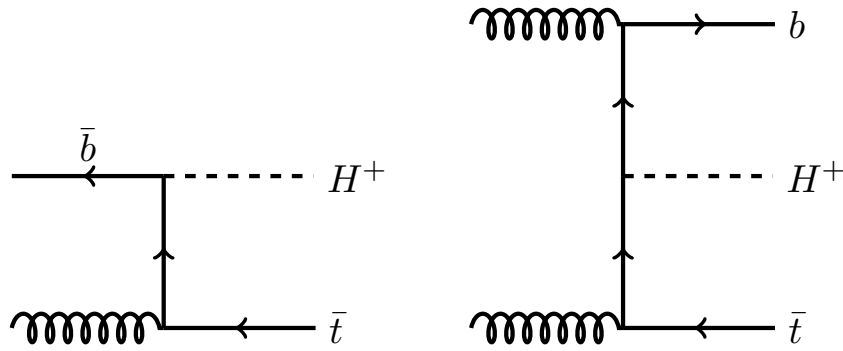
Figure 2.4. Tree-level diagrams for the production of a heavy charged Higgs boson in the 5FS (left) and 4FS (right).
