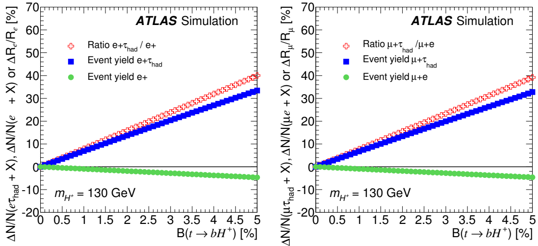
Figure 6.8. The predicted relative change of the event yields \mathcal{N}(e + \tau_{\text{had}}) and \mathcal{N}(e + \mu) , and of their ratio R_e (left) and the predicted relative change of the event yields \mathcal{N}(\mu + \tau_{\text{had}}) and \mathcal{N}(\mu + e) , and of their ratio R_\mu (right). The plots show the dependence of these variables on the branching fraction \mathcal{B}(t \rightarrow bH^+) in the presence of a charged Higgs boson with a mass of 130 GeV.
