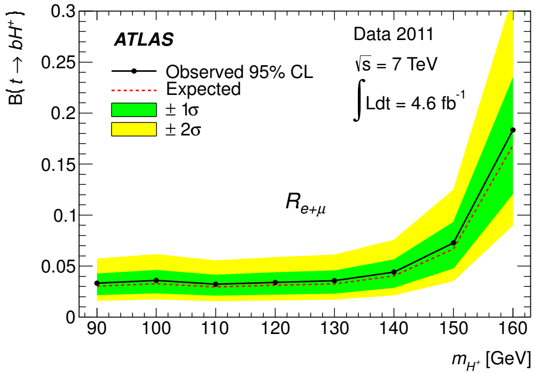
Figure 6.10. Expected and observed 95% confidence level upper limits on \mathcal{B}(t \rightarrow bH^+) for H^+ masses between 90 and 160 GeV and assuming \mathcal{B}(H^+ \rightarrow \tau\nu) = 100\% , using the event yield ratio R_{e+\mu} .
