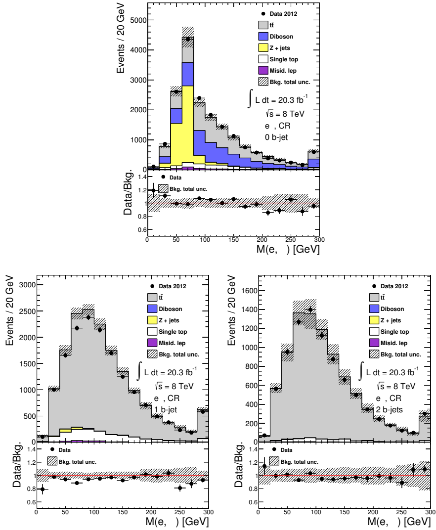
Figure 7.4. The e\mu invariant mass in dilepton events passing the CR selection with 0 b -tagged jets (top), 1 b -tagged jet (bottom left) or 2 b -tagged jets (bottom right). In all plots, the last bin includes overflow.
