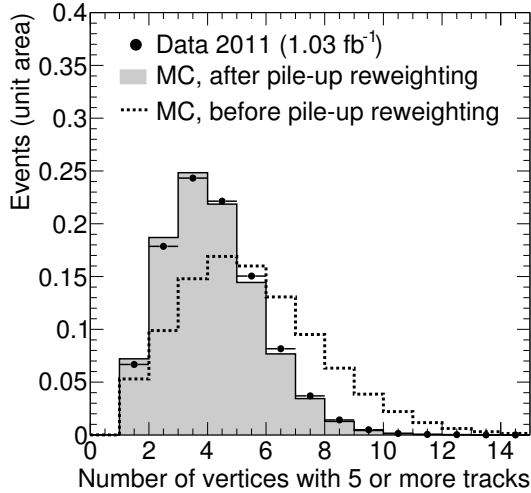
Figure 5.1. Example of pile-up reweighting of a t\bar{t} Monte Carlo (MC) sample to match the distribution of the average number of simultaneous pp collisions in data. The reweighting is validated by comparing the normalized distributions of the number of reconstructed vertices.
