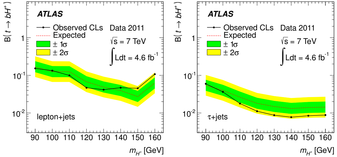
Figure 6.12. 95% confidence level upper limits on \mathcal{B}(t \rightarrow bH^+) , with the assumption that \mathcal{B}(H^+ \rightarrow \tau\nu) = 100\% , as obtained in the lepton + jets channel (left) and in the \tau_{\text{had}} + \text{jets} channel (right) [97].
