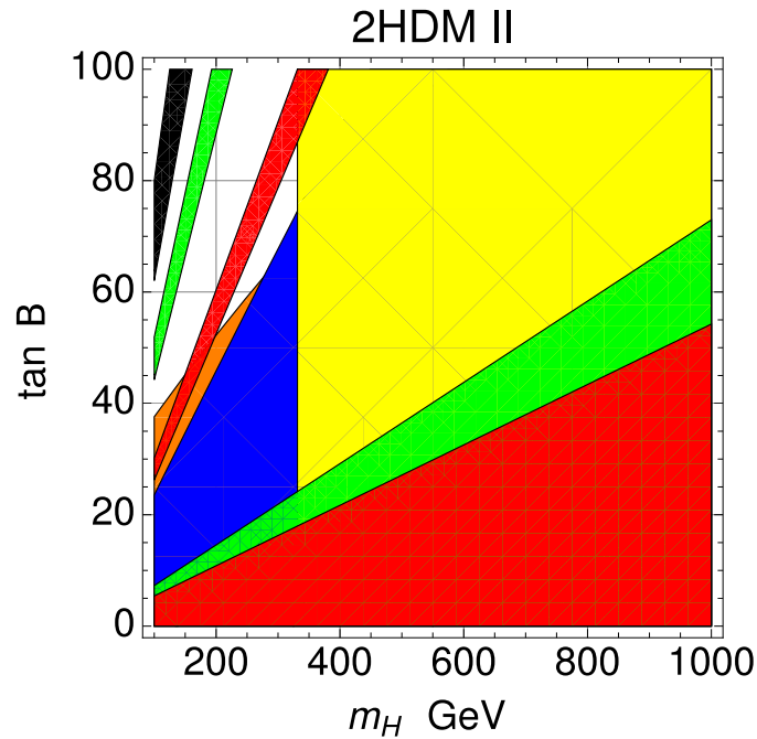
Figure 2.8. Allowed regions (superimposed) in the \tan\beta , m_H = m_A = m_{H^\pm} parameter space of the Type II 2HDM, using constraints from b \rightarrow s\gamma (yellow), B \rightarrow D\tau\nu (green), B \rightarrow \tau\nu (red), B_s \rightarrow \mu^+\mu^- (orange), K \rightarrow \mu\nu/\pi \rightarrow \mu\nu (blue) and B \rightarrow D^*\tau\nu (black). The regions shown include theoretical uncertainties added linearly to the 2\sigma experimental errors [33].
