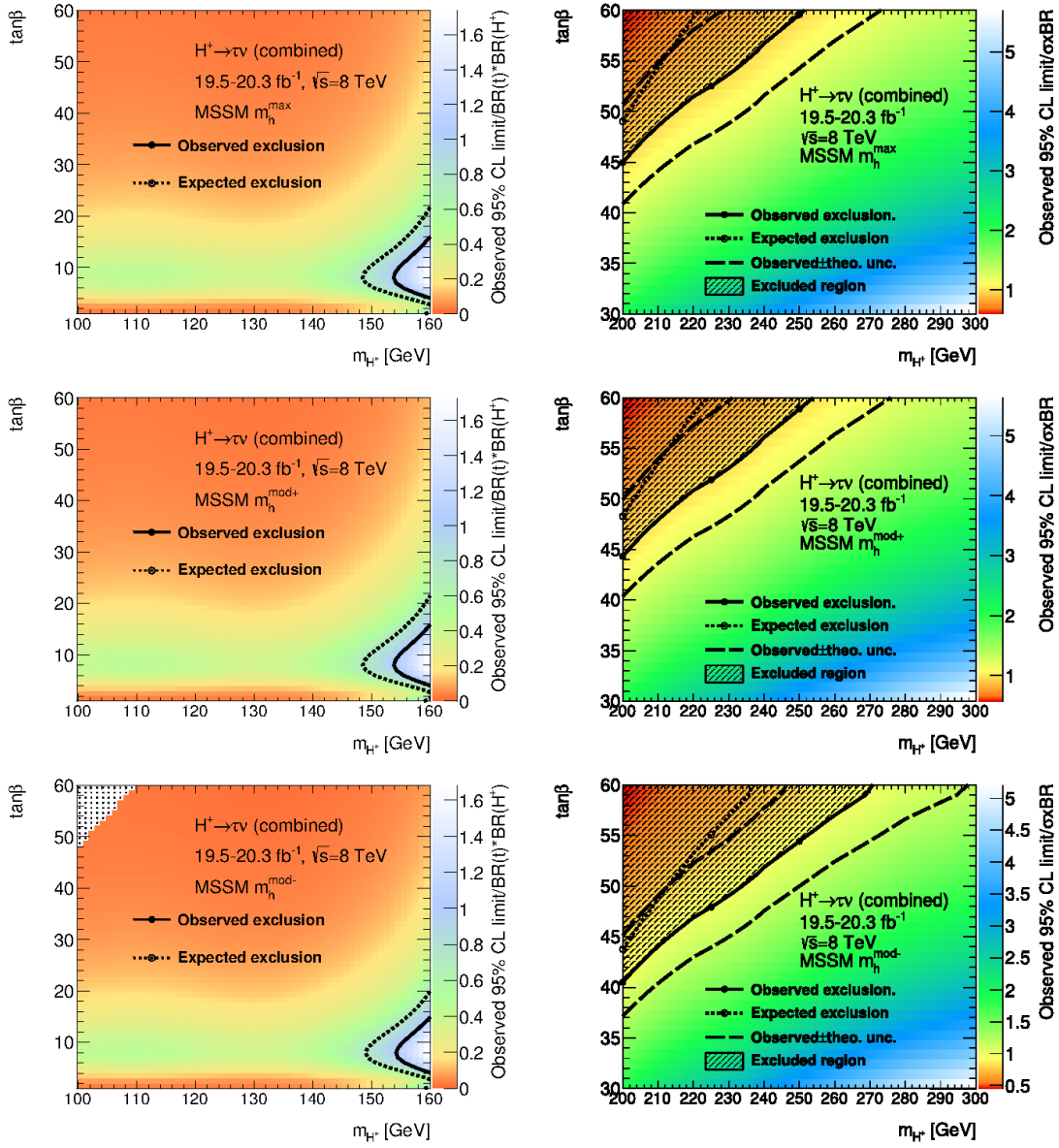
Figure 7.12. Expected and observed 95% confidence level exclusion limits in the \tan\beta , m_{H^+} plane for low (left) and high (right) mass ranges in the updated m_h^{\max} (top), m_h^{\text{mod}+} (middle), and m_h^{\text{mod}-} (bottom) MSSM scenarios, obtained by combining the lepton + \tau_{\text{had}} and \tau_{\text{had}} + jets channels. The colors indicate the ratio of the achieved exclusion limit to the predicted signal strength (cross section and/or branching fraction). A large value means that large improvements of the search sensitivity would be needed to exclude that point in the parameter space. Theoretical predictions above \tan\beta = 60 are not available.
