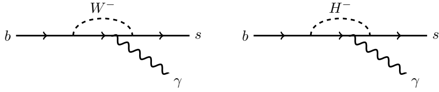
Figure 2.6. Examples of contributions to the b \rightarrow s\gamma decay from a W boson (left) and a charged Higgs boson (right).
