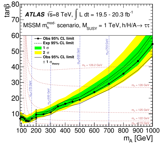
Figure 3.4. 95% confidence level exclusion limits in the \tan\beta, m_A parameter space from a search for neutral Higgs bosons decaying to \tau\tau in ATLAS [45]. Results are shown in the m_h^{\max} (top), m_h^{\text{mod}+} (middle), and m_h^{\text{mod}-} (bottom) scenarios.
