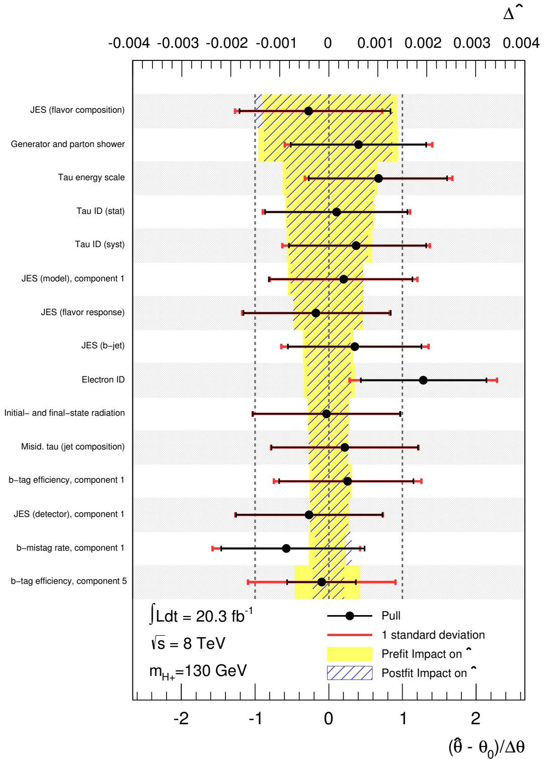
Figure 7.7. Pull distribution for the m_{H^+} = 130 \text{ GeV} hypothesis. The black markers indicate the shift of the best-fit value of each parameter with respect to its nominal value in units of one standard deviation (red) as indicated on the bottom axis, while the yellow and hatched blue bands respectively show the pre- and post-fit impacts on the fitted signal strength as indicated on the top axis. The 15 most important parameters are shown. Some of the uncertainties related to the jet energy scale (JES) or b -tagging are split into several effective components.
