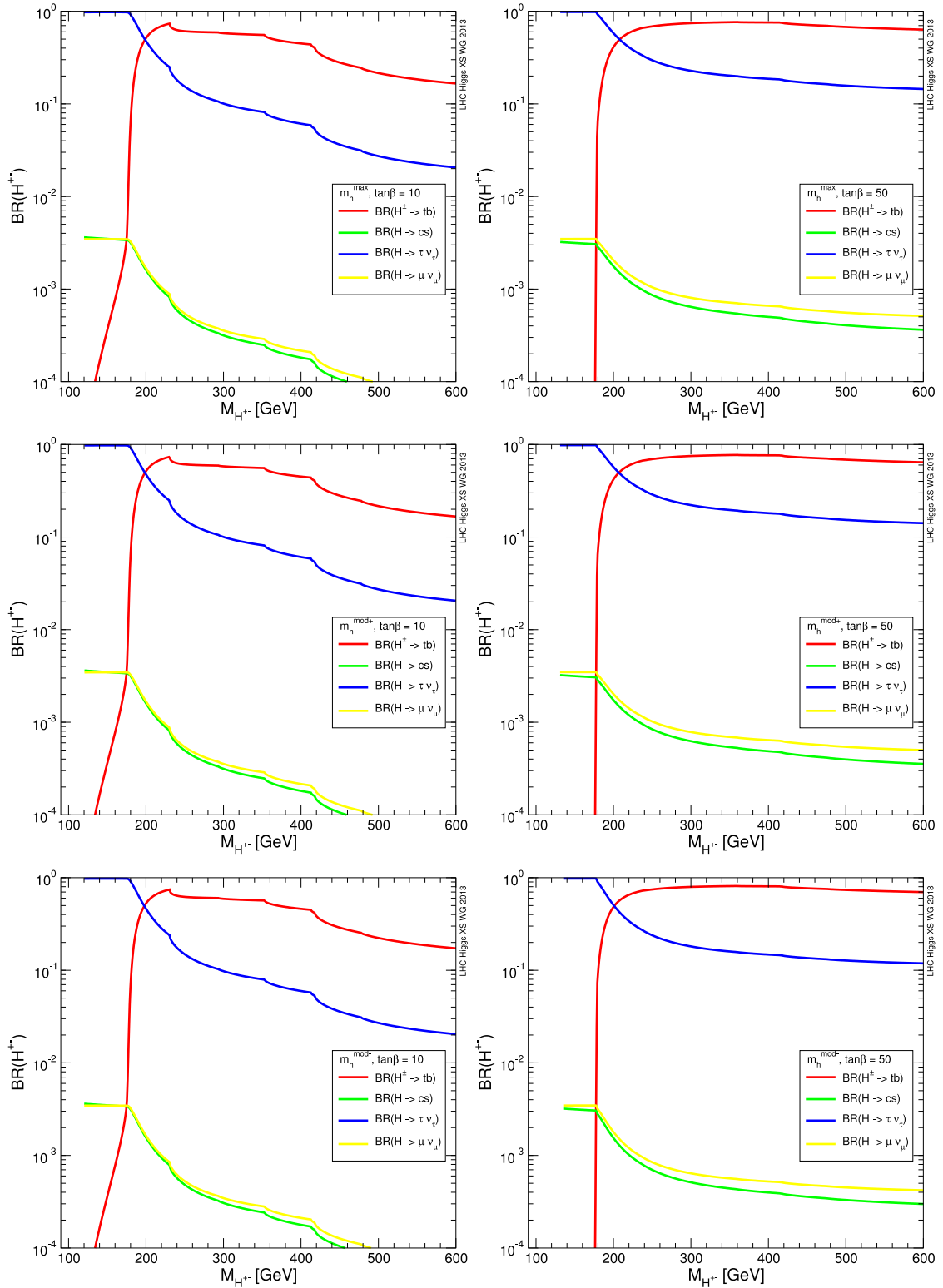
Figure 2.1. Branching fractions of the charged Higgs boson in the MSSM m_h^{\max} (top row), m_h^{\text{mod}+} (middle row), and m_h^{\text{mod}-} (bottom row) scenarios with \tan\beta = 10 (left column) and \tan\beta = 50 (right column) [21].
