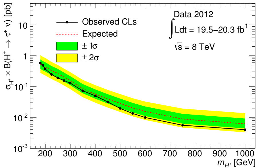
Figure 7.11. Expected and observed 95% confidence level upper limits on charged Higgs boson production in the low (top) and high (bottom) mass range, obtained with a combination of the lepton + \tau_{\text{had}} and \tau_{\text{had}} + jets channels.
