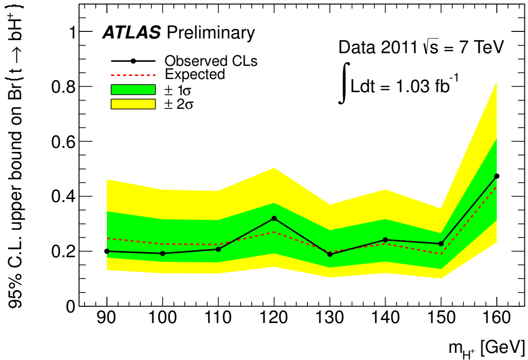
Figure 6.3. 95% confidence level upper limits on \mathcal{B}(t \rightarrow bH^+) as a function of the charged Higgs boson mass, obtained in the dilepton analysis. The solid black line indicates the observed limit, while the dashed line indicates the expected limit with the background-only hypothesis. The green and yellow shaded regions indicate the 1\sigma and 2\sigma error bands, respectively.
