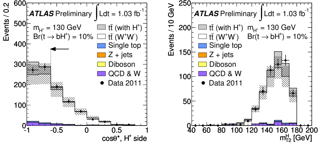
Figure 6.2. The left-hand side plot shows the \cos \theta_\ell^* distribution of the dilepton events. The arrow indicates the signal region \cos \theta_\ell^* < -0.6 and the right-hand side plot shows the m_{T2}^H distribution of the events found in this region. The striped area indicates the systematic uncertainties on the backgrounds and the grey histogram shows the contribution of events with a 130 GeV charged Higgs boson with \mathcal{B}(t \rightarrow bH^+) = 10\% . A fitted value of 150.4 pb is used for \sigma_{bbWW} .
