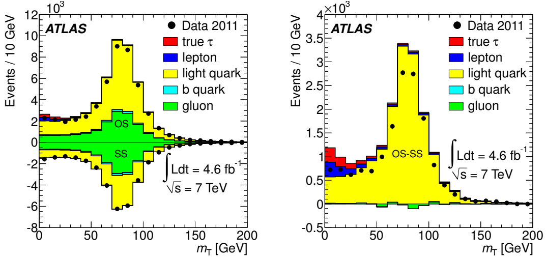
Figure 6.6. Distributions of m_T after applying the W + > 2\text{jets} event selection (the requirement m_T > 30 GeV is not applied in these plots). The colors correspond to the type of highest-energy generator-level particle found within a cone of radius R = 0.2 around the \tau_{\text{had}} candidate. The left-hand side plot shows OS and SS events with positive respectively negative weights, while the right-hand side plot shows the result of subtracting the SS events from the OS events.
