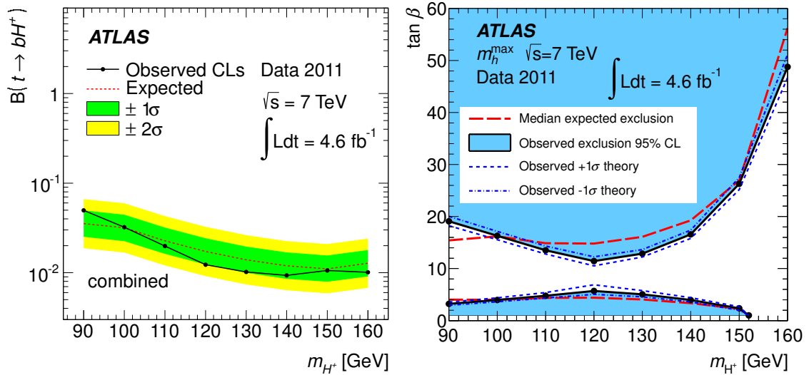
Figure 6.13. 95% confidence level upper limits on \mathcal{B}(t \rightarrow bH^+) , with the assumption that \mathcal{B}(H^+ \rightarrow \tau\nu) = 100\% , obtained by combining the lepton + jets, \tau_{\text{had}} + \text{jets} (both from Ref. [97]), and lepton + \tau_{\text{had}} channels (left), and their interpretation in the MSSM m_h^{\text{max}} scenario (right).
