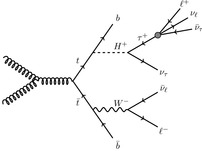
Figure 6.1. Feynman diagram of a t\bar{t} event involving a charged Higgs boson, with two charged leptons \ell = e, \mu in the final state.
