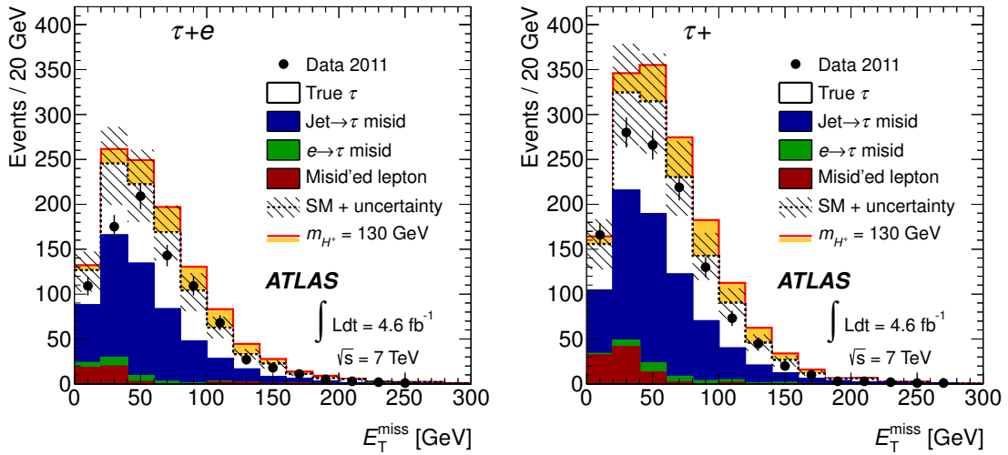
Figure 6.4. E_T^{\text{miss}} distribution in e + \tau_{\text{had}} (left) and \mu + \tau_{\text{had}} events (right). The individual contributions of both the signal and the t\bar{t} background are scaled to match the prediction in the presence of a 130 GeV charged Higgs boson with \mathcal{B}(t \rightarrow bH^+) = 5\% and \mathcal{B}(H^+ \rightarrow \tau\nu) = 100\% . The Standard Model prediction is shown as a dashed line, with the hatched area indicating its total uncertainty.
