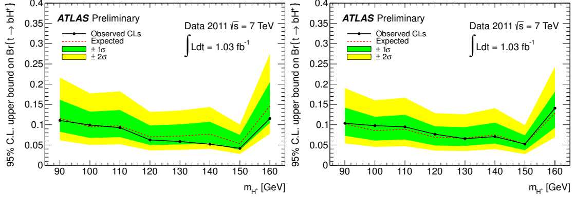
Figure 6.11. 95% confidence level upper limits on \mathcal{B}(t \rightarrow bH^+) , with the assumption that \mathcal{B}(H^+ \rightarrow \tau\nu) = 100\% , as obtained in the lepton + jets channel [93] (left) and with a combination of the lepton + jets and dilepton channels (right) using early 2011 data.
