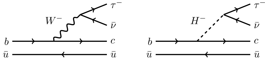
Figure 2.7. B \rightarrow D^{(*)}\tau\nu decay, mediated by a W boson (left) or a charged Higgs boson (right).
