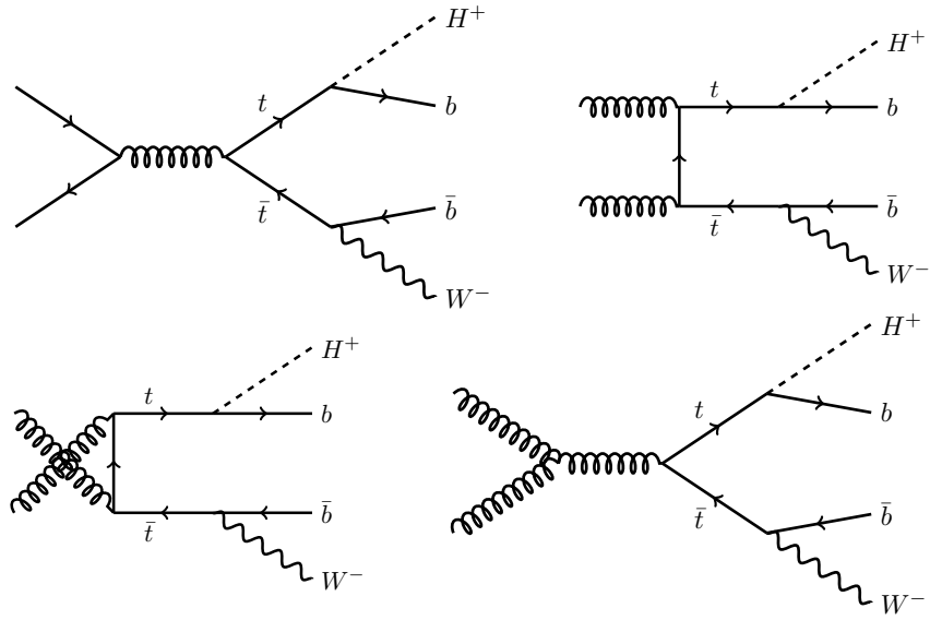
Figure 2.2. Light charged Higgs boson production in the decay of top quarks. Top quark pair production proceeds mainly via q\bar{q} fusion at the Tevatron and gluon-gluon fusion at the LHC.
