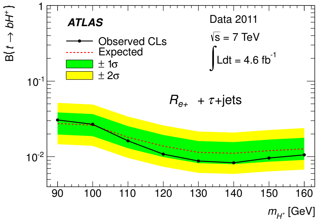
Figure 6.14. 95% confidence level upper limits on \mathcal{B}(t \rightarrow bH^+) , with the assumption that \mathcal{B}(H^+ \rightarrow \tau\nu) = 100\% , obtained with a combination of the direct search in the \tau_{\text{had}} + \text{jets} channel and the event yield ratio R_{e+\mu} .
