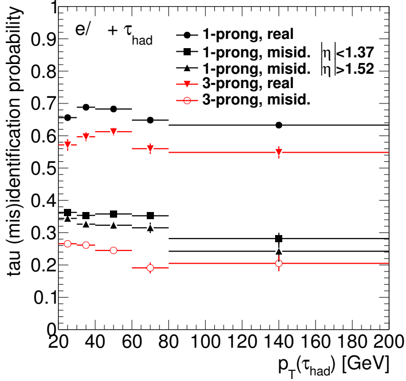
Figure 7.2. The \tau_{\text{had}} (mis)identification probabilities used in the matrix method.
