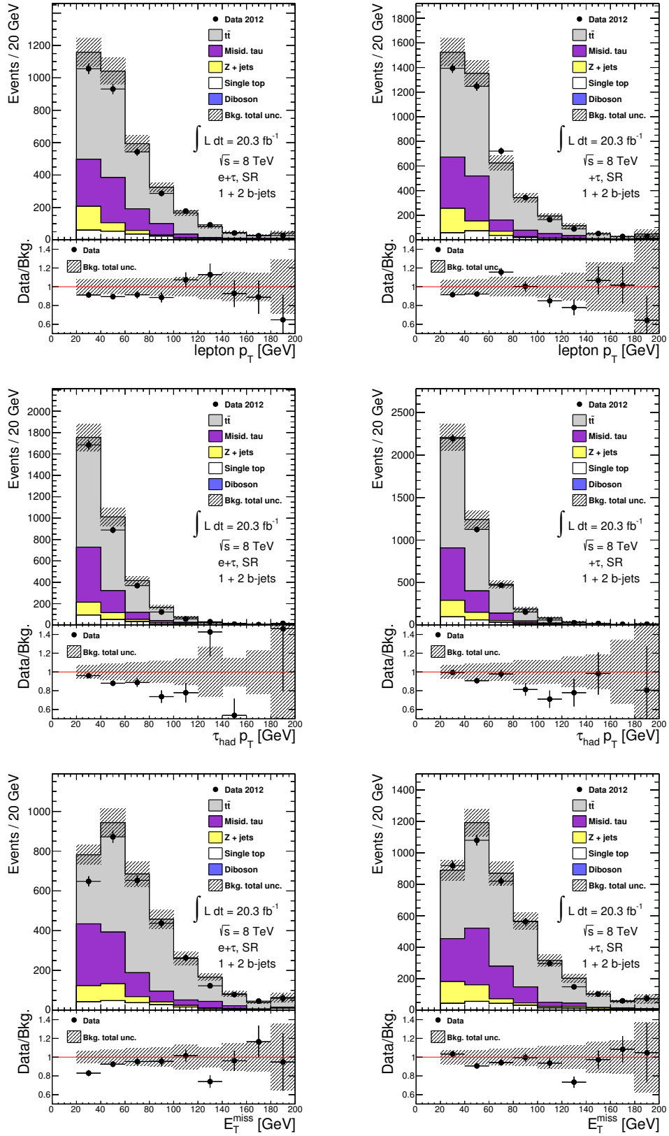
Figure 7.3. The lepton p_T (top), the p_T of the \tau_{\text{had}} object (middle), and the E_T^{\text{miss}} (bottom) in e + \tau_{\text{had}} (left) and \mu + \tau_{\text{had}} (right) events passing the SR selection. In all plots, the last bin includes overflow.
