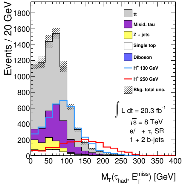
Figure 7.1. Comparison of the m_T distribution for the Standard Model backgrounds (stacked histograms) and two signal samples with charged Higgs boson masses of 130 GeV and 250 GeV in the lepton + \tau_{\text{had}} channel. The normalization of the two signal samples correspond to \mathcal{B}(t \rightarrow bH^+) = 10\% or a production cross section of 10 pb, respectively.
