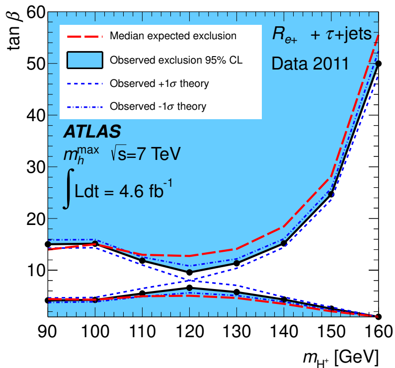
Figure 6.15. 95% confidence level exclusion limits in the parameter space of the MSSM m_h^{\text{max}} scenario, as obtained from the combination of the \tau_{\text{had}} + \text{jets} channel and the event yield ratio R_{e+\mu} .
