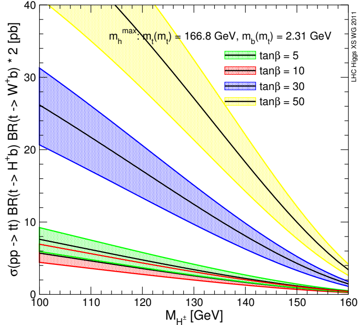
Figure 2.3. Cross section for the process pp \rightarrow t\bar{t} \rightarrow b\bar{b}W^\mp H^\pm at 7 TeV in the m_h^{\max} scenario, including scale and PDF uncertainties, as well as uncertainties due to missing electroweak, QCD, and SUSY corrections [25]. Note that both H^+ and H^- production is taken into account.
