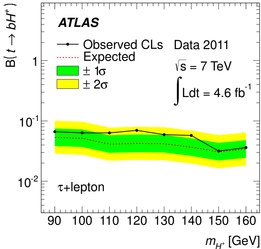
Figure 6.5. Expected and observed 95% confidence level exclusion limits on the branching fraction \mathcal{B}(t \rightarrow bH^+) for a range of charged Higgs boson masses between 90 and 160 GeV, and with the assumption \mathcal{B}(H^+ \rightarrow \tau\nu) = 100\% , as obtained in the analysis of lepton + \tau_{\text{had}} events in 7 TeV data.
