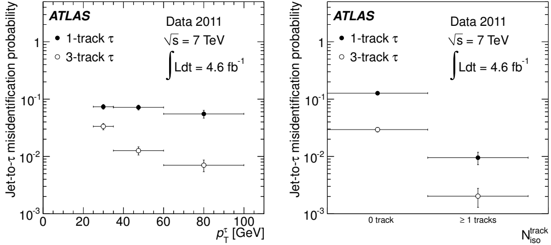
Figure 6.7. Probabilities for a jet initiated by a light quark to be misidentified as a \tau_{\text{had}} with one or three tracks, measured in OS-SS events in data using the W + > 2 jets event selection, as a function of p_T (left) and of the number of tracks N_{\text{iso}}^{\text{track}} in the isolation cone (right).
