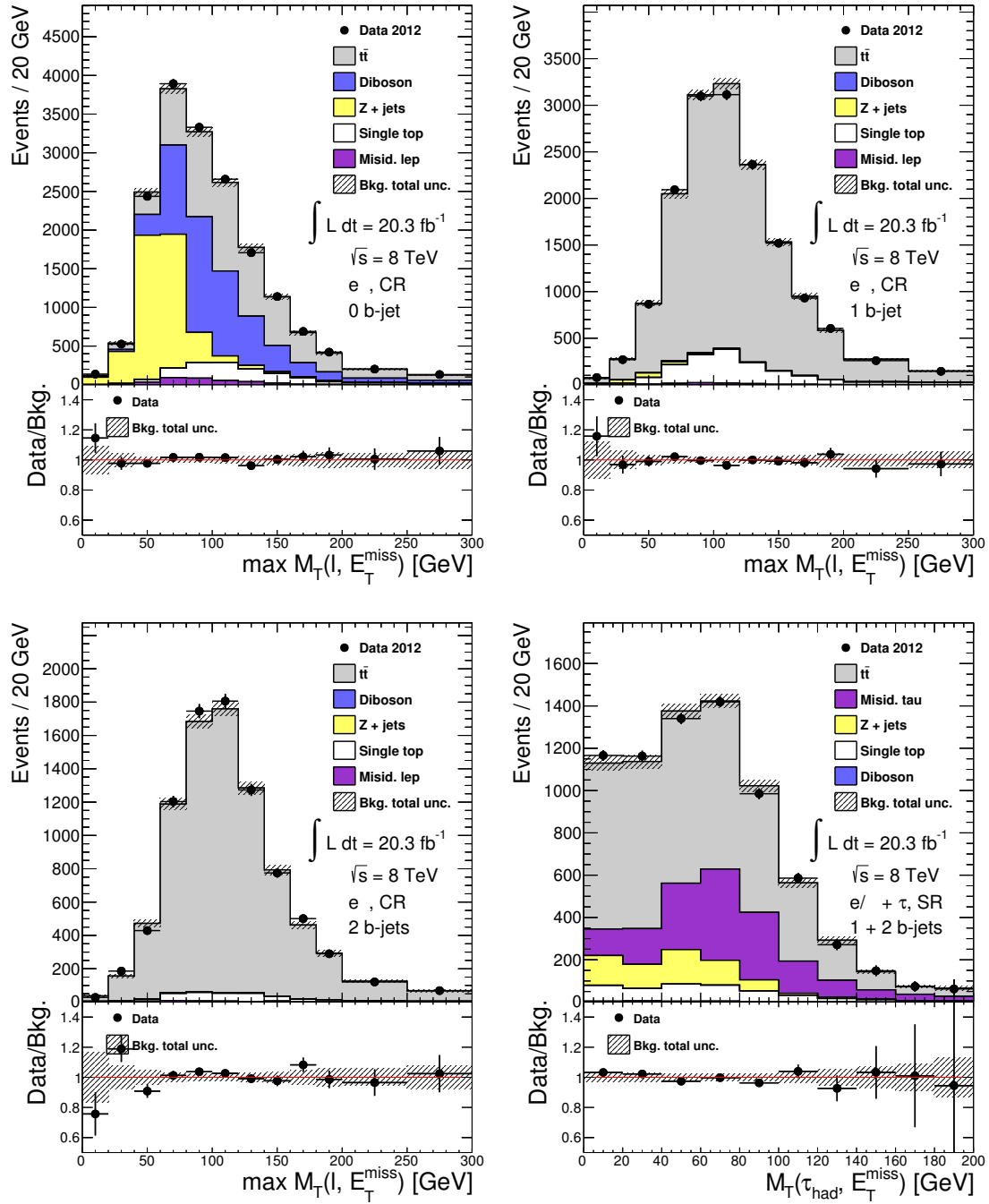
Figure 7.6. Post-fit plots of the maximum transverse mass of dilepton events passing the CR selection with 0 b -tagged jets (top left), 1 b -tagged jet (top right), and 2 b -tagged jets (bottom left), as well as the transverse mass of lepton + \tau_{\text{had}} events passing the SR selection with one or two b -tagged jets. In these plots, the best-fit values of all nuisance parameters under the background-only hypothesis, and their uncertainties, are shown. The last bin includes overflow.
