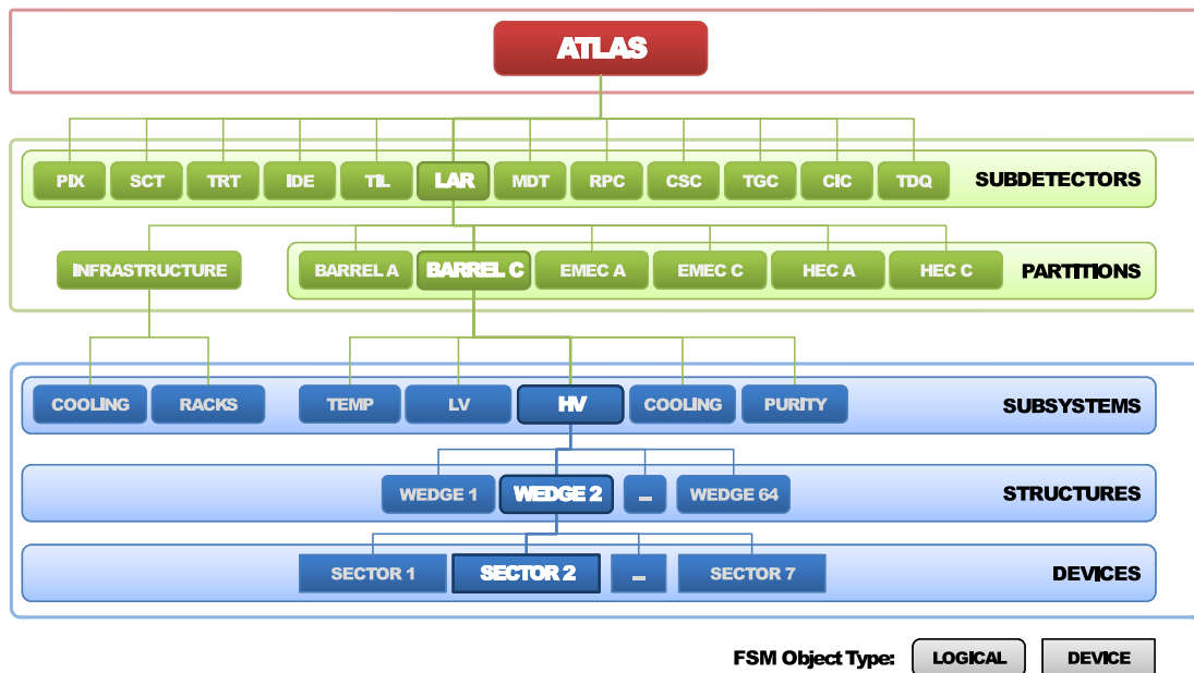
Figure 4.5. The ATLAS DCS architecture (top) and parts of its logical representation as a Finite State Machine (bottom). This figure is reprinted from Ref. [56].
