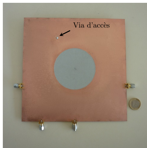
FIGURE 2.72 – Composant compressif 2D.
