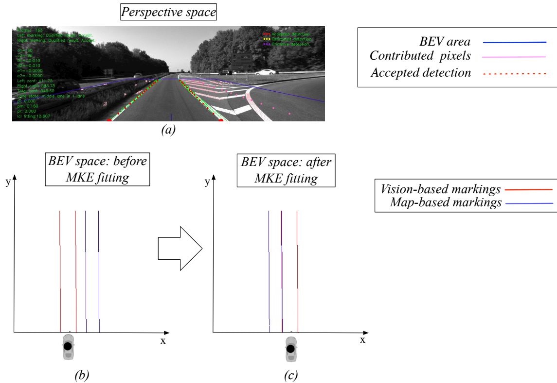
Figure 4.5: Example of localization error. (a) Lane detection in perspective space; (b) the markings before MKE fitting; (c) the markings after MKE fitting.
