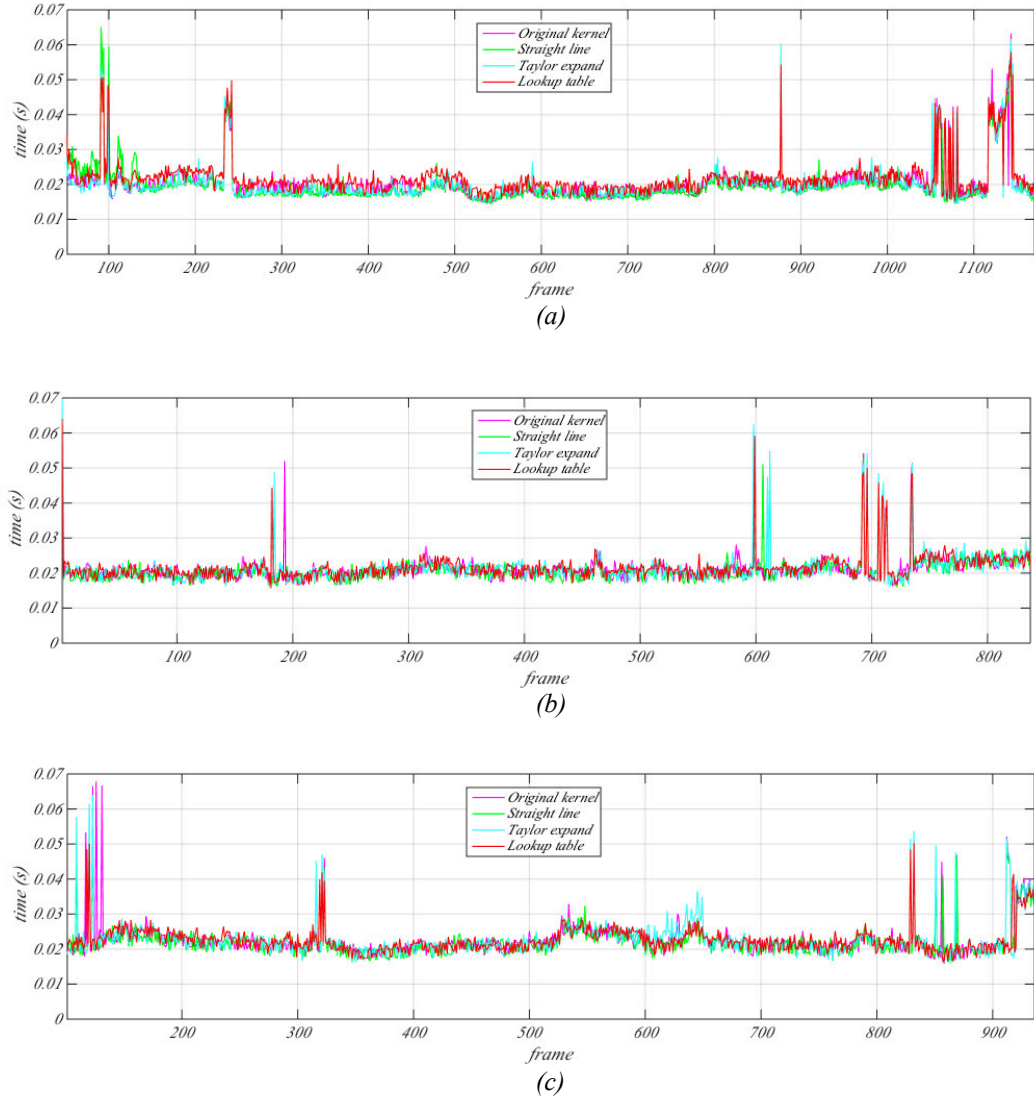
Figure 2.20: Run time of four MKE methods in different KITTI scenarios. (a)-(c) are the algorithm run time of different kernels on different KITTI scenarios.
