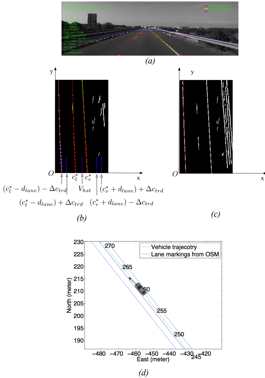
Figure 4.7: Example of normal detection in map topology error modeling. (a) Lane detection in perspective space; (b) detected the markings of the host lane and the third marking in BEV space; (c) the third lane marking and lane marking “signatures”; (d) vehicle position in ENU space. Red curves are the markings of the host lane, while pink lines are the third lane markings.
