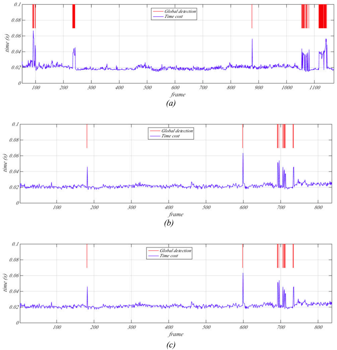
Figure 2.17: Time cost of lane detection algorithm. (a)-(c) represent three different scenarios of KITTI database. Blue curves are time cost, red curves are lane tracking/detecting state.
