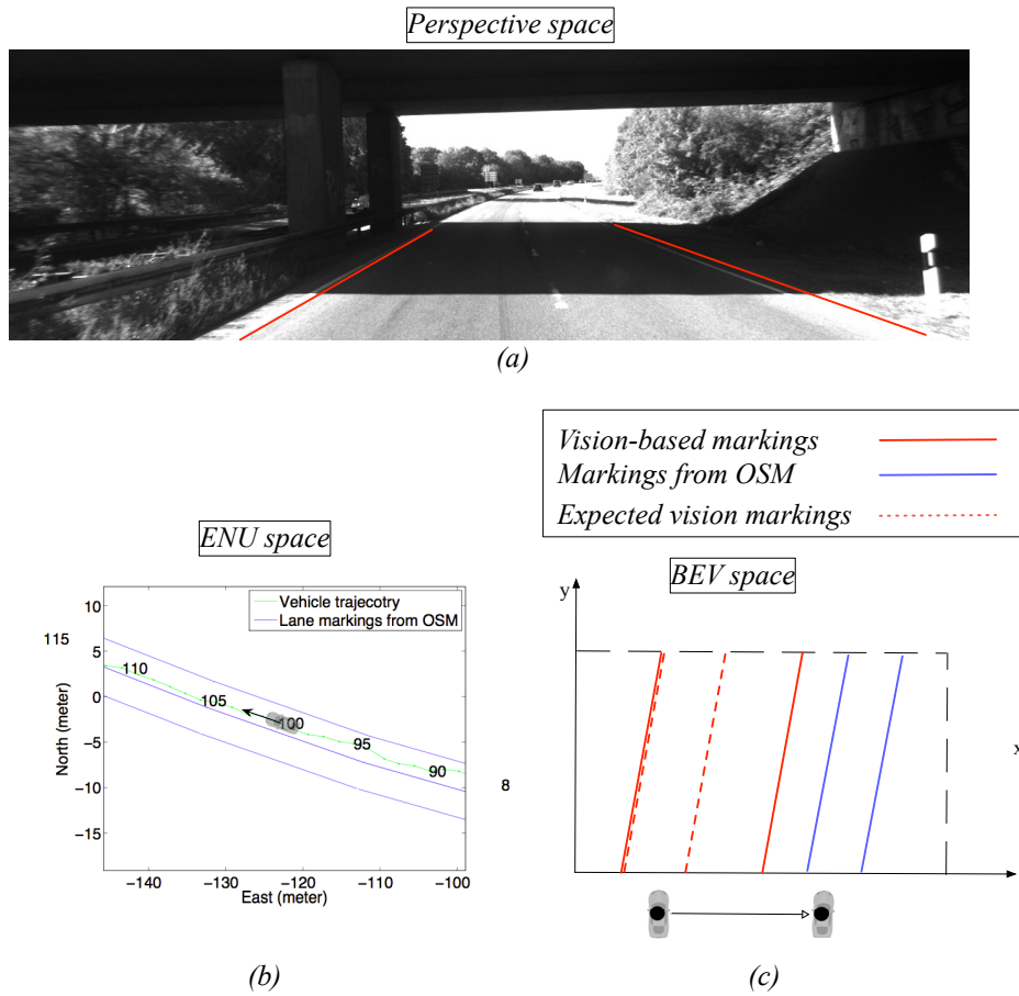
Figure 4.1: Example of lane detection error. (a) Lane detection in perspective space; (b) vehicle position in ENU space; (c) Lane markings from vision detection and OSM in BEV space.
