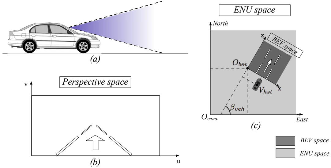
Figure A.1: Camera implementation and coordinates definition. (a) Camera setup; (b) perspective image from camera; (c) ENU space \mathbb{R}^2 (light gray) and BEV space \mathbb{B}^2 (dark gray).
