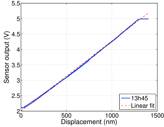
Fig. F.2. FT-S540 (S-2501) force sensor characterization.
