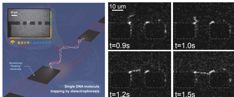
Fig. 4.1. Isolation and trapping of long single DNA molecules using high electric field between integrated electrodes in a microfluidic environment. The video frames detail the process of DNA trapping [Kumemura 2007].
