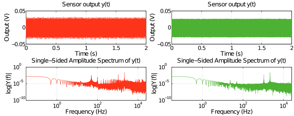
Fig. 3.29. Frequency characterizations of the noise of the tweezers sensor output, in regular room conditions (left) and in a grounded box (right). Tweezers are stimulated with sinusoidal signal at its resonance frequency. Uppers graphs shows sensor outputs while below are represented frequency analysis of the output signals. (Tweezers RV12).
