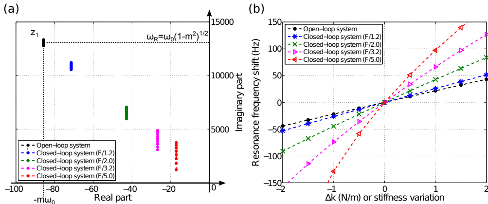
Fig. 5.3. (a) Root locus of the tweezers driven in open loop and in closed-loop. One complex conjugate pole z_1 of the 2nd order equivalent tweezers model is plotted in the s -plan. Equivalent system performances, resonance frequency \omega_r and damping m , are shown. Poles of the systems move with the variation of the parameter k . \Delta k varies from -2 to 2 N/m by 0.5 N/m step. (b) Subsequent evolution of the resonant frequency shift f_r of the open loop system (OLS) and of the different closed-loop systems (CLSs) vs. variations of k . In black, the evolution of the resonant frequency of the OLS. In blue, the evolution of the resonant frequency of the CLS resonating at a frequency 1.2 times lower than the device resonating frequency ( \beta = 1.2 ). In green, with the CLS resonating at a frequency 2 times lower ( \beta = 2 ). In pink, with the CLS resonating at a frequency 3.2 times lower ( \beta = 3.2 ). And in red, with the CLS resonating at a frequency 5 times lower ( \beta = 5 ).
