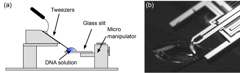
Fig. 4.2. Experimental setup of the DNA trapping. (a) Schematic of the setup. Tweezers are brought at the surface of a DNA solution droplet. (b) Photograph of the tweezers tips at the surface of DNA solution droplet for DNA molecule trapping.
