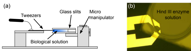
Fig. 4.13. Experimental setup of the bioreaction experiment with HindIII enzymes. (a) Schematic of the setup (side view). Tweezers are immersed inside a slit made of glass slits and containing the enzyme solution. (b) Microscopy photograph of the tweezers tips inside the experimental slit and inside the enzyme solution.
