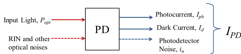
Fig. 3.33. Generation of noise from the photodetector
