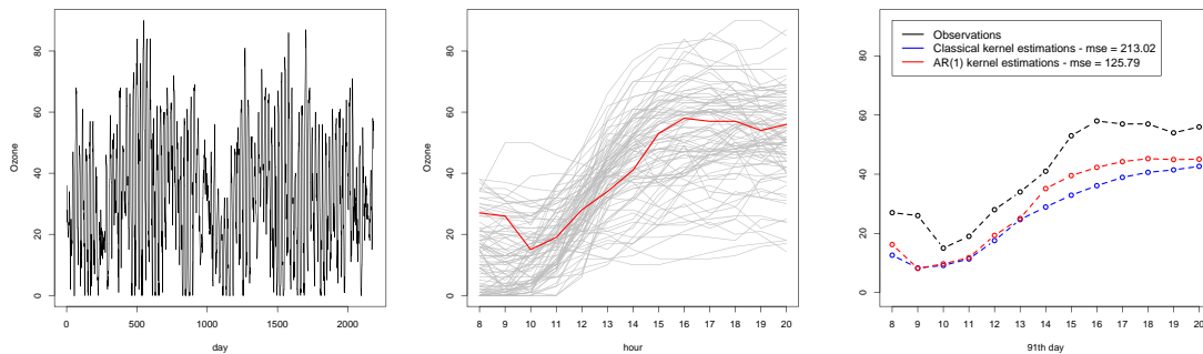
Figure 5.7 – Ozone concentrations at Station 93 Left: entire series. Middle: considered curves. Right: predictions.
