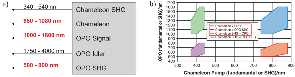
Figure 2.2: Specifications of the femtosecond system. (a) Independent wavelength tuning of laser+OPO with multiple outputs operating at different spectral range. Outputs used in our studies are marked in red. (b) Possible wavelength combinations.
