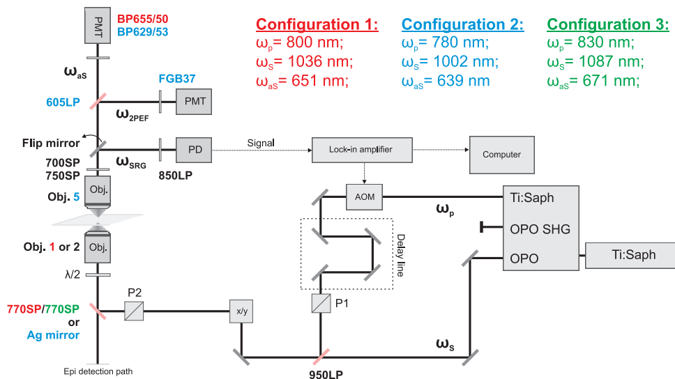
Figure B.2: The experimental configurations 1, 2 and 3 of the femtosecond set-up. The sample is illuminated by the the pump and the Stokes beams in one of the three configurations. The spectrally filtered CARS ( \omega_{aS} ) and 2PEF ( \omega_{2PEF} ) signals are collected either in the forward direction using PMTs or in the backward direction shown in the Fig. B.4. The spectrally filtered SRS ( \omega_{SRG} ) signal is collected in the forward direction using PD detector. Optical elements used specifically in the configuration 1 are color coded in red, in the configuration 2 in blue and in configuration 3 in green. Black color corresponds to elements used in all configurations. The epi-detection path for this configuration is shown in Fig. B.4.
