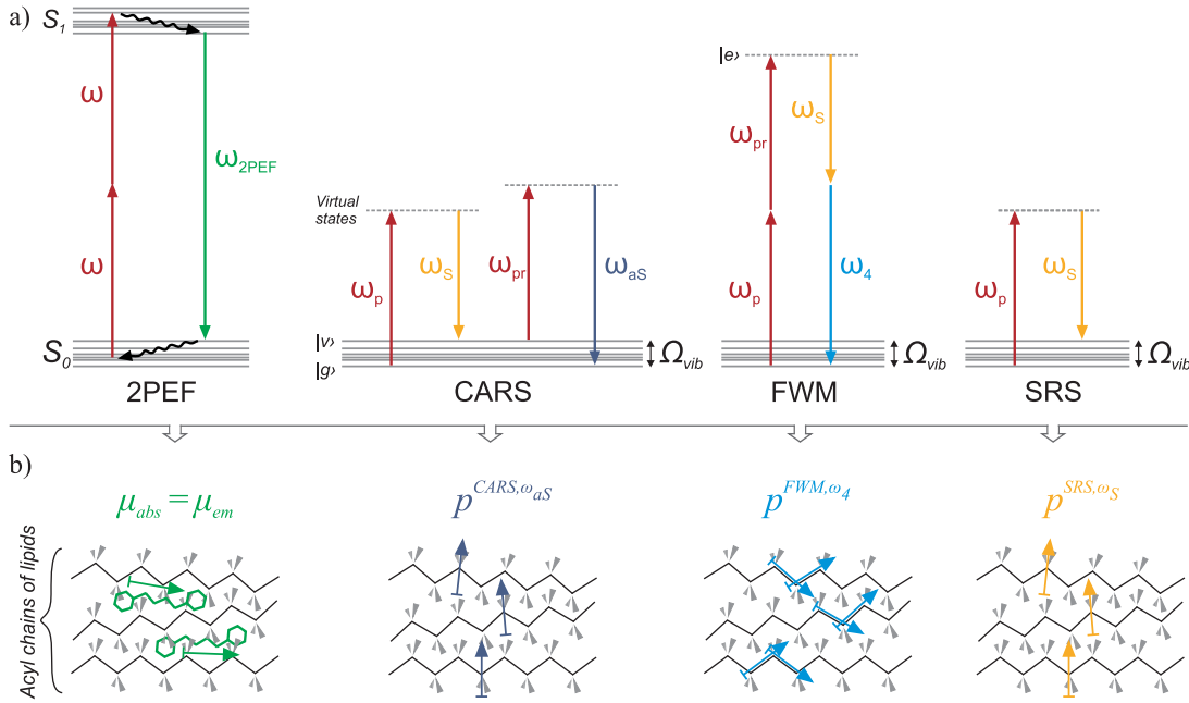
Figure 1.1: (a) Energy diagram schemes of the different contrasts used in these studies. (b) The radiation from a molecule either originates from the emission transition dipoles \mu_{em} (2PEF) or the third order nonlinear dipoles p^{SRS, CARS, FWM} (SRS, CARS, FWM) induced by the excitation fields involved in the contrast used. The colored arrows exhibit the directions of the induced dipoles involved in the nonlinear processes, which define the probed molecular organization directions.
