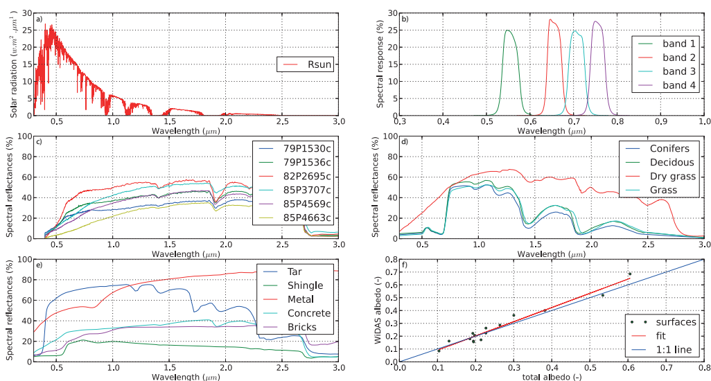
Figure 5.1: Illustration of the computation of the "camera albedo" and global albedo for each type of surface. (a) Incoming solar radiation. (b) WiDAS filter functions. Spectral signatures for soil (c), vegetation (d) and for artificial materials (e). (f) Scatter plot proving relationship to retrieve global albedo from discrete values (WiDAS).
