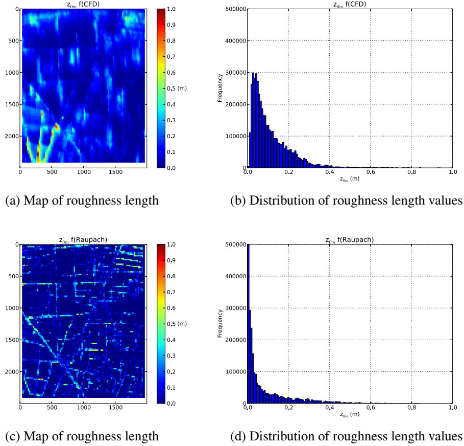
Figure 5.5: Roughness length for momentum transfer values over the Yingke Oasis station retrieved from CFD and Raupach's model.
