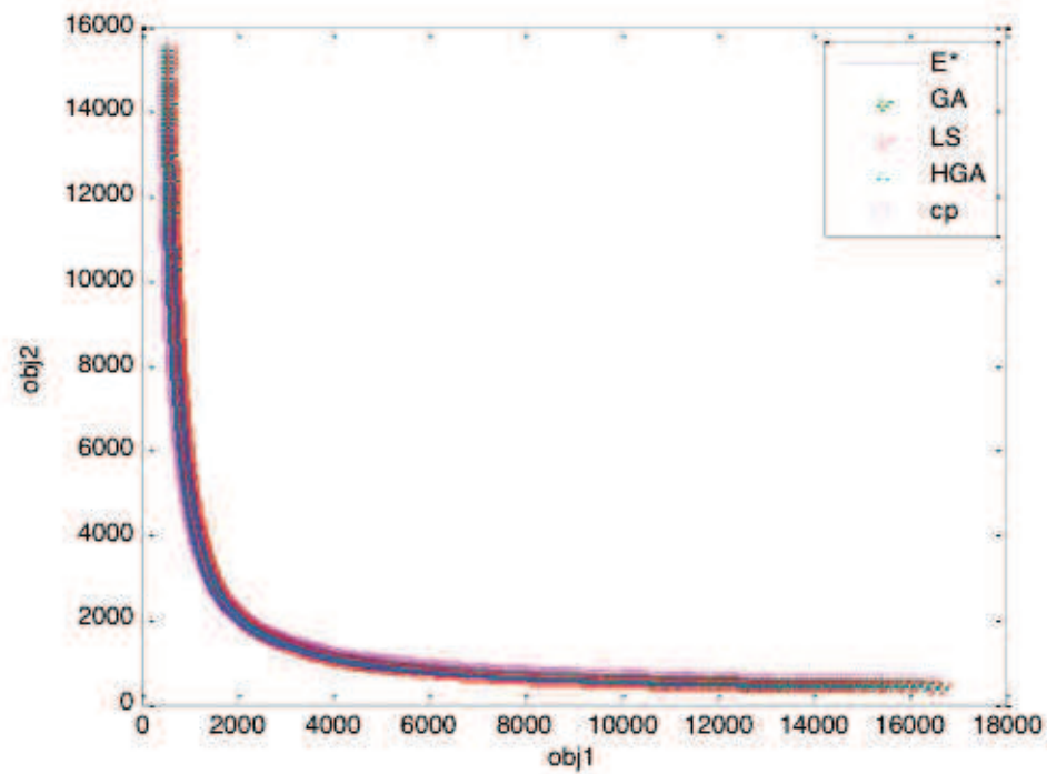
Figure 4.6: Pareto fronts of 2AP500-1A100
