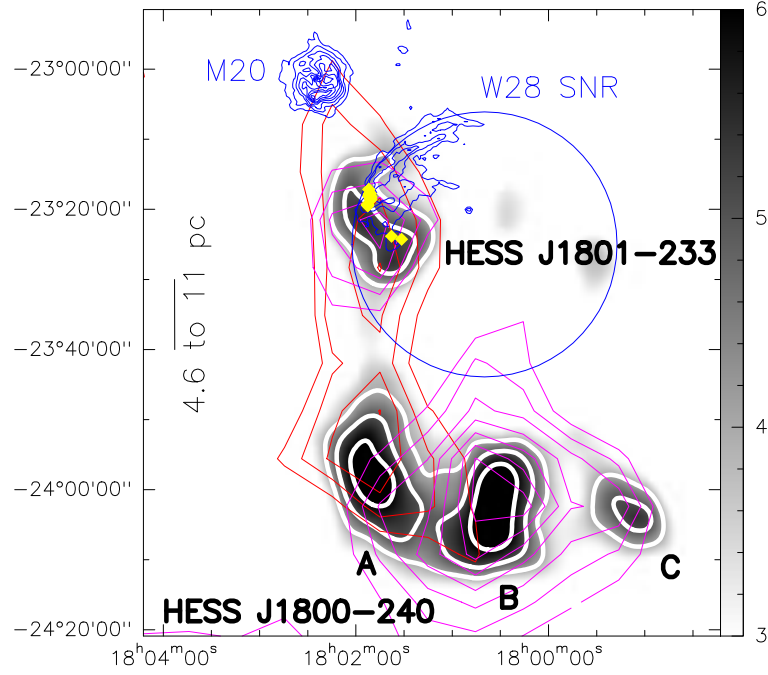
Figure 4.4: Large scale map of the W28 complex: evidence of the interaction (Vaupré et al., 2014). The blue circle gives the approximate radio boundary of the SNR W28 (Brogan et al., 2006). A large molecular cloud next to the remnant is shown by CO(1-0) emission (Dame et al., 2001): red contours show the emission integrated over 15 - 25 \text{ km s}^{-1} and magenta contours trace the emission integrated over 5 - 15 \text{ km s}^{-1} (levels are 40 - 70 \text{ K km s}^{-1} by 5 \text{ K km s}^{-1} ). Extended TeV emission from the cloud is suggestive evidence of the interaction of the SNR with the cloud through proton-proton collisions and pion-decay. TeV emission as seen by HESS is shown by the grayscale (in \sigma ) and thick white contours (levels are 4 - 6 \sigma ). Further evidence of the interaction can be found e.g. in the presence of OH masers (Claussen et al., 1997), shown by yellow diamonds, which are a signature of shocked gas.
