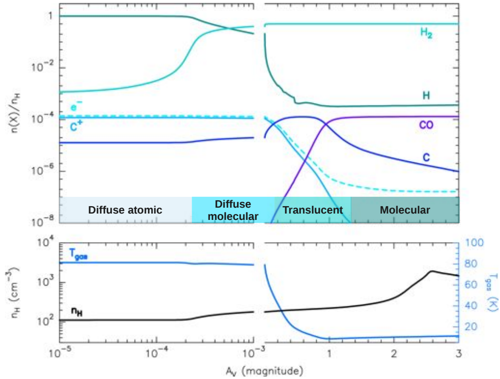
Figure 1.2: Top: Classification of clouds w.r.t. the visual extinction, based on the dominant reservoirs of C and H, following Snow and McCall (2006). Bottom: Corresponding density and temperature profiles. The visual extinction is computed from N_{\text{H}} \sim 1.87 \times 10^{21} \text{ cm}^{-2} \text{ mag}^{-1} \times A_V (Bohlin et al., 1978).
