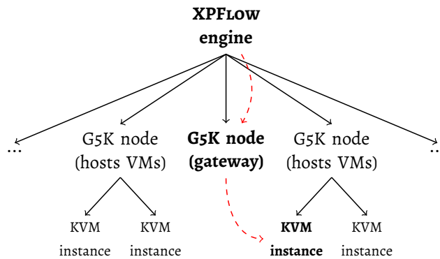
Figure 20: Hierarchical structure of nodes used in the cloud-like testbed. Three nested levels can be distinguished (XPFLow engine, Grid'5000 nodes, KVM instances). The red, dashed path describes a connection used to access and control virtual machines.
