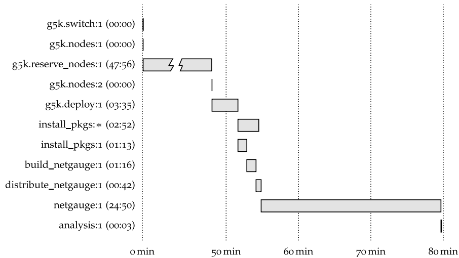
Figure 11: Gantt chart of an experiment (edited for readability). Various activities are executed, some of them in parallel: install_pkgs:* represents multiple parallel activities install_pkgs that execute on the nodes of the experiment (by means of forall experimental pattern).
