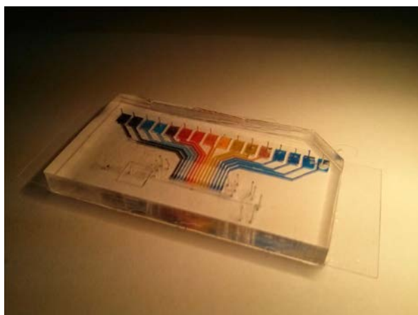
Figure 7.8 – Multiplexed platform for the in situ encoding of droplets with DNA barcodes
